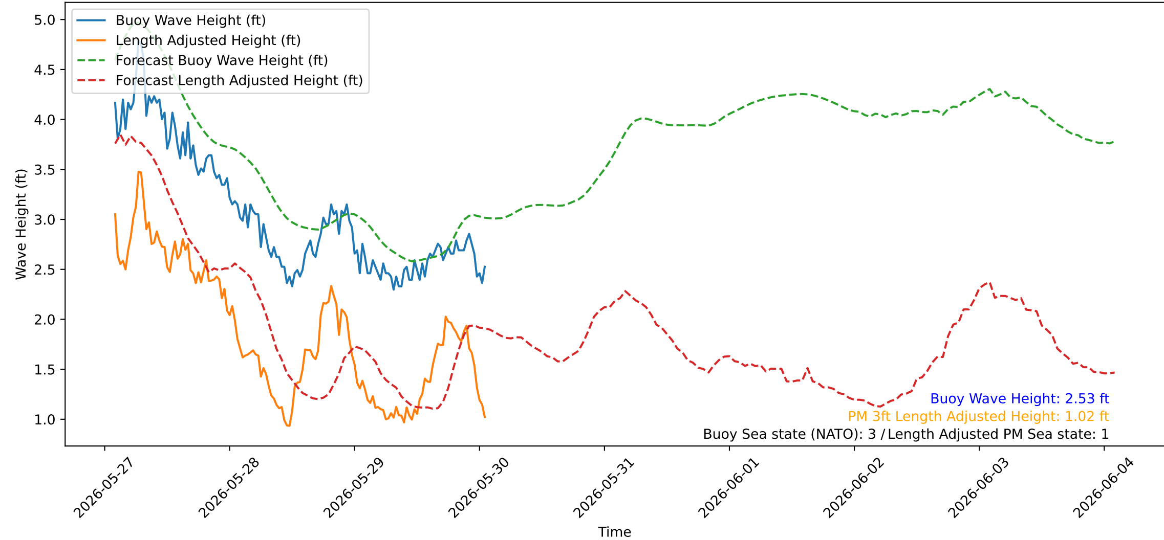
Wave Heights over Time for Red Beach at 2026-05-30 01:50:43
