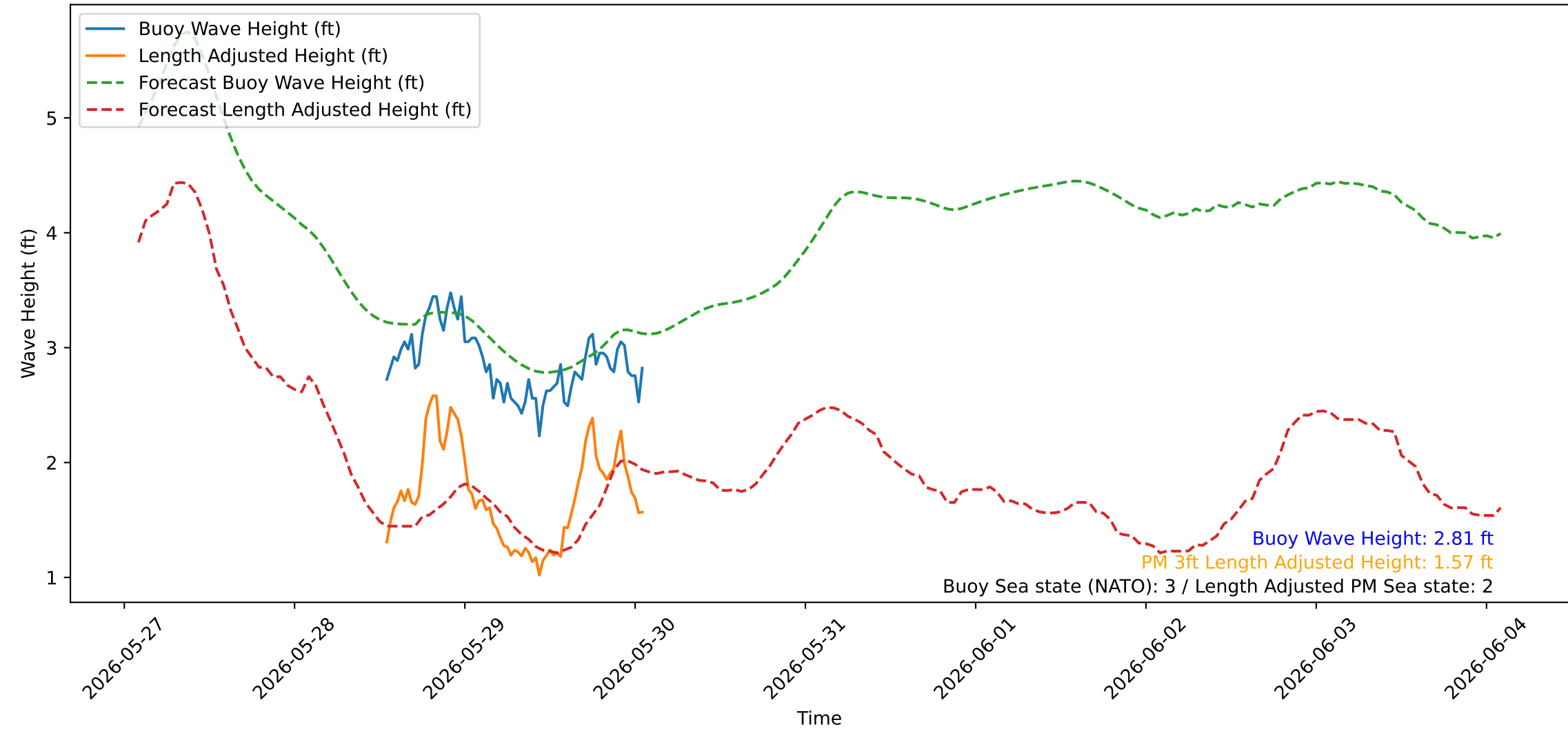
Wave Heights over Time for Oceanside Harbor at 2026-05-30 01:50:22
