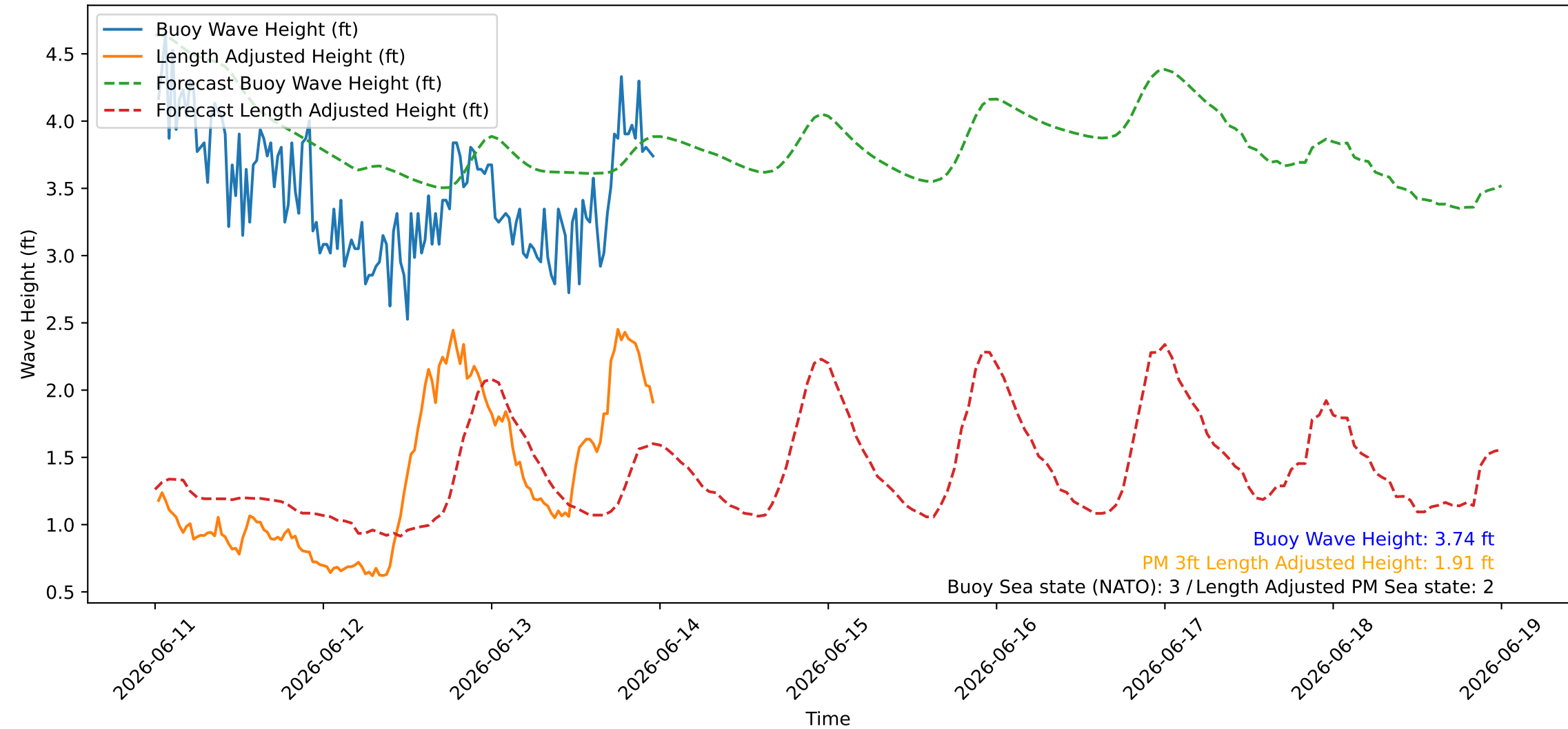
Wave Heights over Time for Red Beach at 2026-06-14 00:00:45
