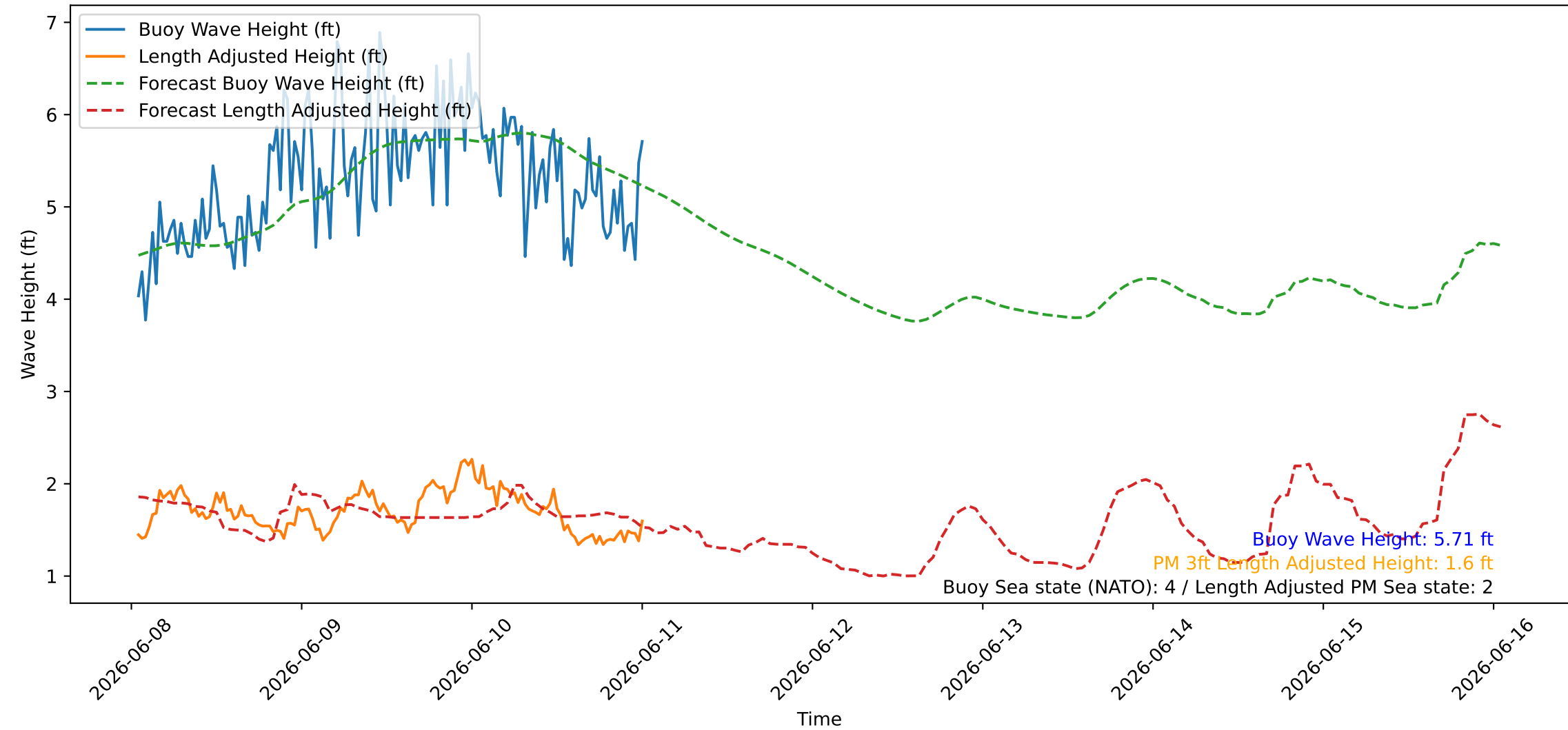
Wave Heights over Time for Green Beach at 2026-06-11 01:01:09
