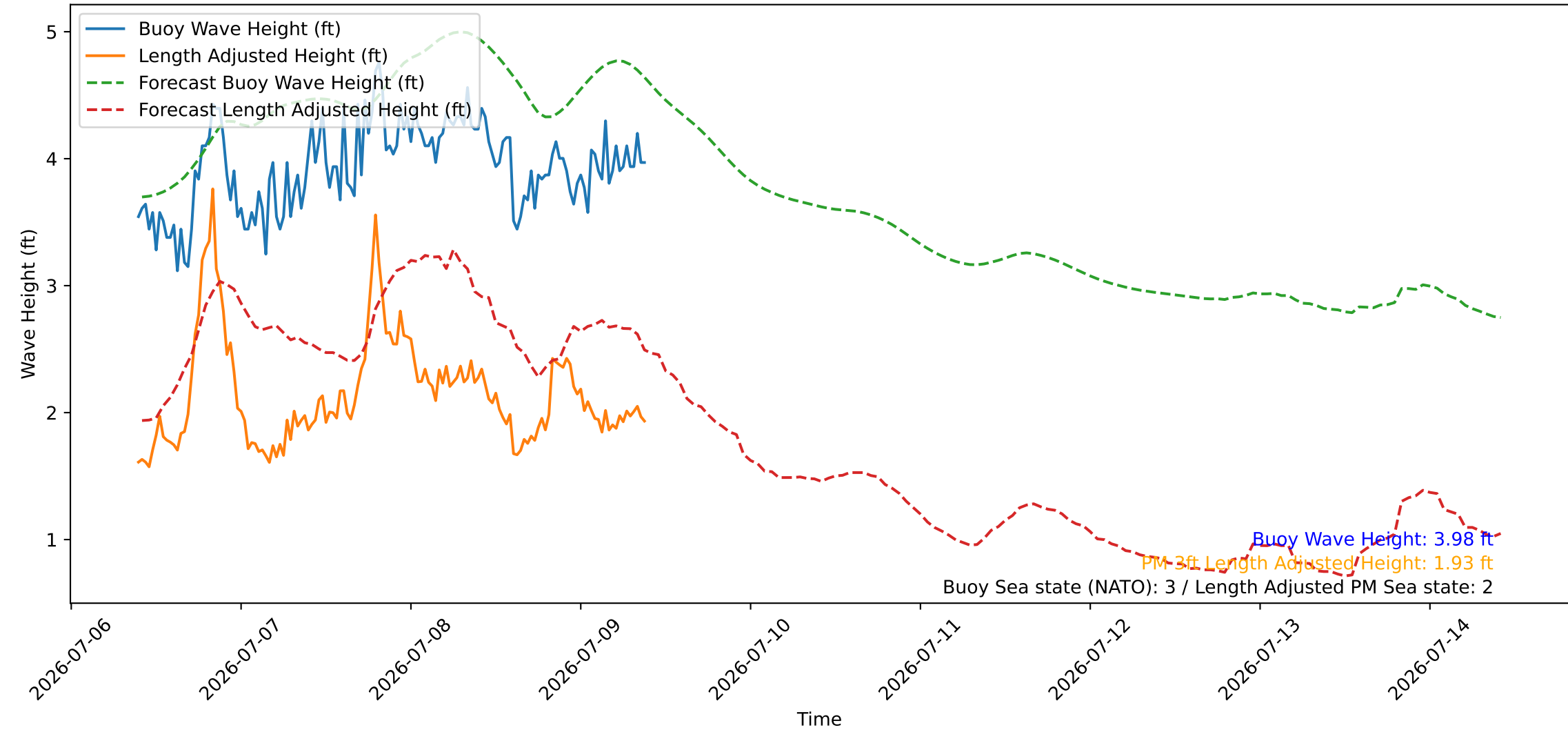
Wave Heights over Time for Green Beach at 2026-07-09 09:41:09
