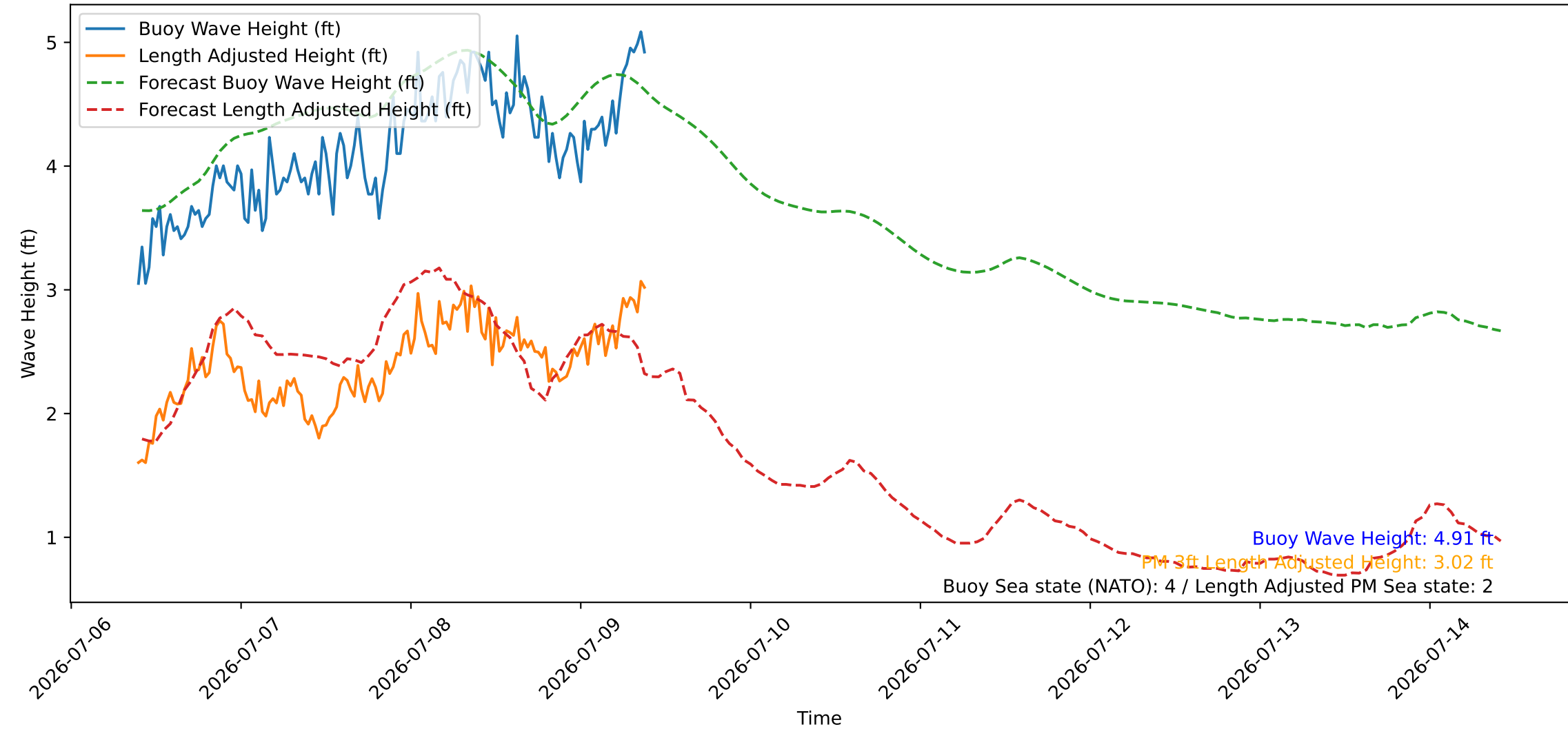
Wave Heights over Time for Oceanside Harbor at 2026-07-09 09:40:27
