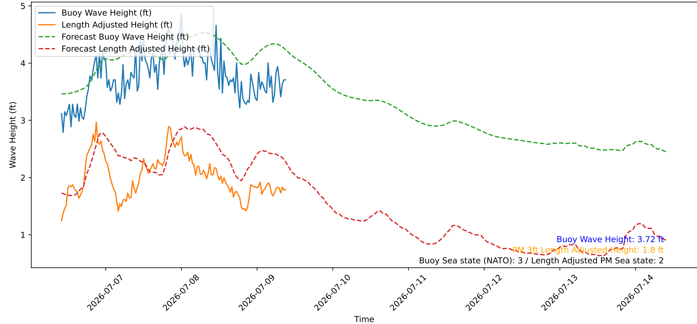
Wave Heights over Time for Red Beach at 2026-07-09 09:40:47
