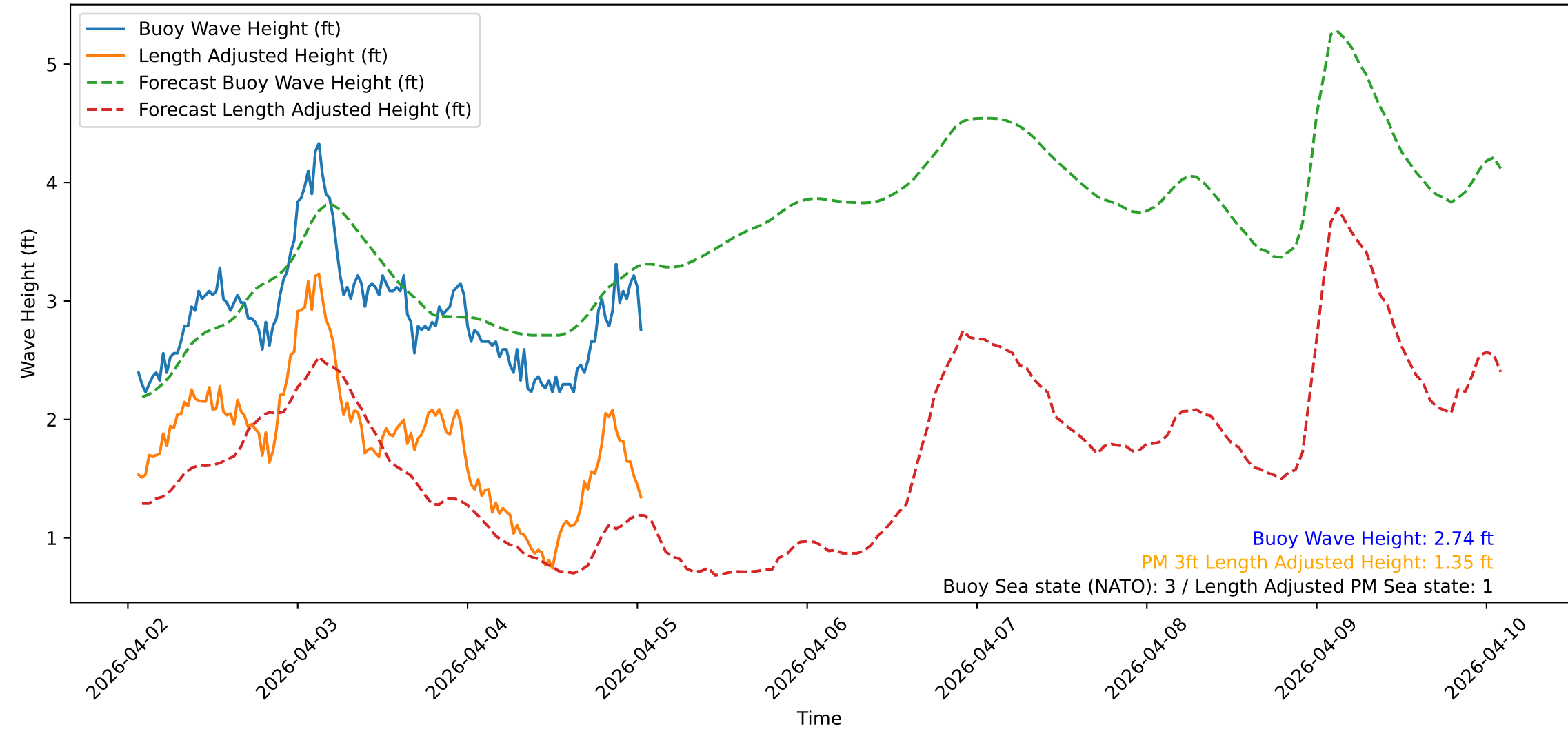
Wave Heights over Time for Green Beach at 2026-04-05 01:31:09
