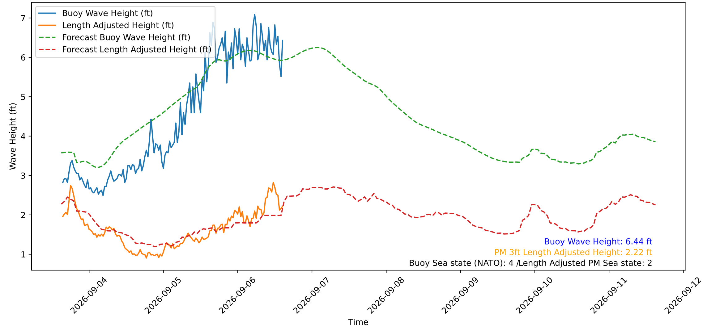
Wave Heights over Time for Green Beach at 2026-09-06 15:21:14
