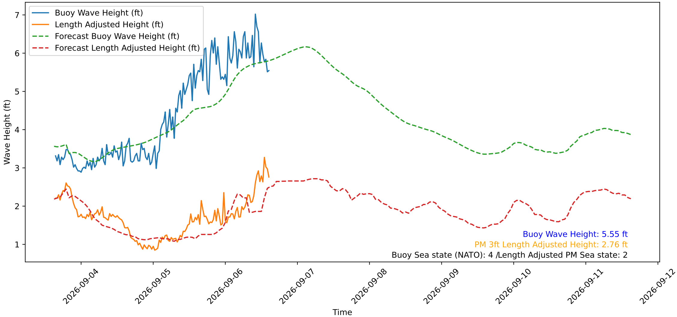
Wave Heights over Time for Oceanside Harbor at 2026-09-06 15:20:30
