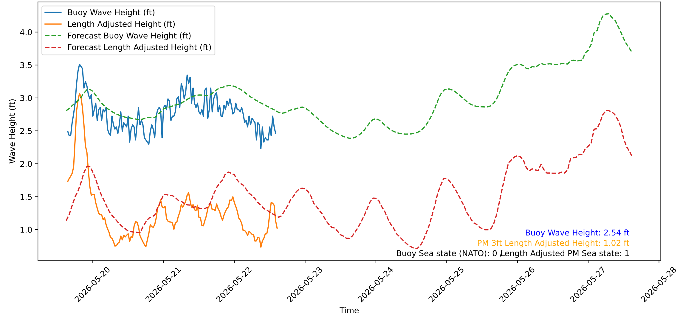
Wave Heights over Time for Red Beach at 2026-05-22 15:20:53
