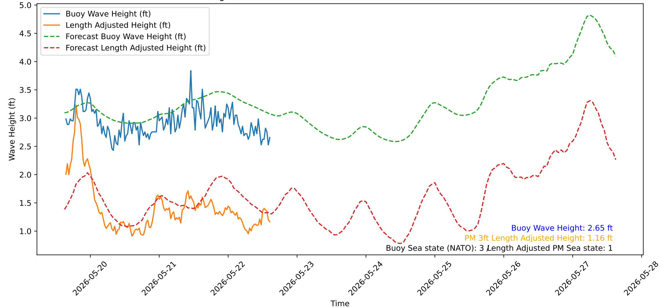
Wave Heights over Time for Oceanside Harbor at 2026-05-22 15:20:32
