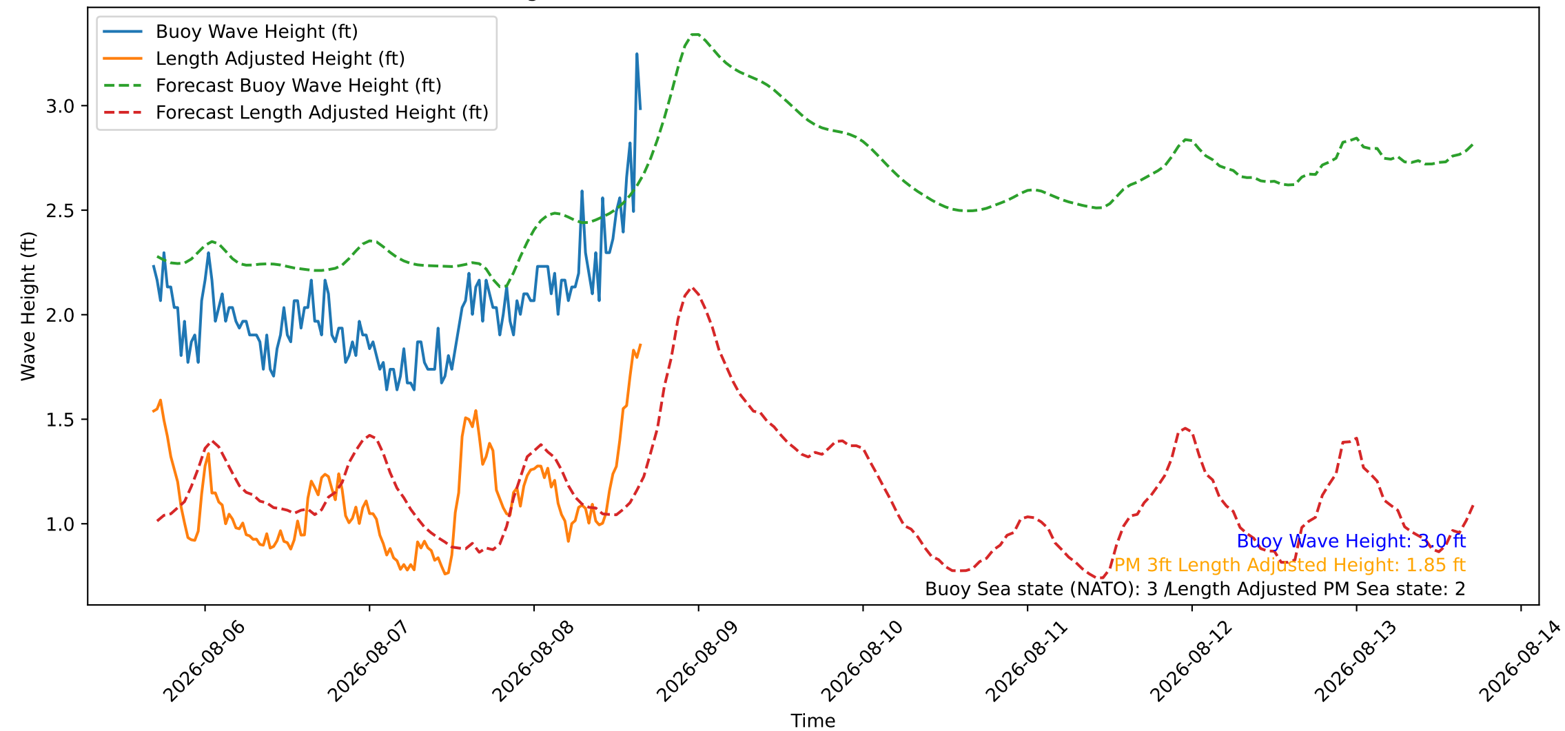
Wave Heights over Time for Oceanside Harbor at 2026-08-08 16:30:26
