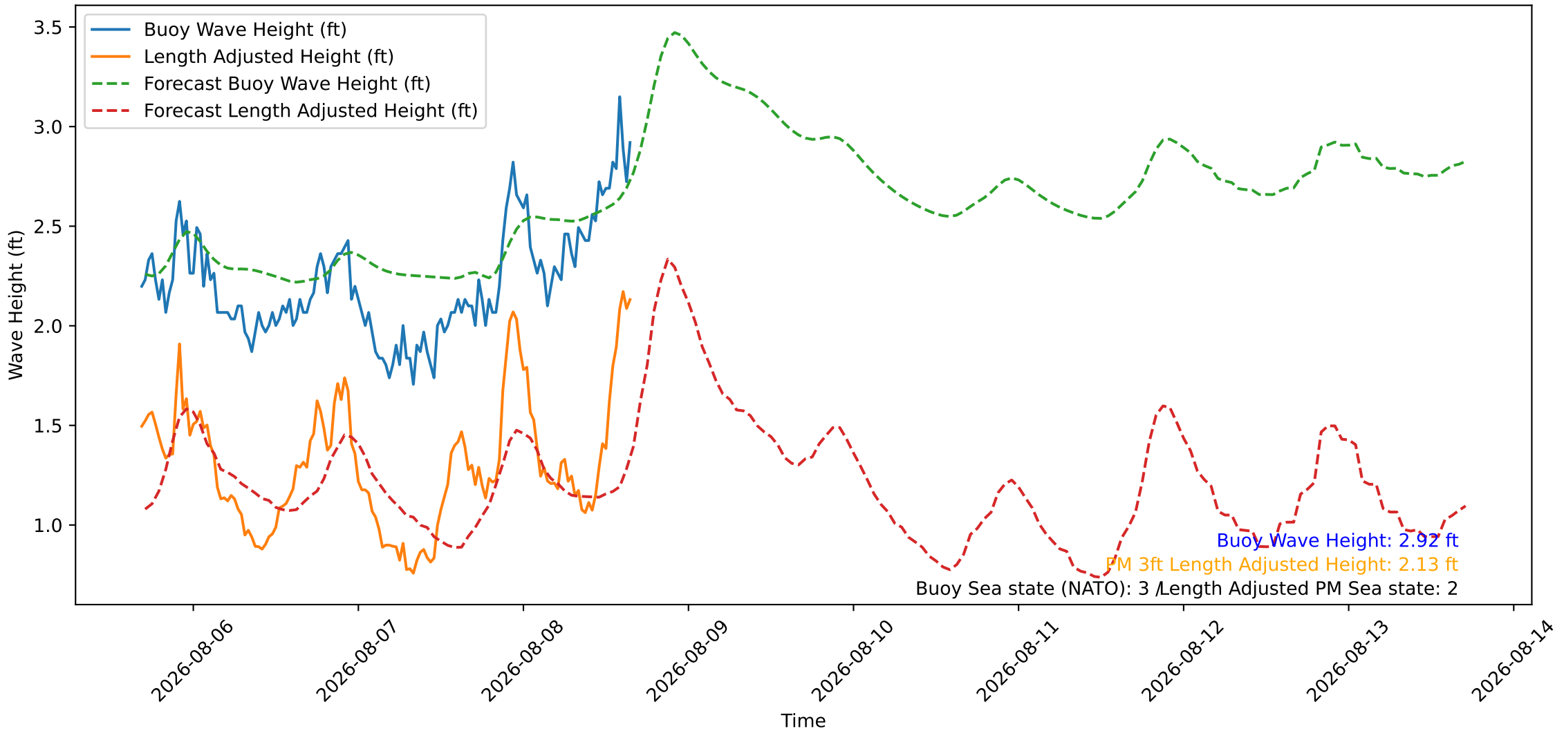
Wave Heights over Time for Green Beach at 2026-08-08 16:31:08
