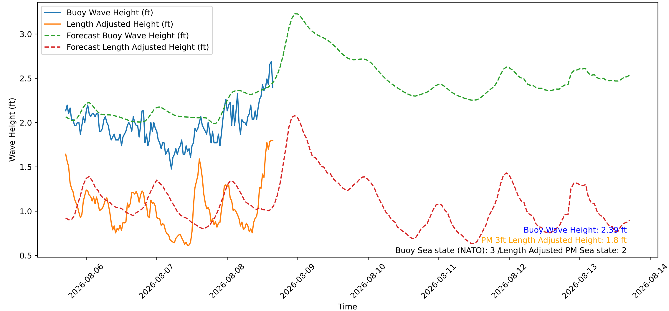
Wave Heights over Time for Red Beach at 2026-08-08 16:30:46
