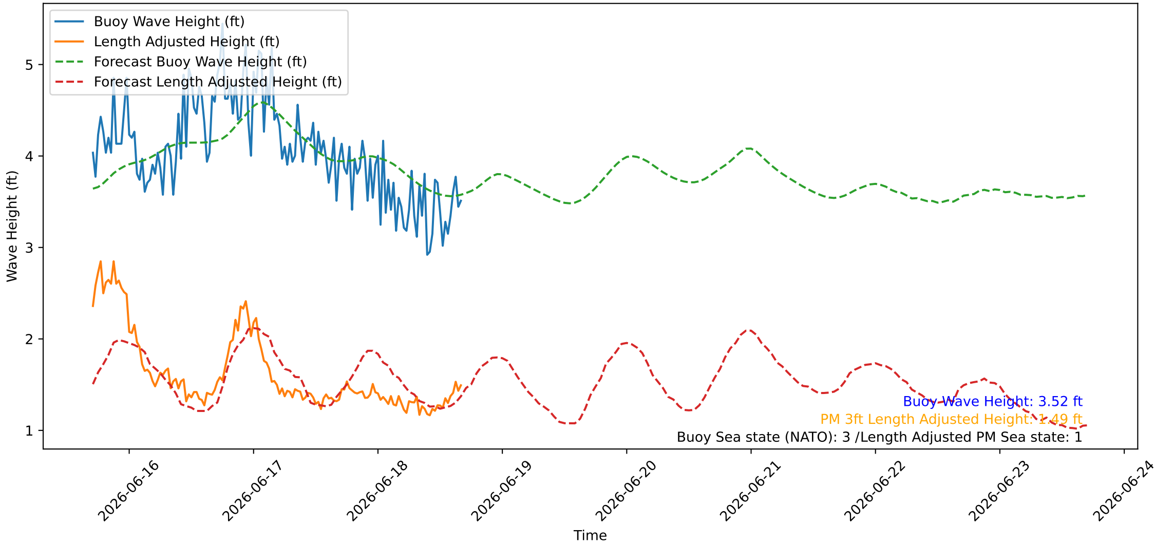
Wave Heights over Time for Oceanside Harbor at 2026-06-18 17:00:26
