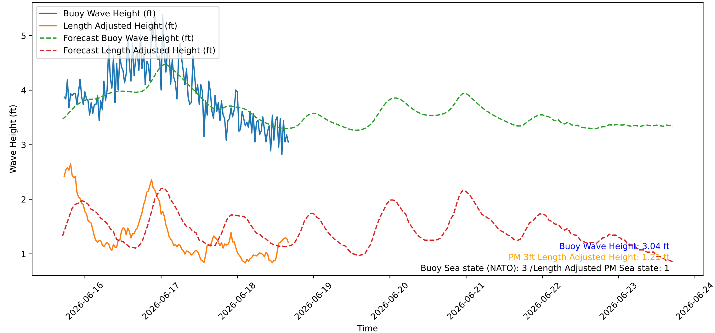
Wave Heights over Time for Red Beach at 2026-06-18 17:00:45
