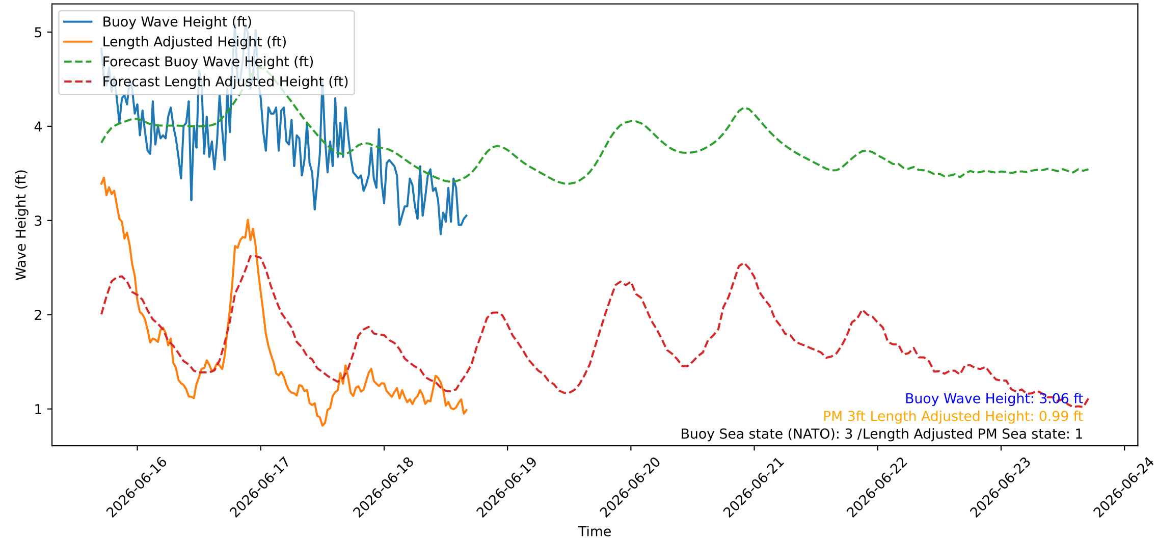
Wave Heights over Time for Green Beach at 2026-06-18 17:01:08
