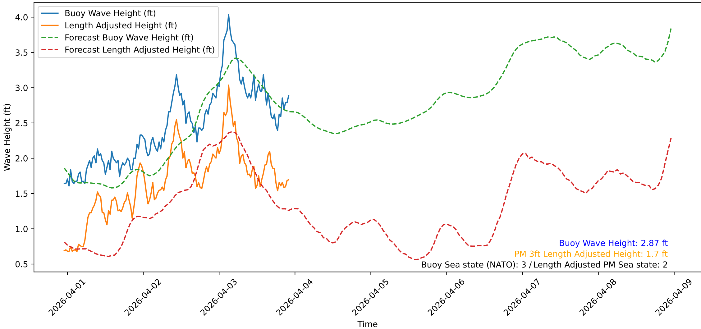
Wave Heights over Time for Oceanside Harbor at 2026-04-03 22:50:36
