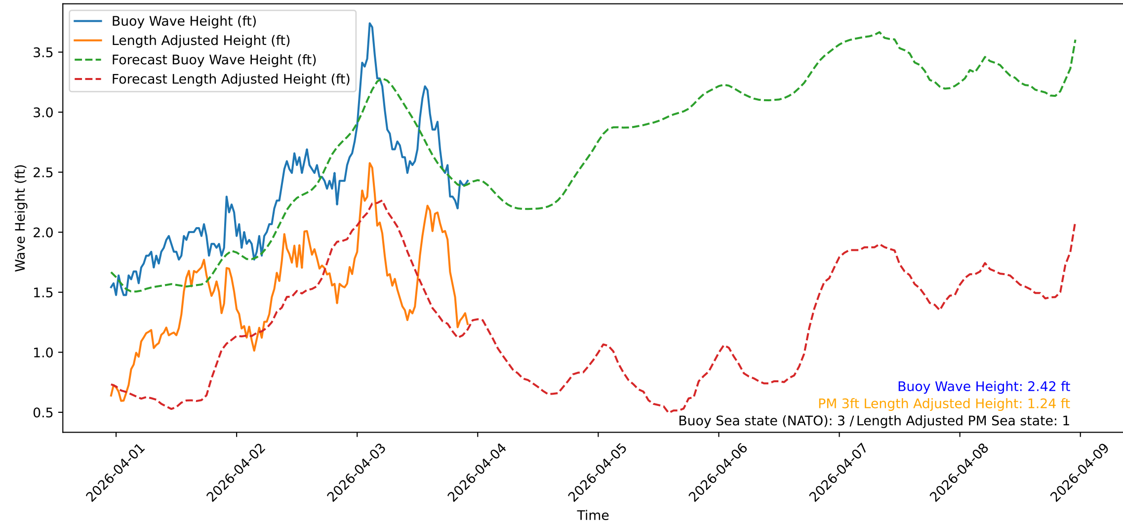
Wave Heights over Time for Red Beach at 2026-04-03 22:50:56
