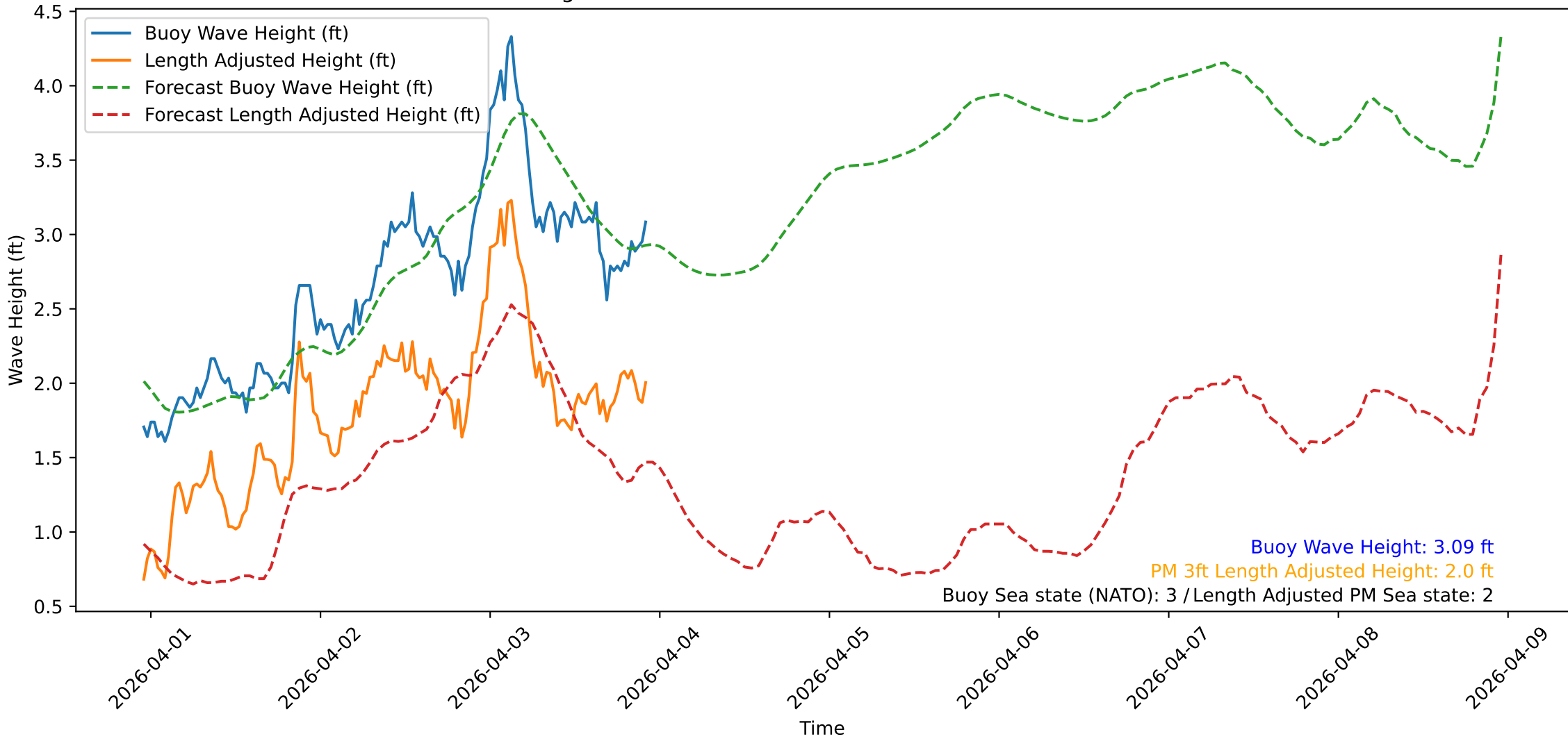
Wave Heights over Time for Green Beach at 2026-04-03 22:51:26
