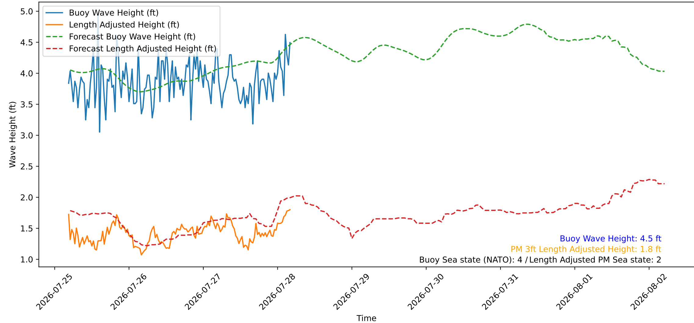
Wave Heights over Time for Oceanside Harbor at 2026-07-28 04:40:26
