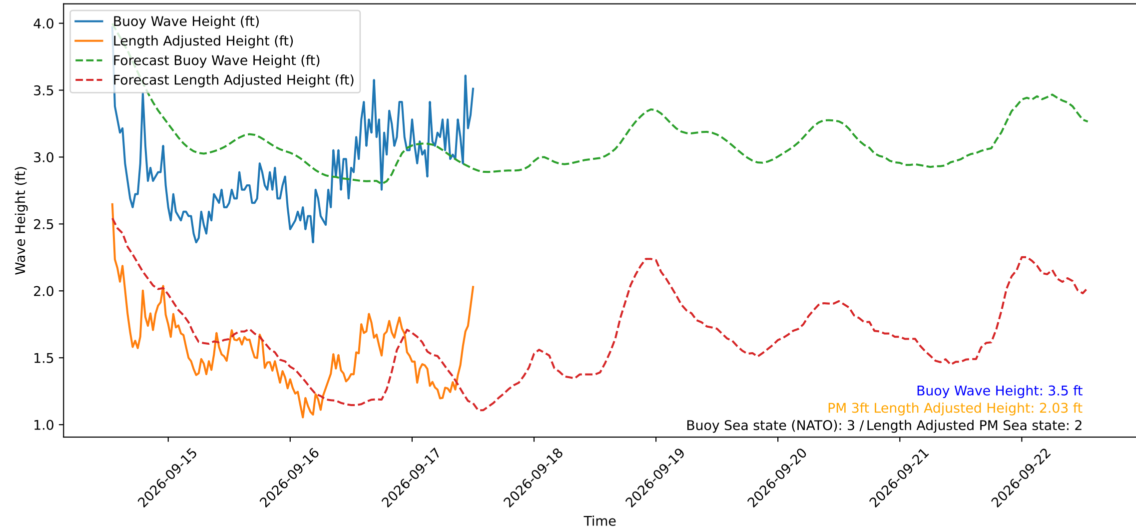
Wave Heights over Time for Oceanside Harbor at 2026-09-17 12:50:29
