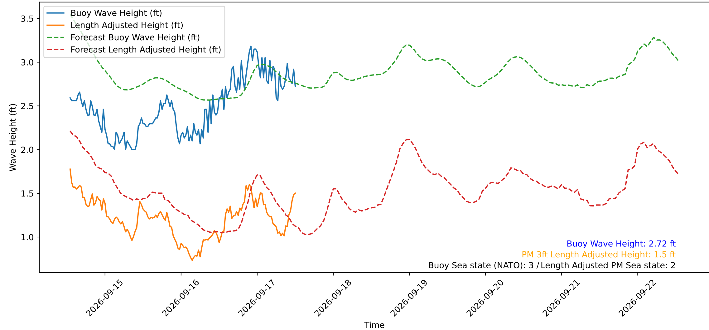
Wave Heights over Time for Red Beach at 2026-09-17 12:50:50
