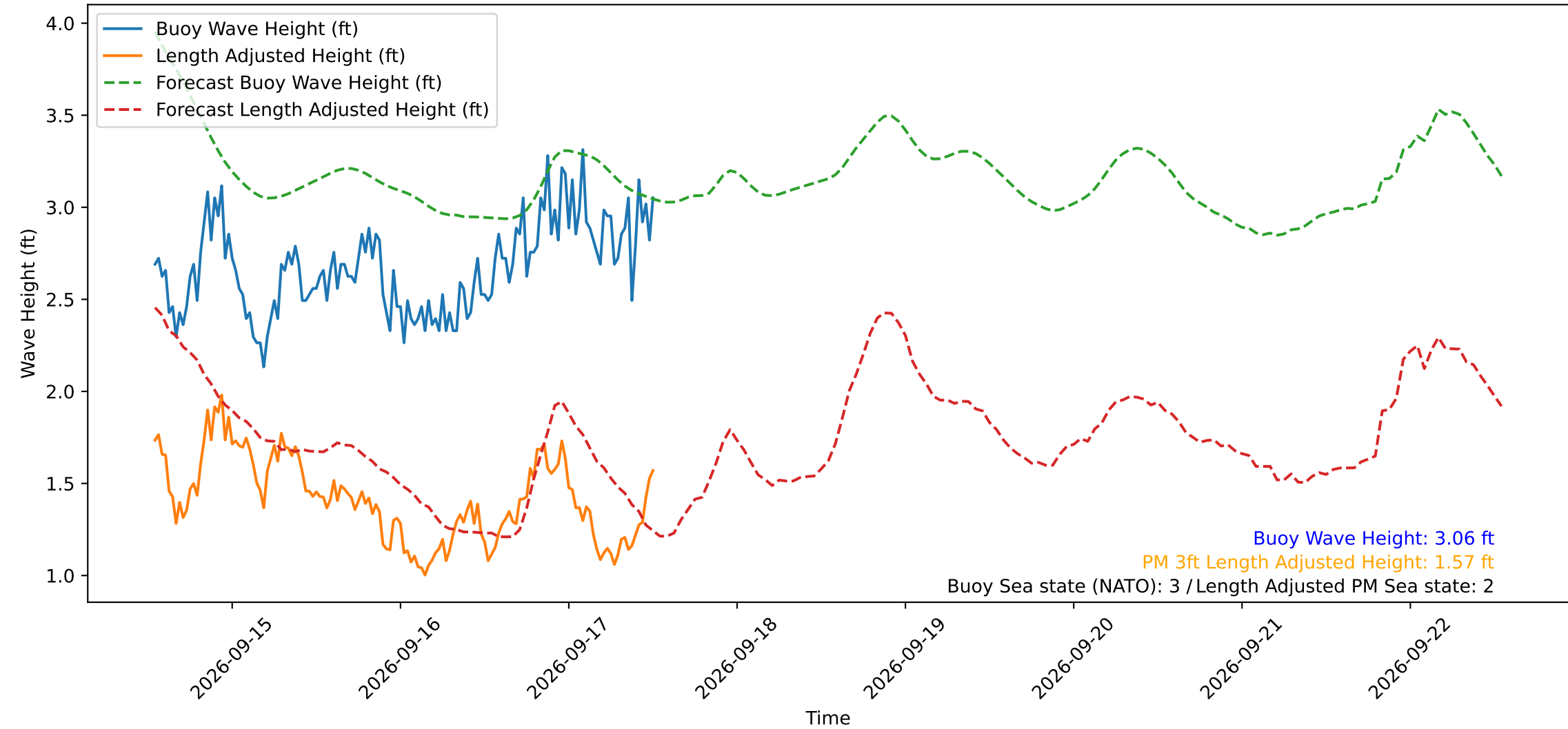
Wave Heights over Time for Green Beach at 2026-09-17 12:51:13
