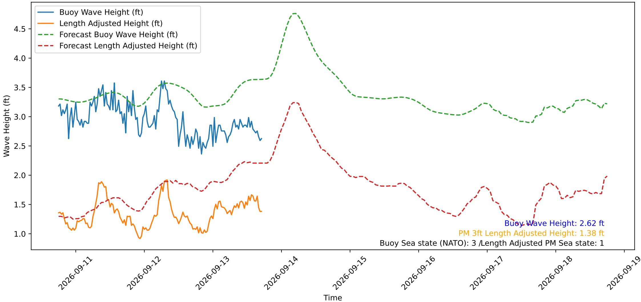
Wave Heights over Time for Green Beach at 2026-09-13 17:51:14
