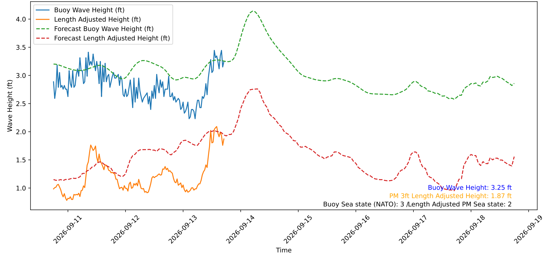
Wave Heights over Time for Red Beach at 2026-09-13 17:50:50
