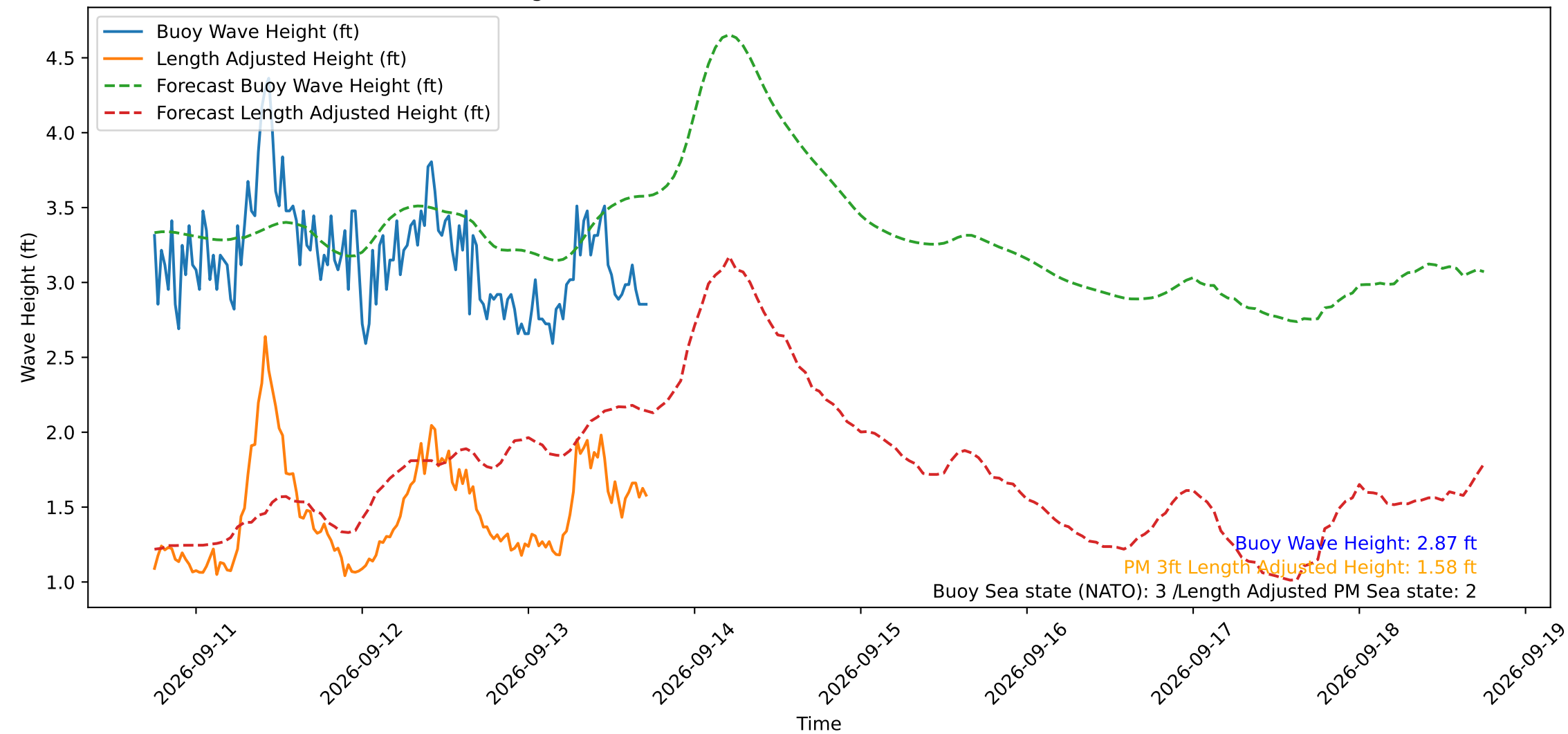
Wave Heights over Time for Oceanside Harbor at 2026-09-13 17:50:29
