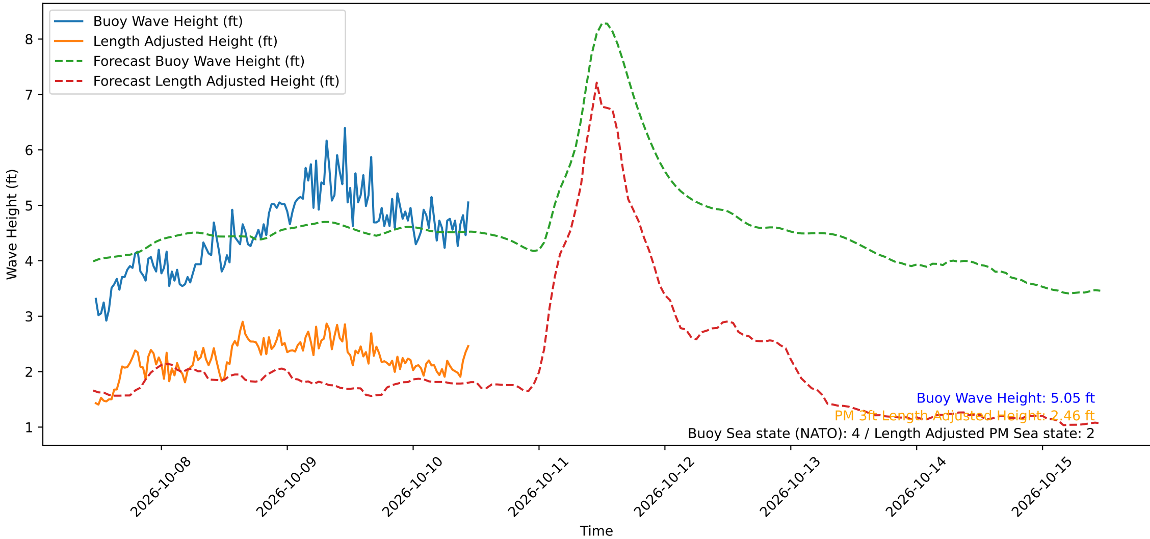
Wave Heights over Time for Oceanside Harbor at 2026-10-10 11:20:29
