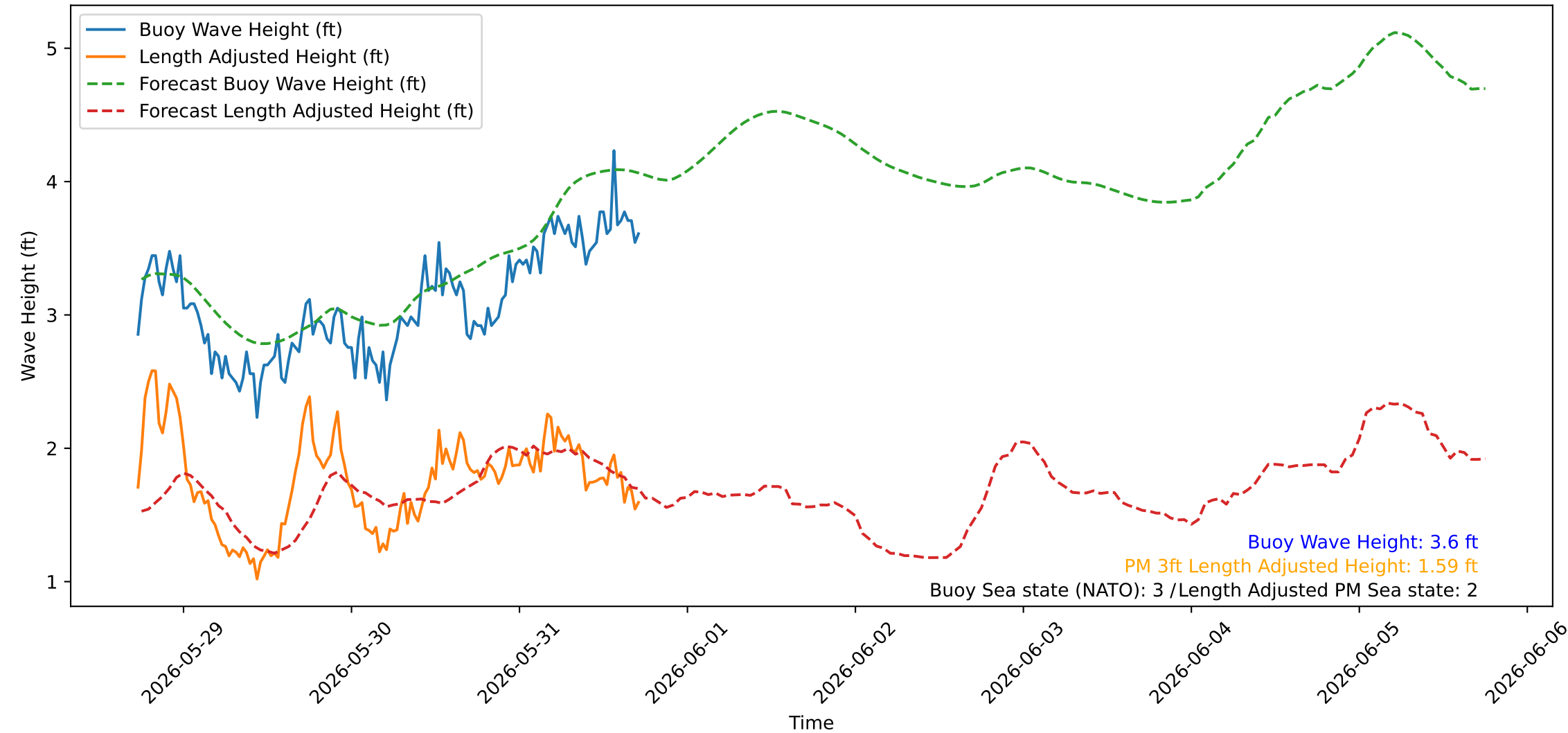
Wave Heights over Time for Oceanside Harbor at 2026-05-31 17:30:26
