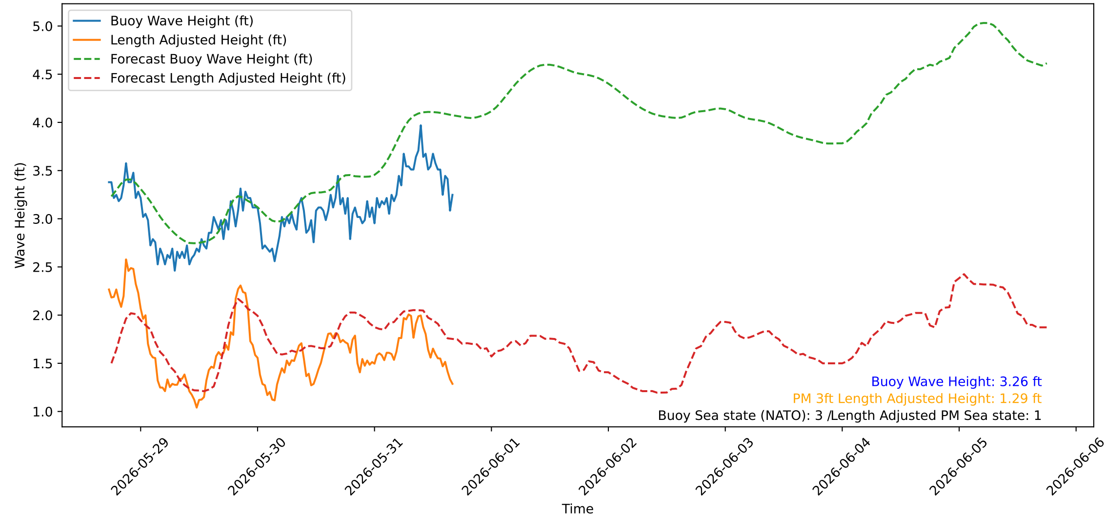
Wave Heights over Time for Green Beach at 2026-05-31 17:31:08
