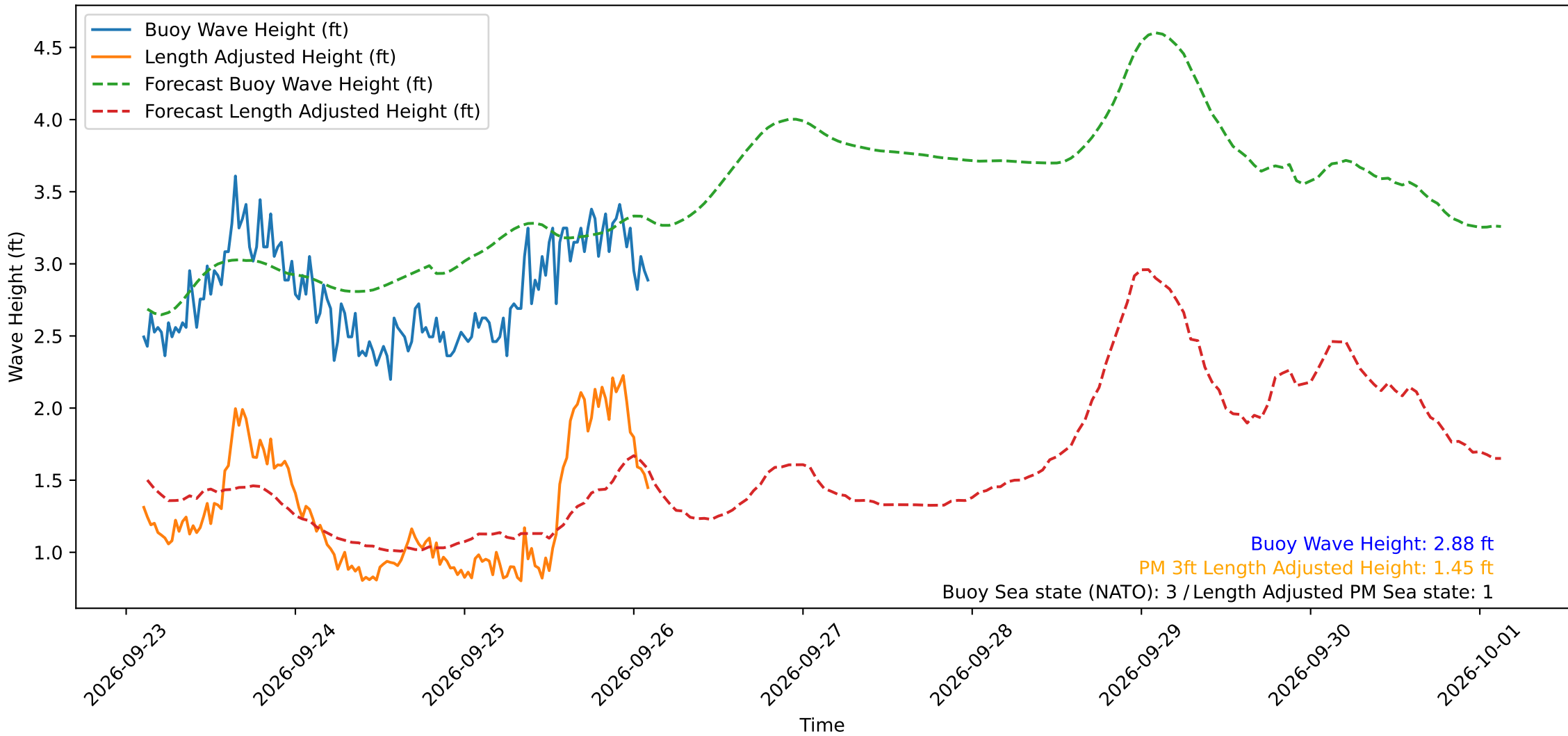
Wave Heights over Time for Oceanside Harbor at 2026-09-26 02:40:29
