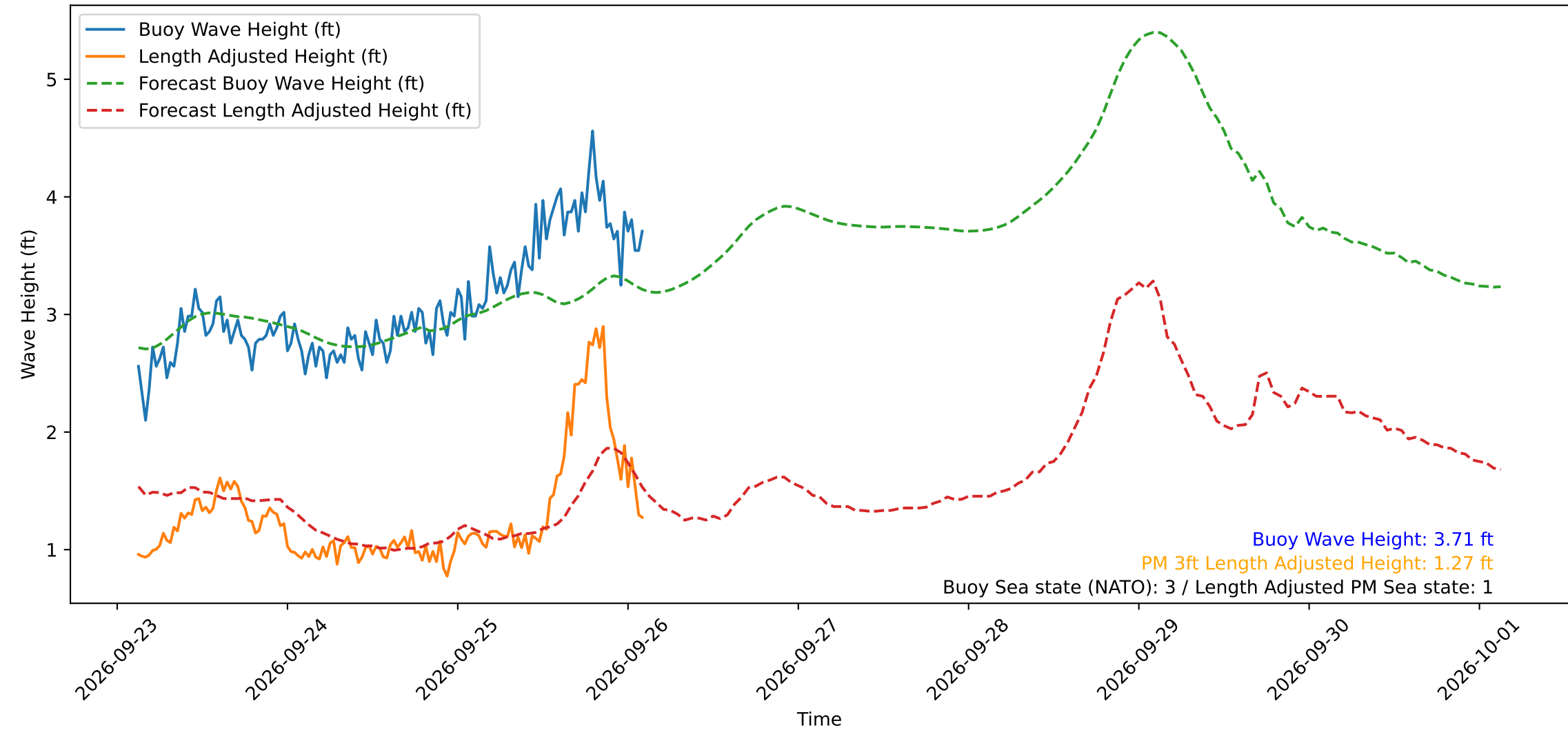
Wave Heights over Time for Green Beach at 2026-09-26 02:41:11
