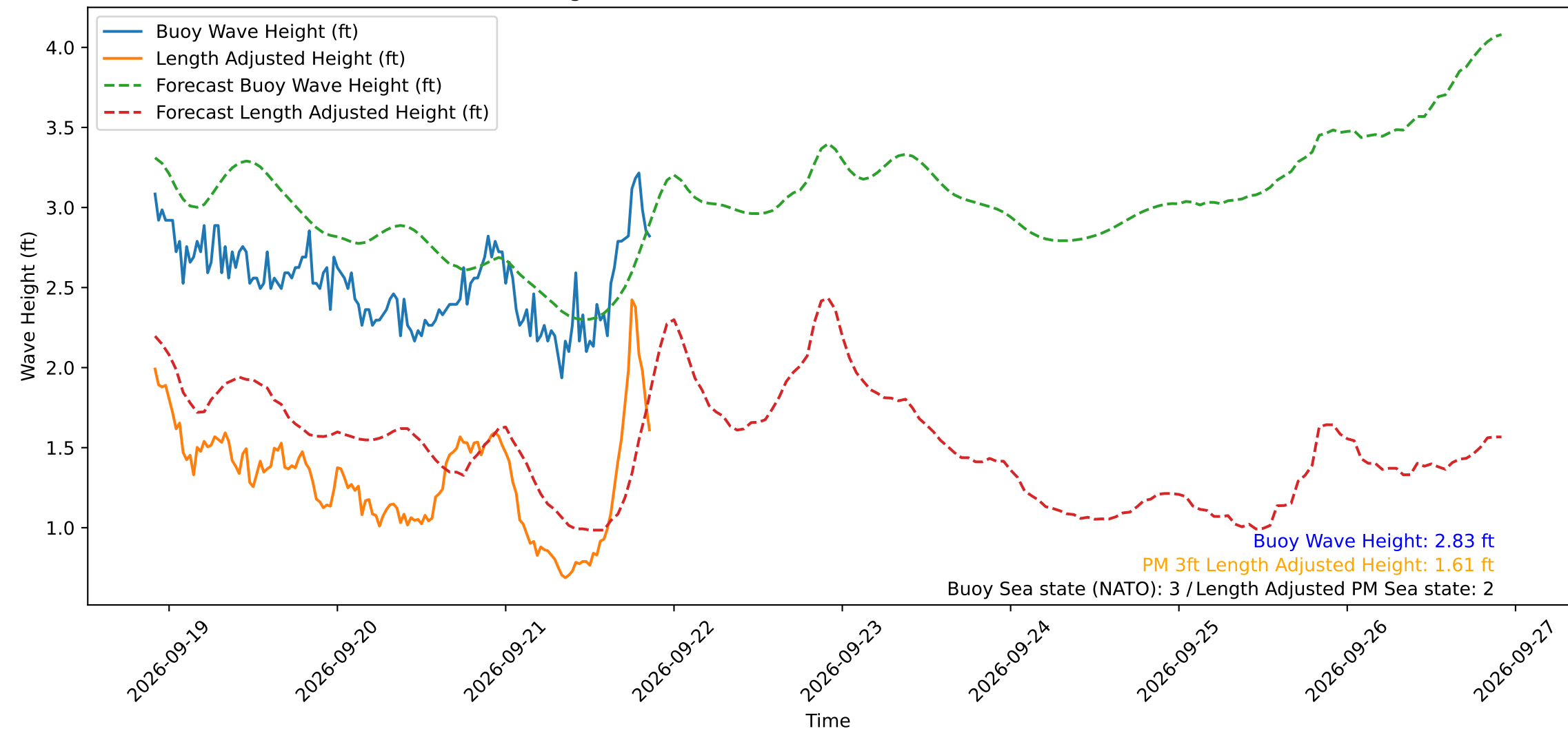
Wave Heights over Time for Green Beach at 2026-09-21 21:31:12
