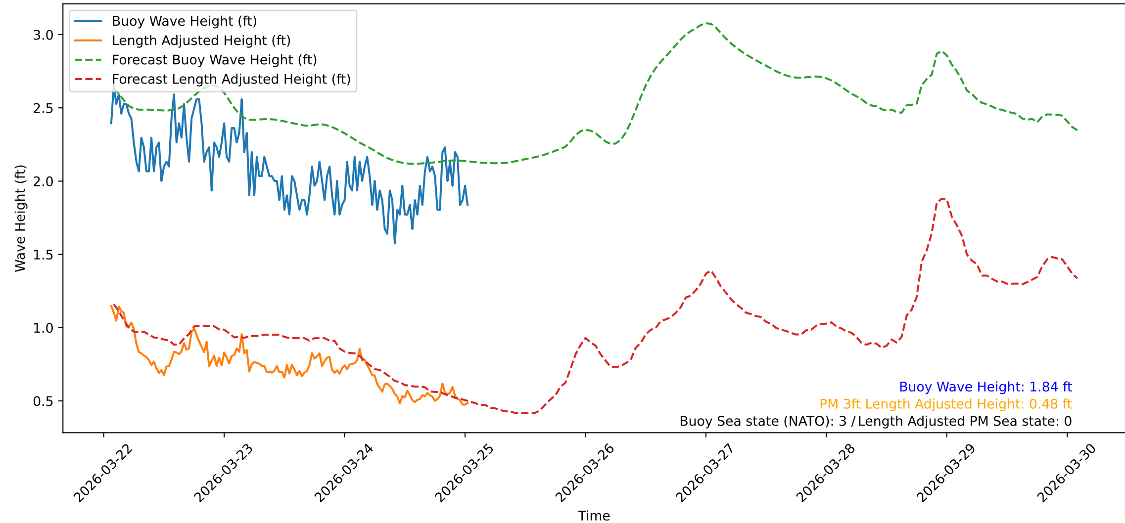
Wave Heights over Time for Oceanside Harbor at 2026-03-25 01:30:31
