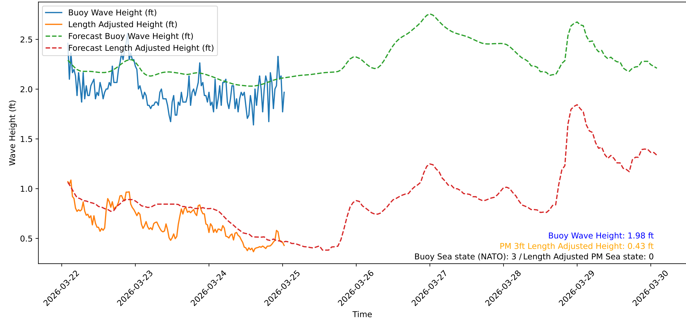
Wave Heights over Time for Red Beach at 2026-03-25 01:30:47
