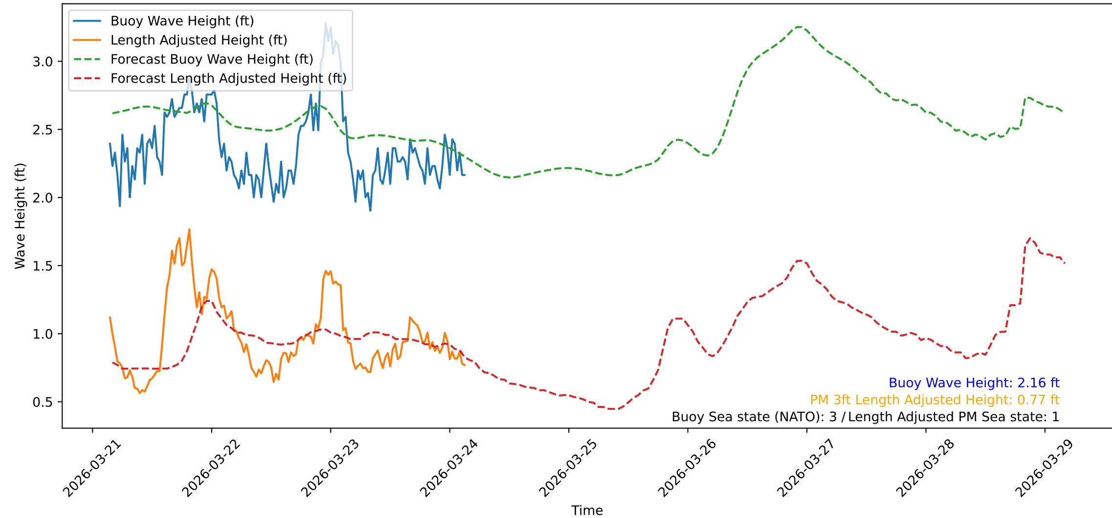
Wave Heights over Time for Green Beach at 2026-03-24 03:41:08
