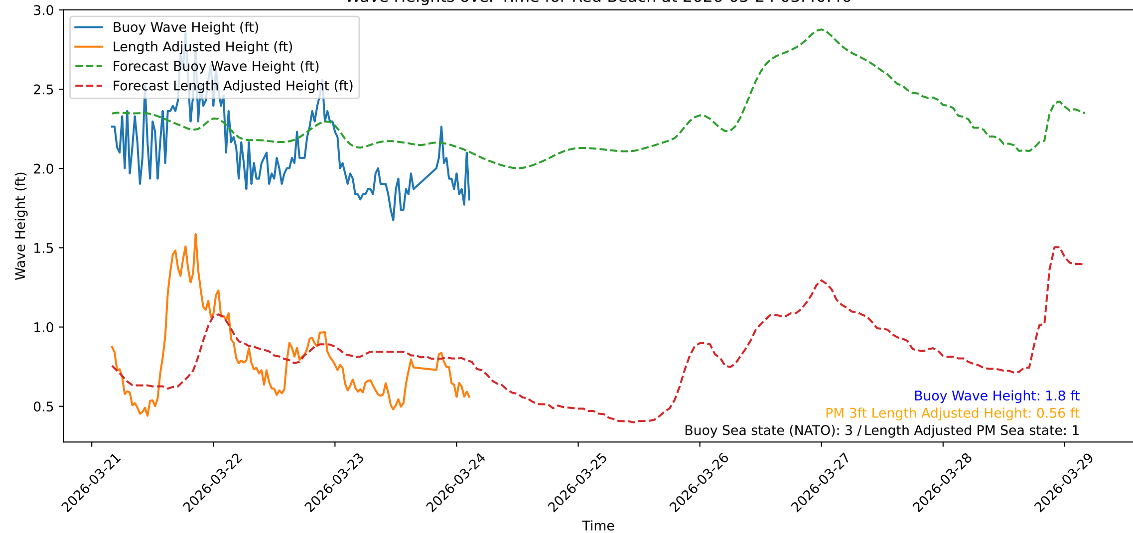
Wave Heights over Time for Red Beach at 2026-03-24 03:40:46
