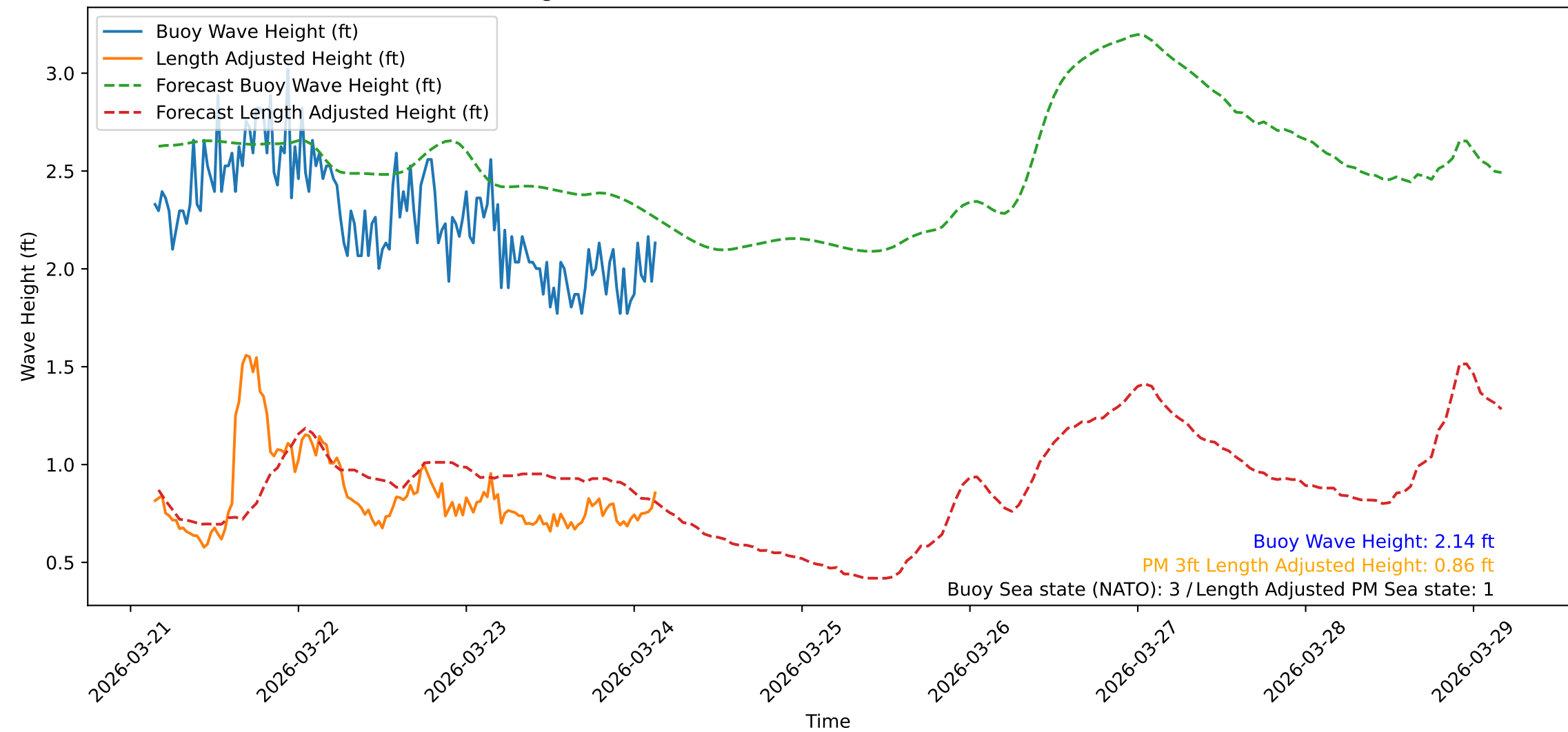
Wave Heights over Time for Oceanside Harbor at 2026-03-24 03:40:30
