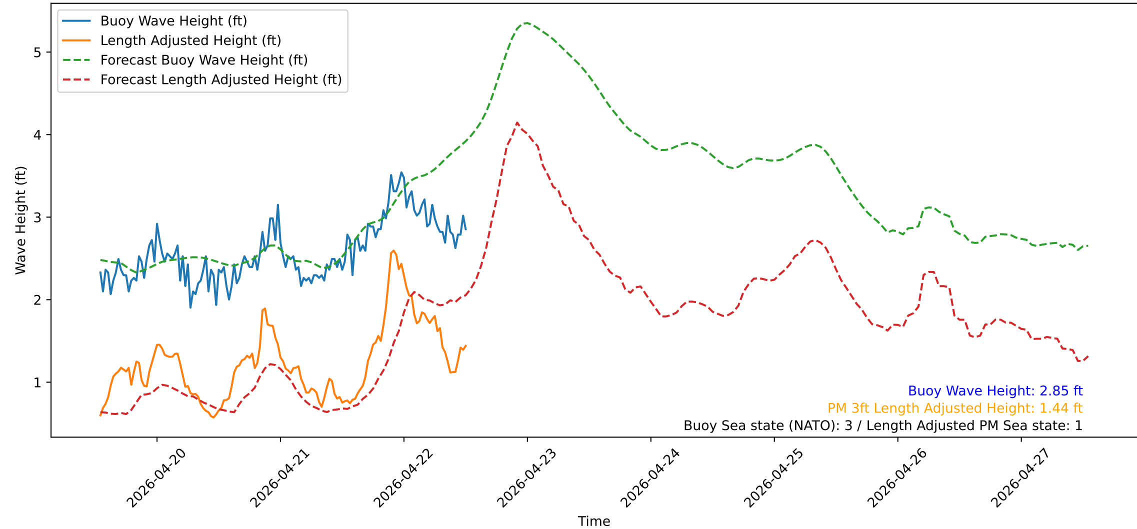
Wave Heights over Time for Green Beach at 2026-04-22 12:51:14
