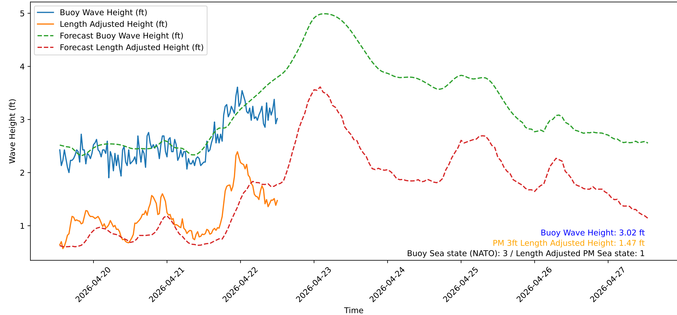
Wave Heights over Time for Oceanside Harbor at 2026-04-22 12:50:31
