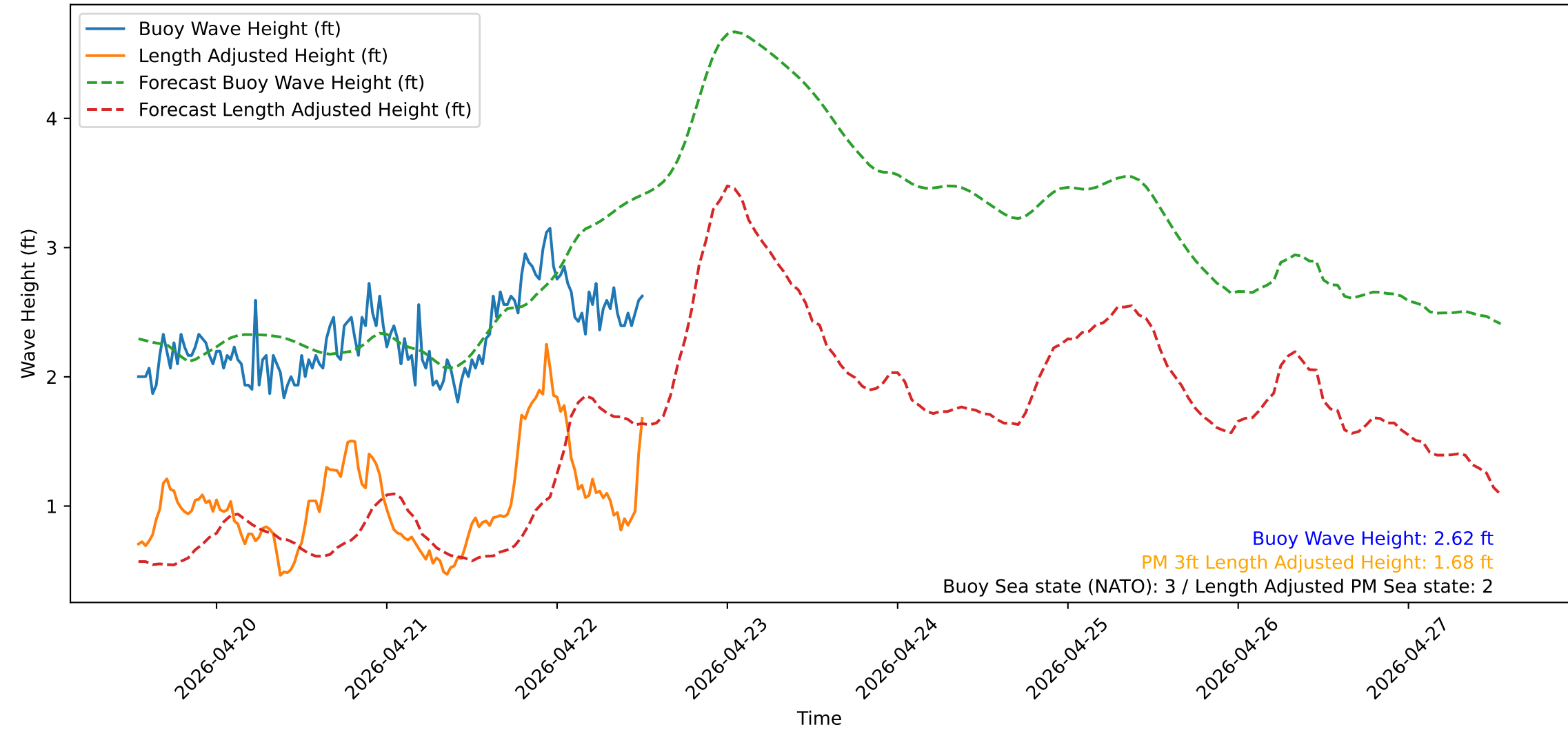
Wave Heights over Time for Red Beach at 2026-04-22 12:50:51
