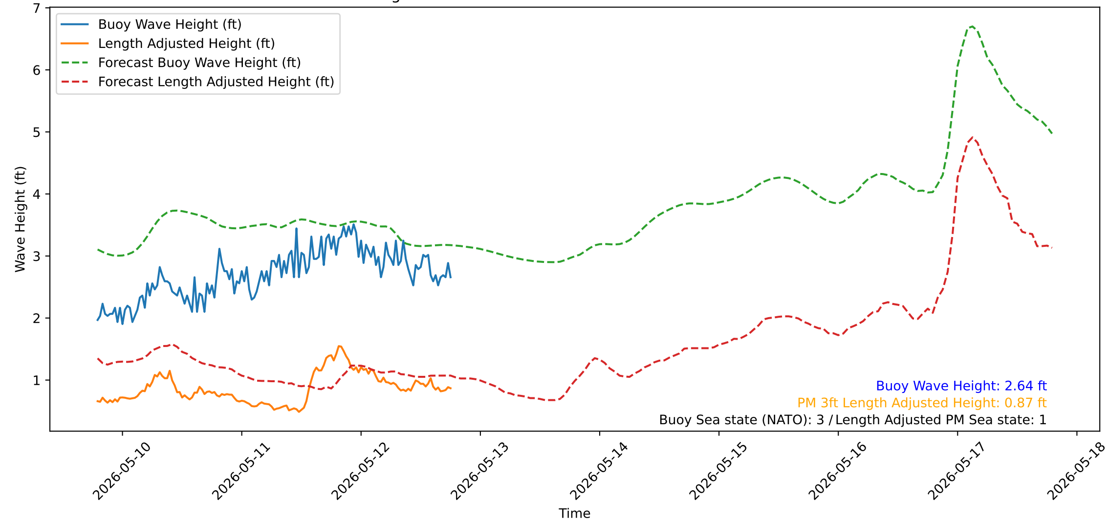
Wave Heights over Time for Green Beach at 2026-05-12 18:51:14
