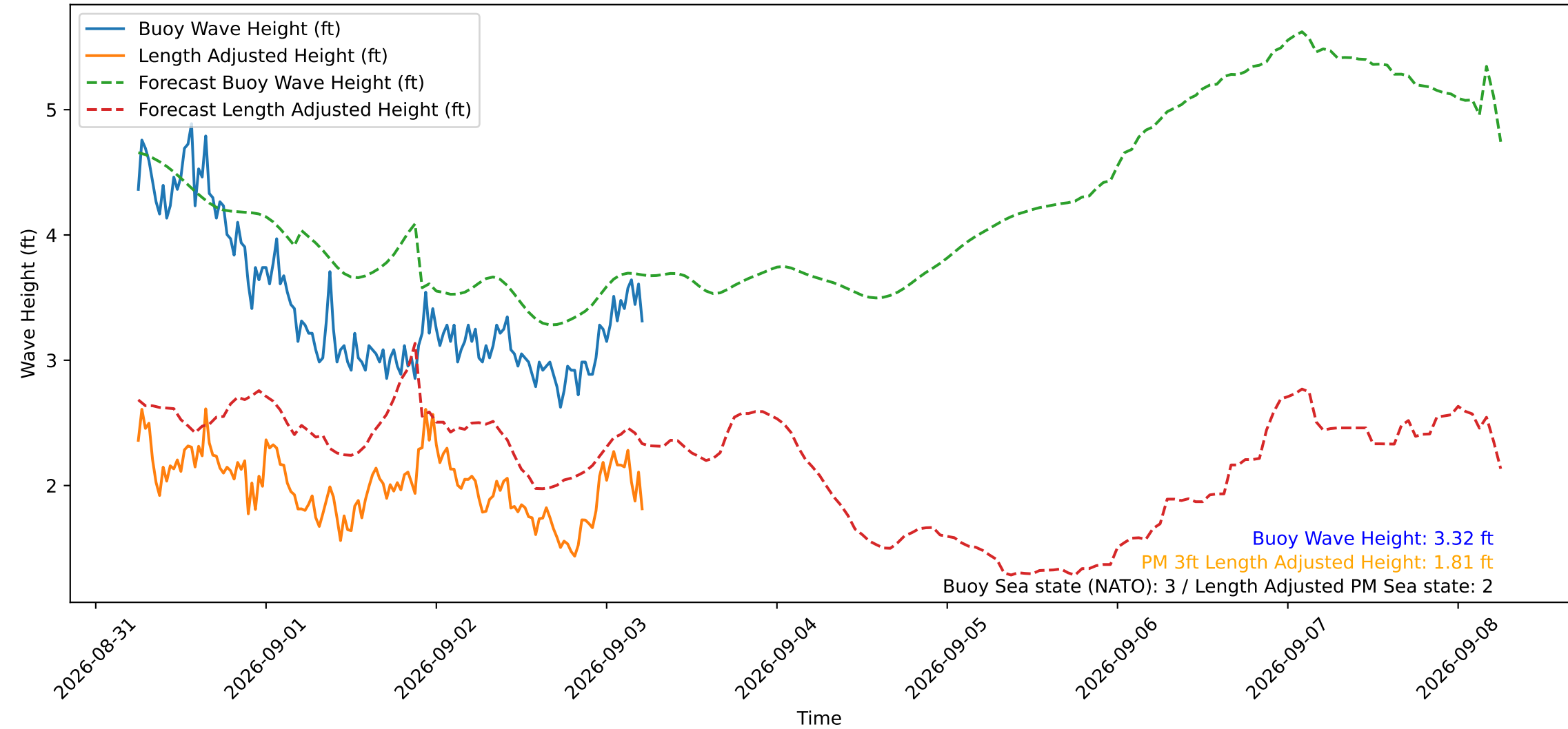
Wave Heights over Time for Oceanside Harbor at 2026-09-03 06:00:29
