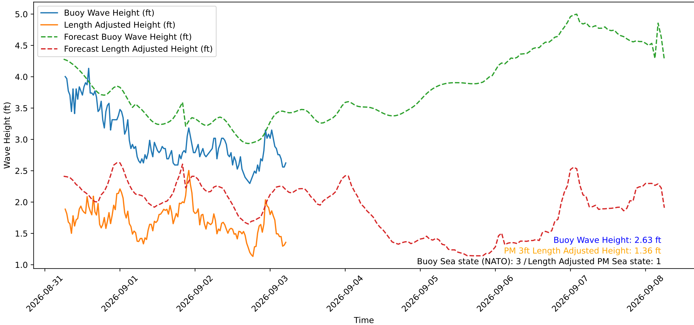
Wave Heights over Time for Red Beach at 2026-09-03 06:00:49
