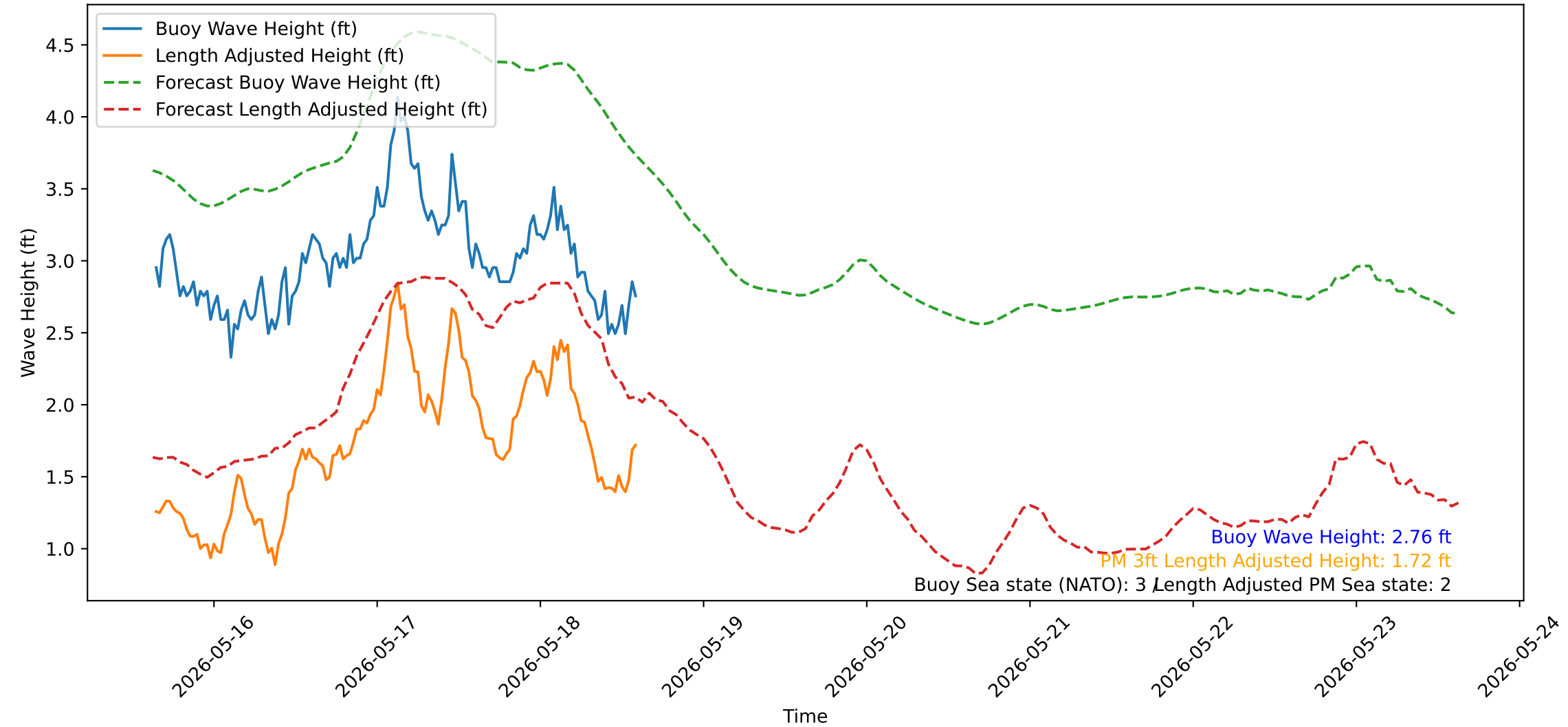
Wave Heights over Time for Red Beach at 2026-05-18 15:00:51
