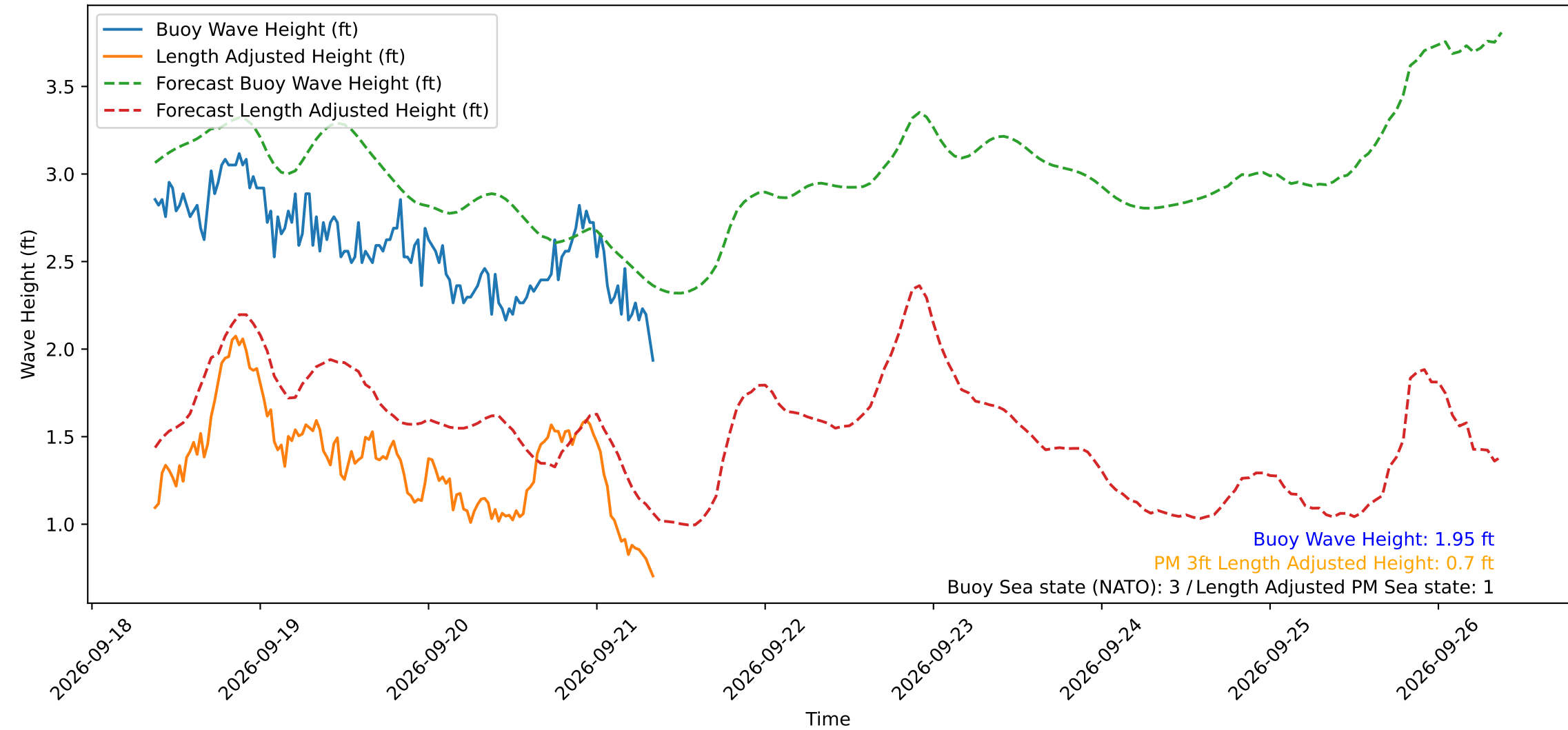
Wave Heights over Time for Green Beach at 2026-09-21 08:41:11
