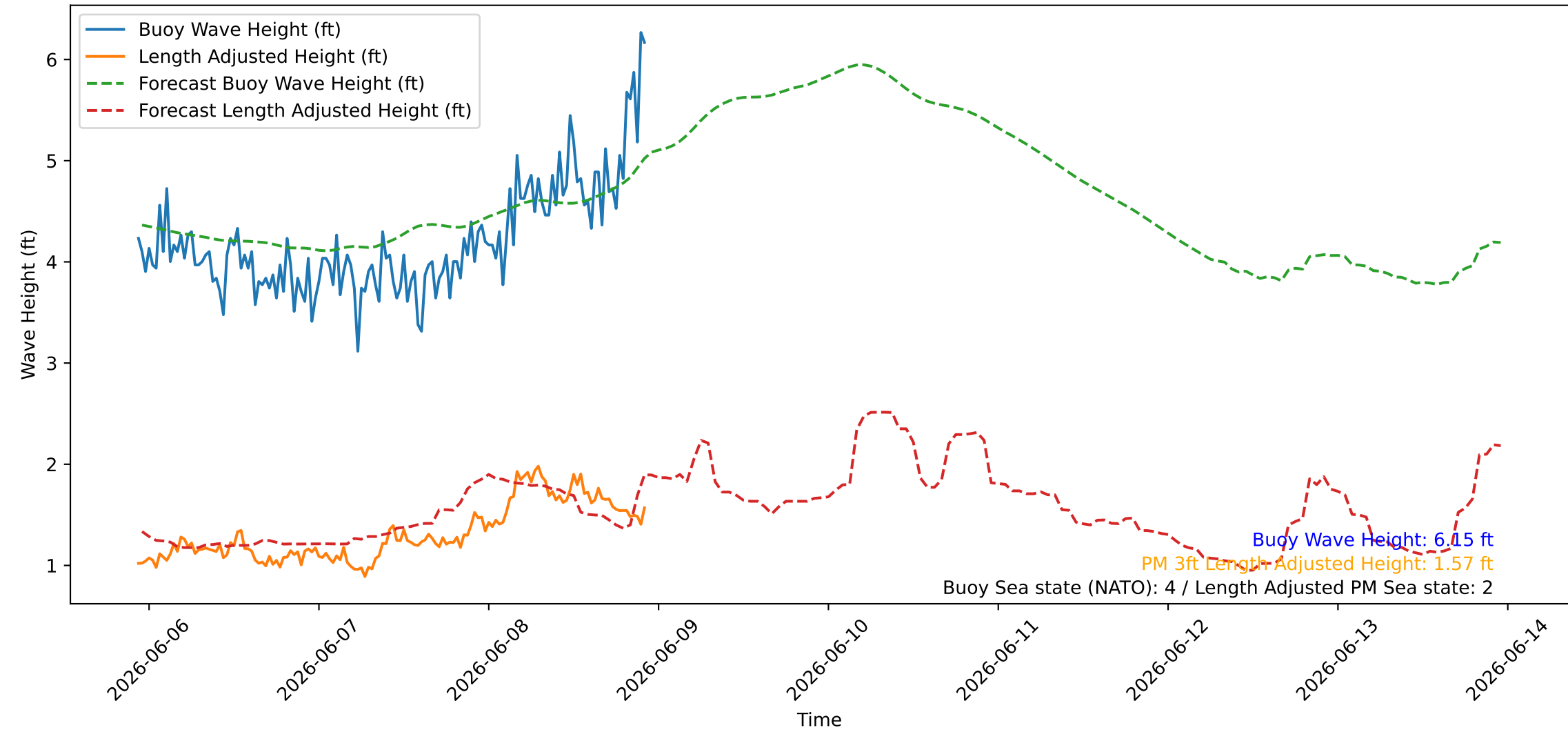
Wave Heights over Time for Green Beach at 2026-06-08 22:41:08
