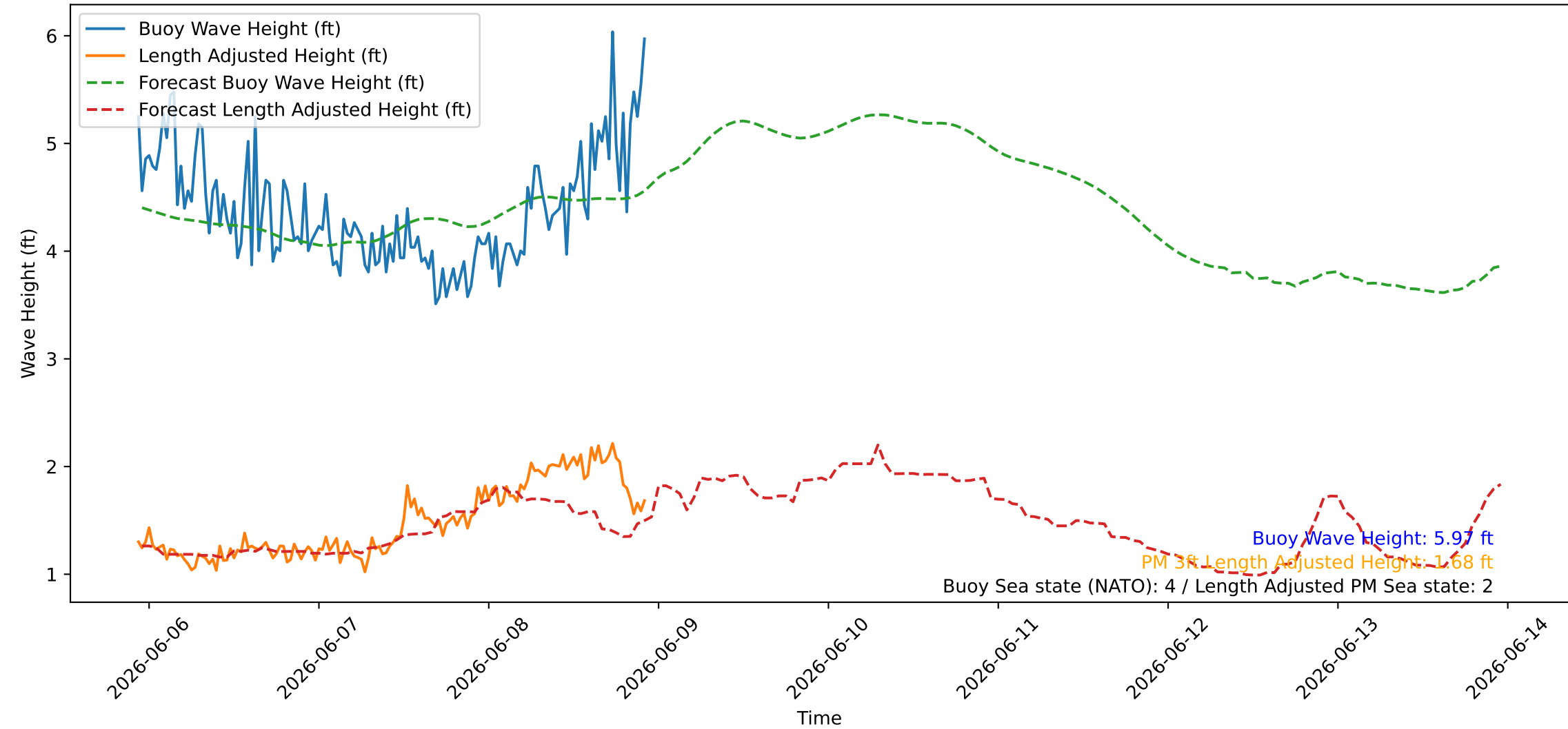
Wave Heights over Time for Oceanside Harbor at 2026-06-08 22:40:26
