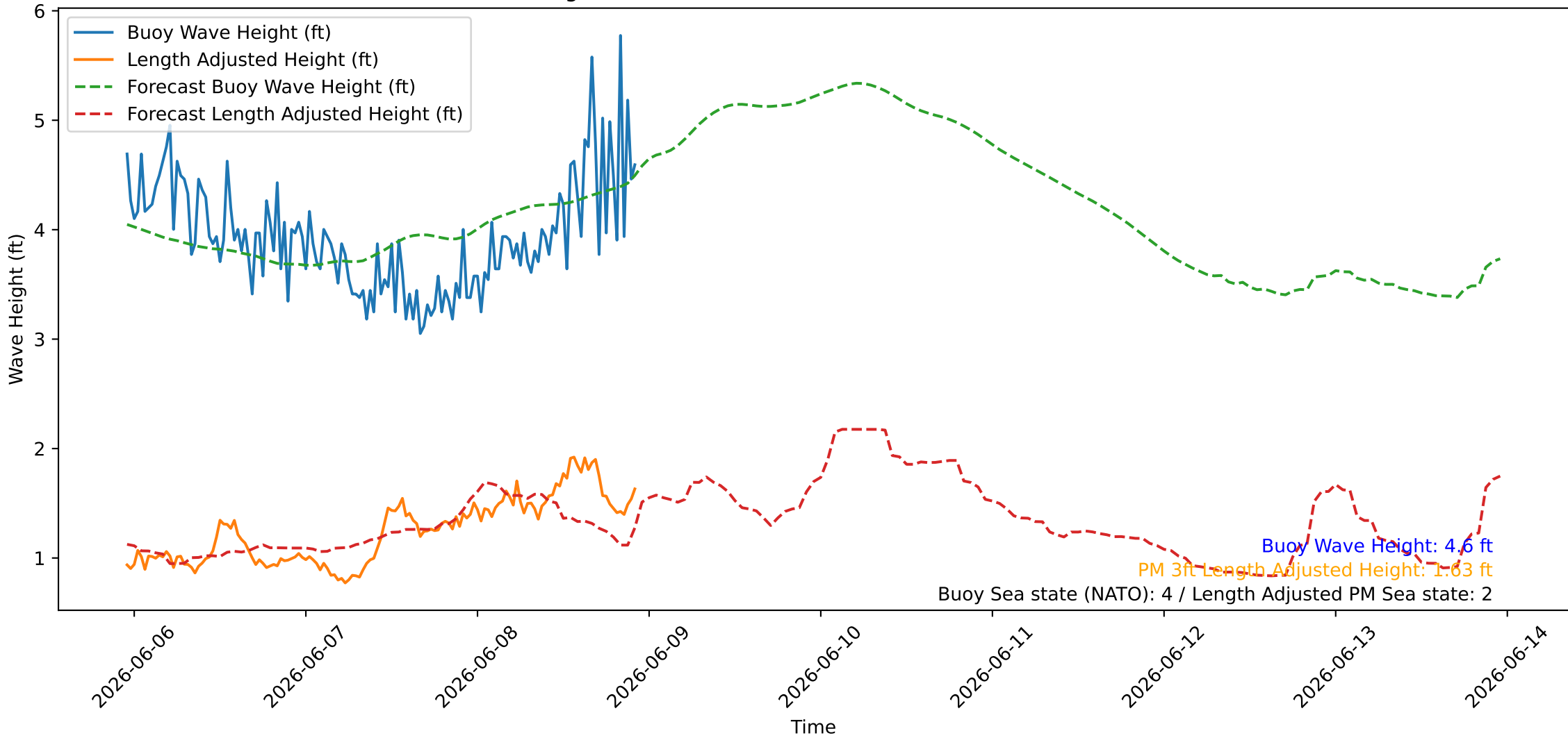
Wave Heights over Time for Red Beach at 2026-06-08 22:40:45
