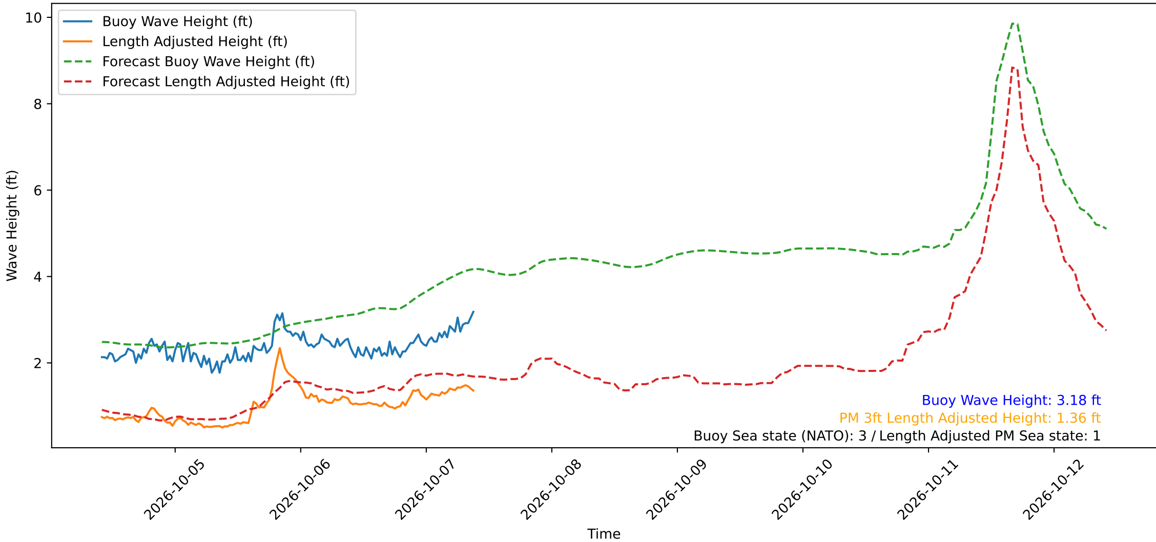
Wave Heights over Time for Green Beach at 2026-10-07 09:51:14
