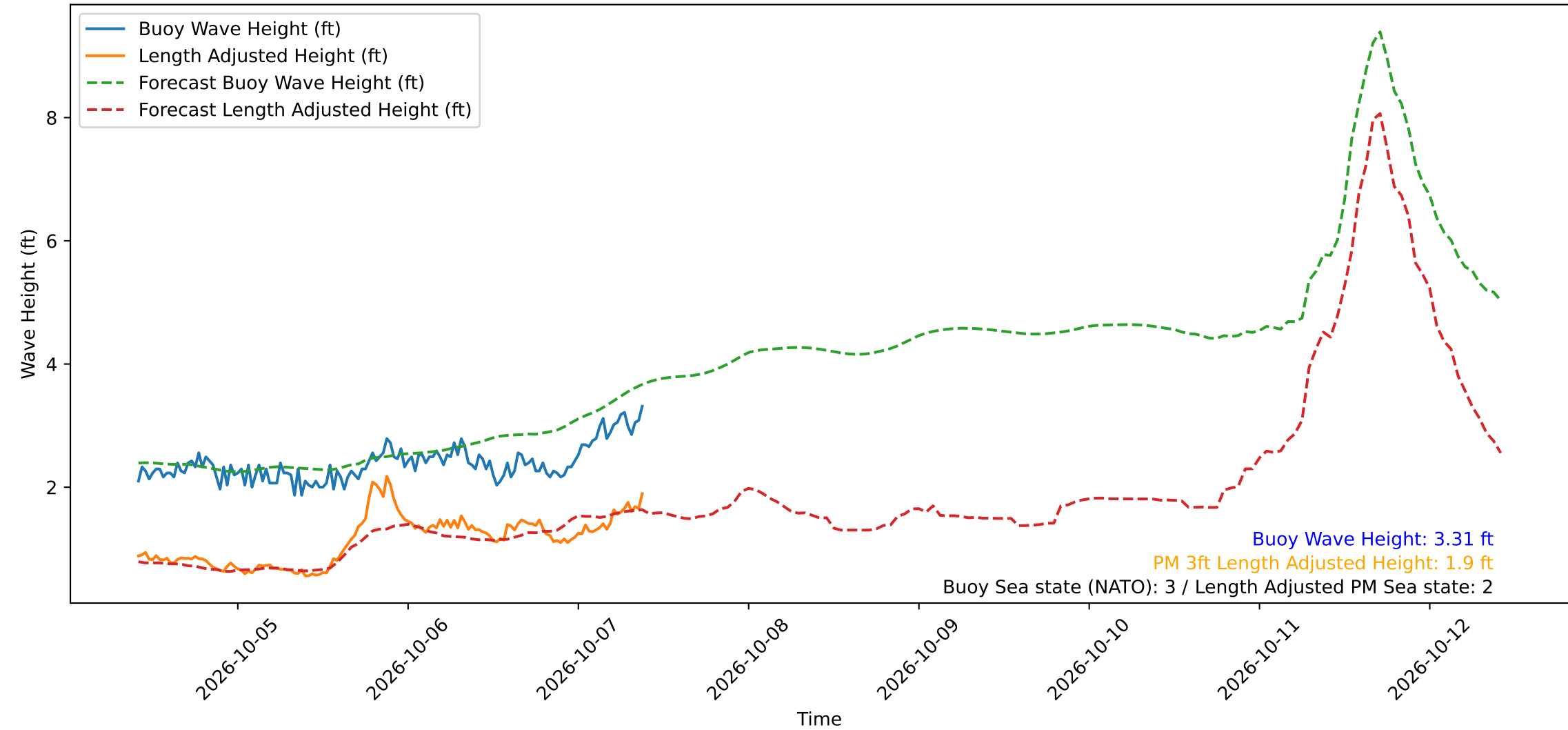
Wave Heights over Time for Oceanside Harbor at 2026-10-07 09:50:30
