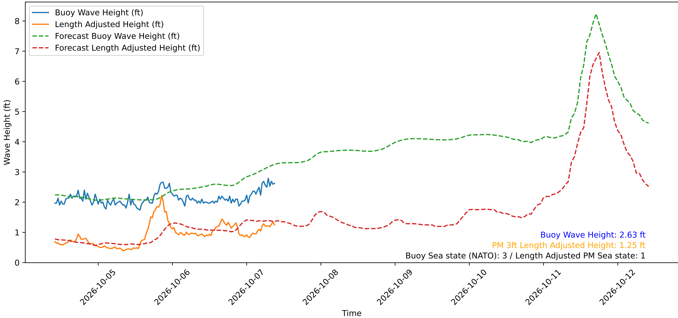
Wave Heights over Time for Red Beach at 2026-10-07 09:50:50
