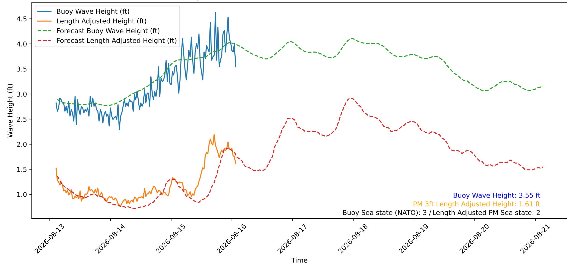
Wave Heights over Time for Oceanside Harbor at 2026-08-16 02:30:26
