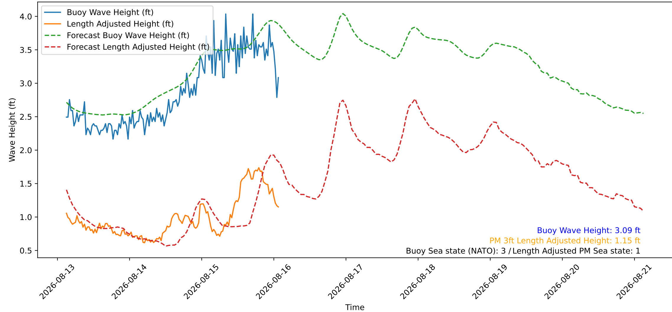
Wave Heights over Time for Red Beach at 2026-08-16 02:30:46
