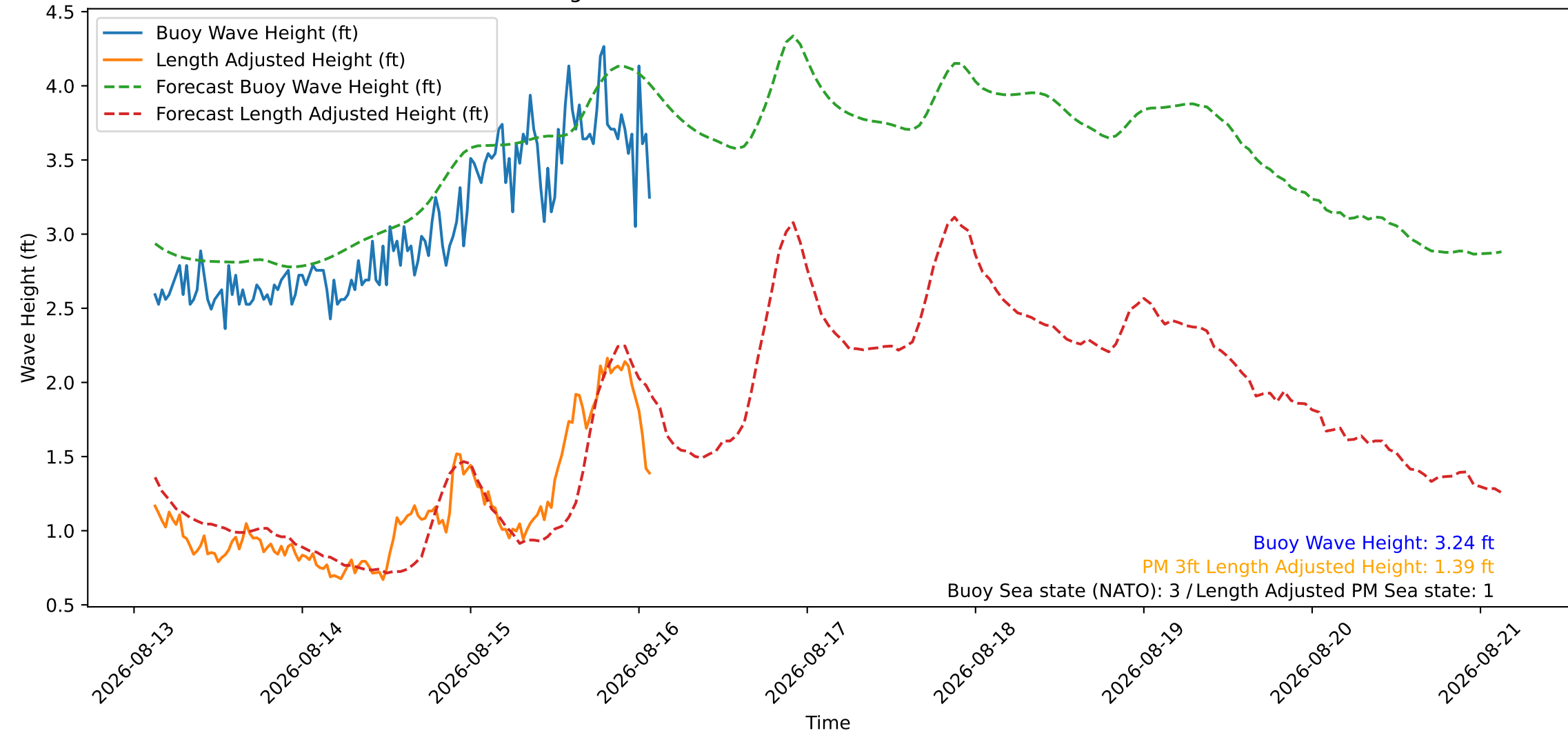
Wave Heights over Time for Green Beach at 2026-08-16 02:31:08
