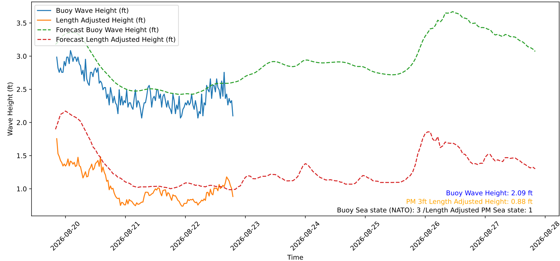
Wave Heights over Time for Red Beach at 2026-08-22 20:00:49
