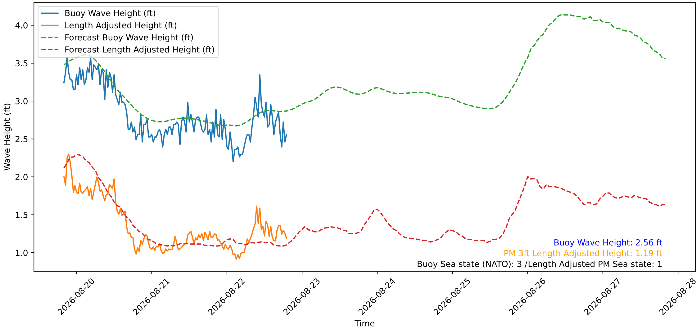
Wave Heights over Time for Oceanside Harbor at 2026-08-22 20:00:29
