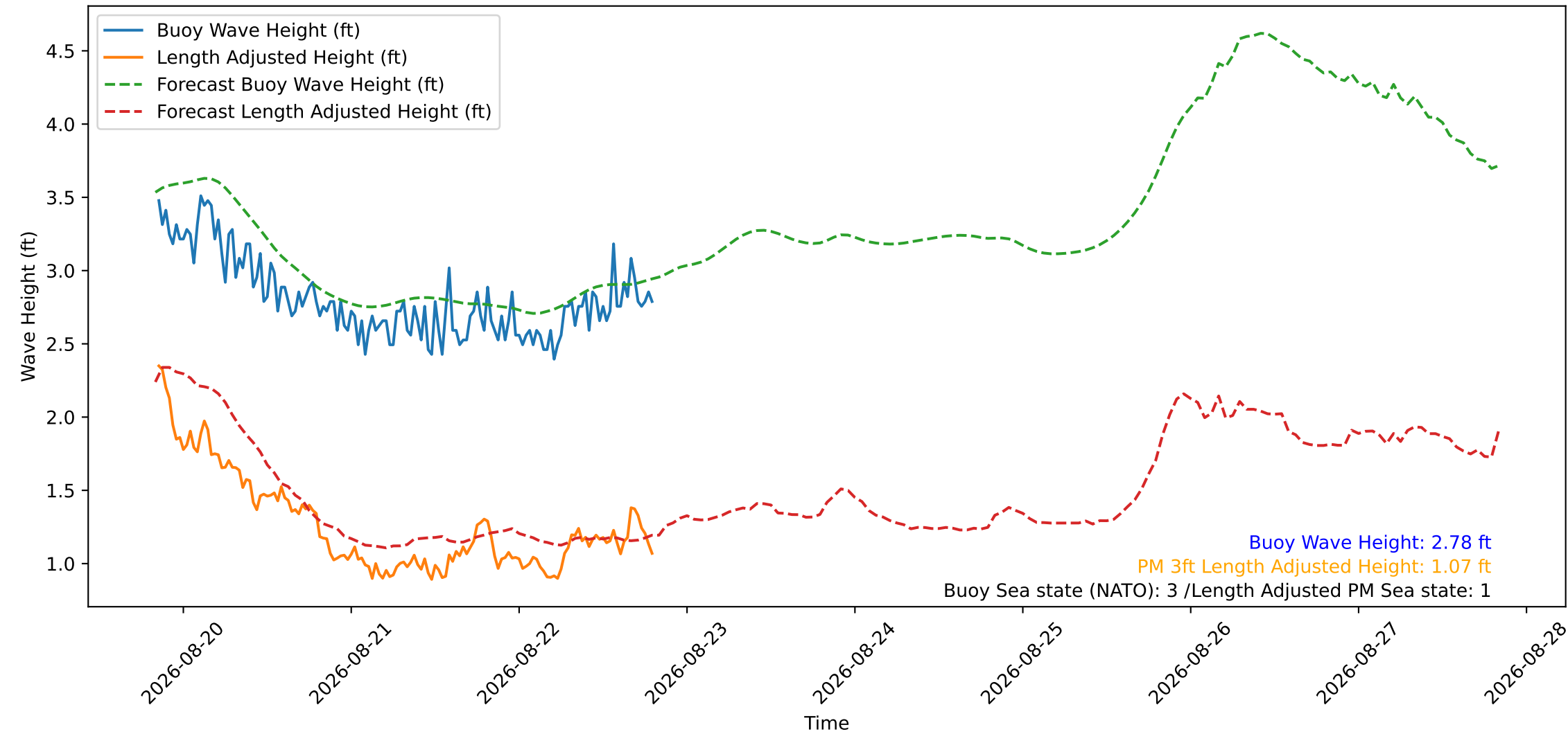
Wave Heights over Time for Green Beach at 2026-08-22 20:01:12
