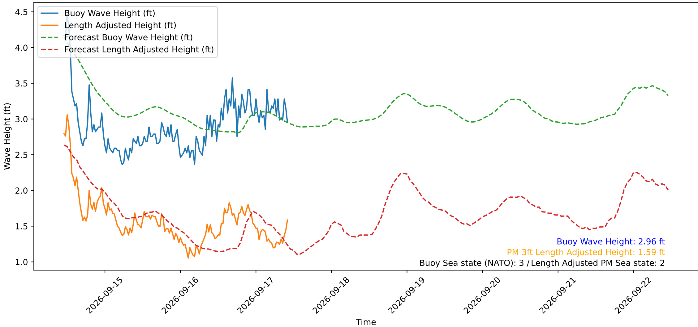
Wave Heights over Time for Oceanside Harbor at 2026-09-17 11:00:29
