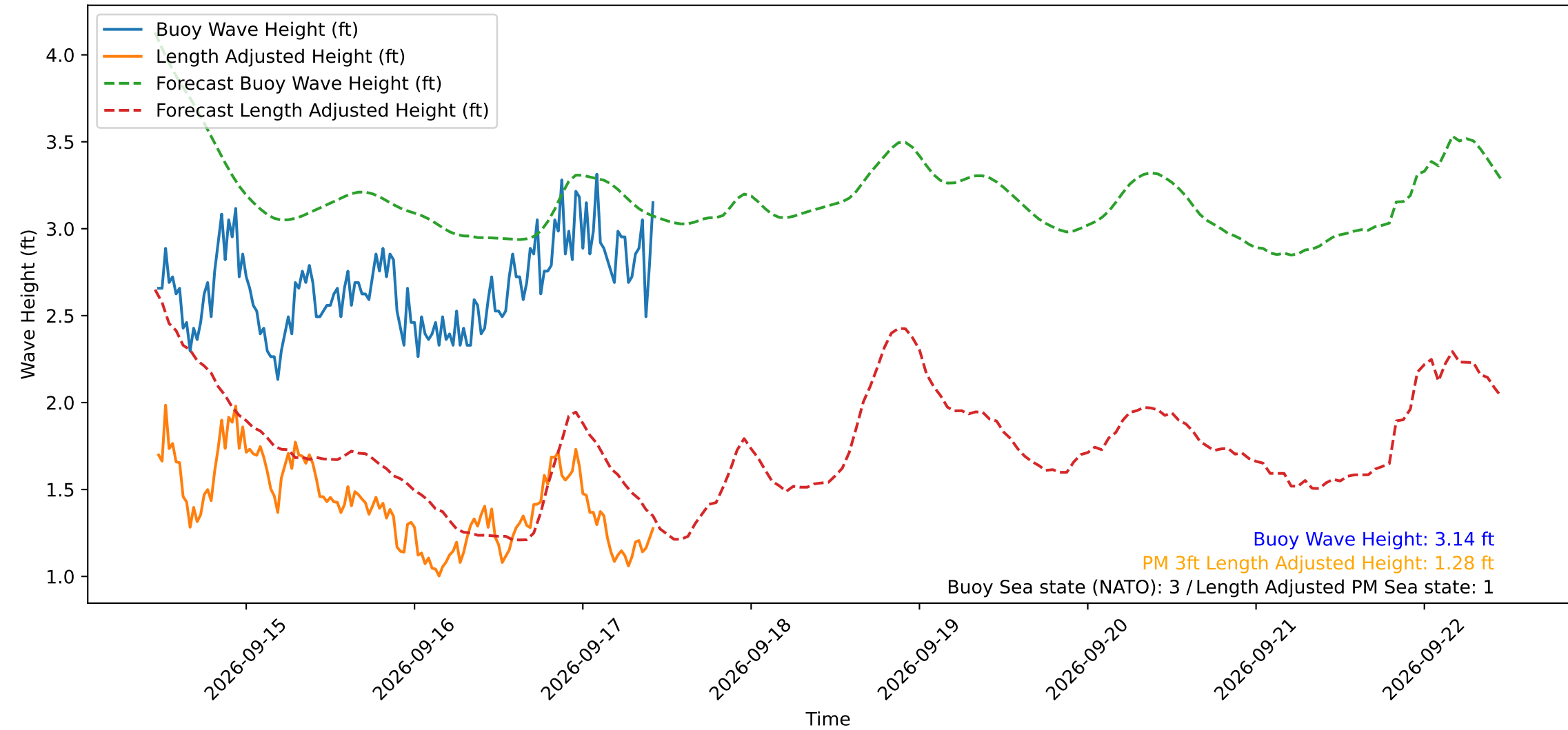
Wave Heights over Time for Green Beach at 2026-09-17 11:01:11
