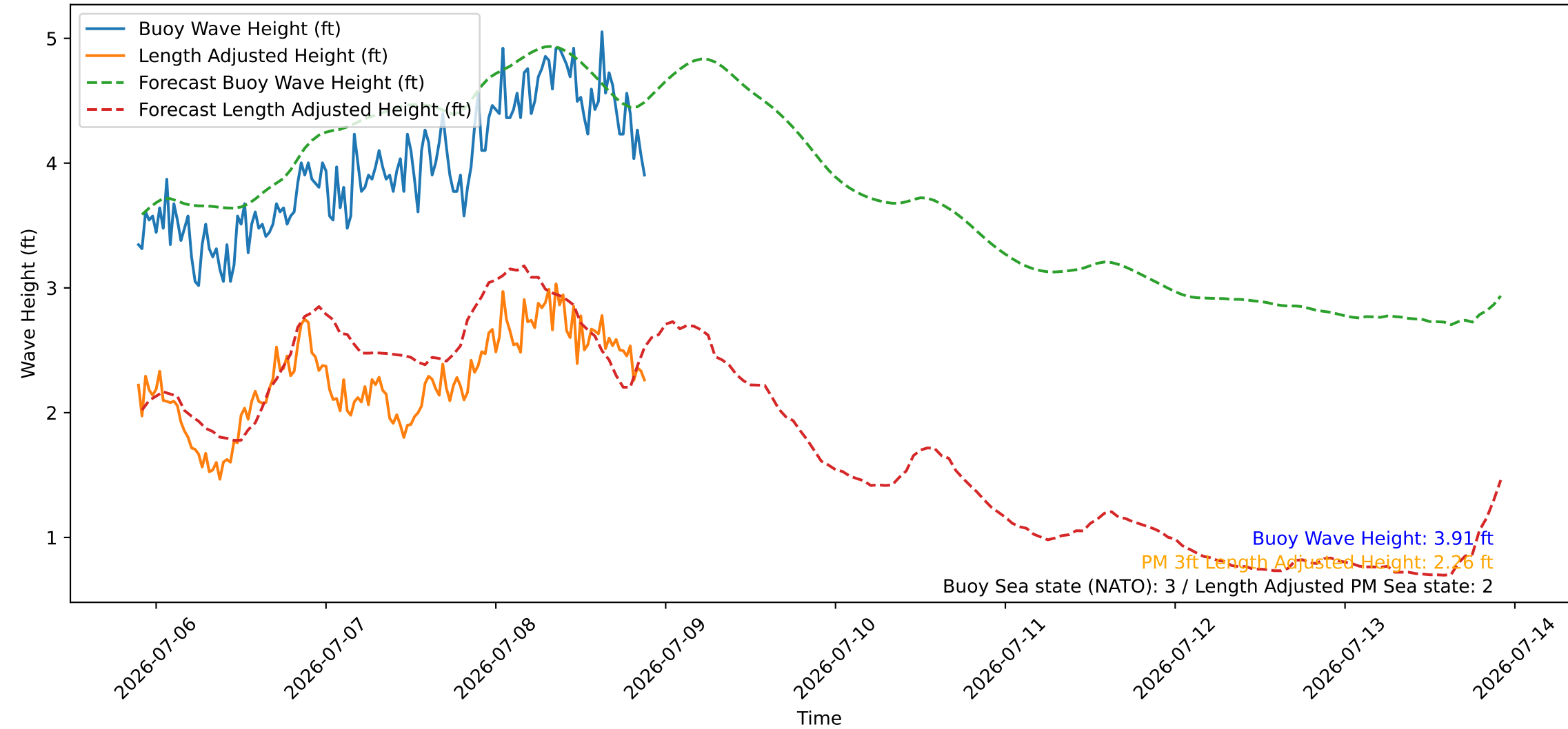
Wave Heights over Time for Oceanside Harbor at 2026-07-08 21:40:26
