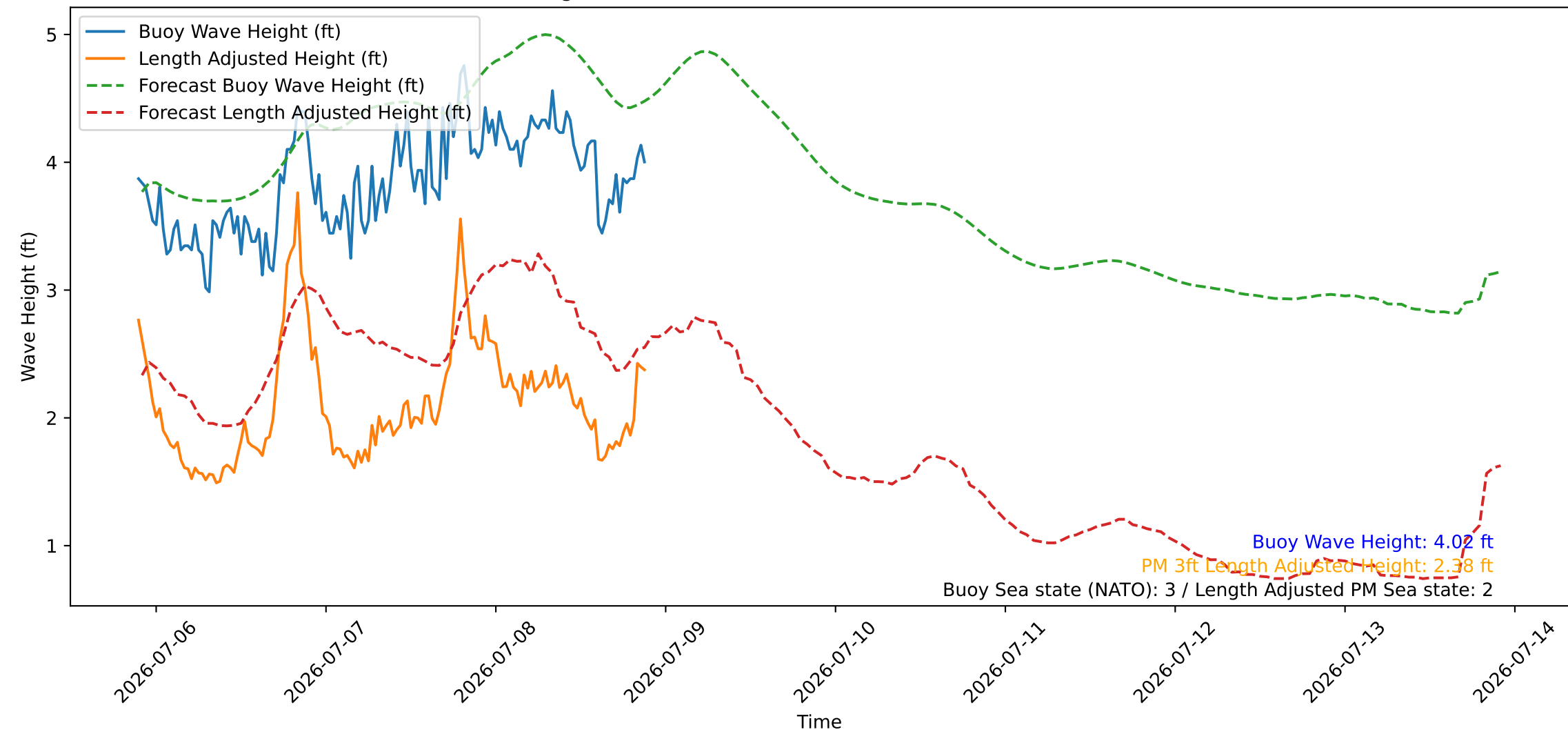
Wave Heights over Time for Green Beach at 2026-07-08 21:41:07
