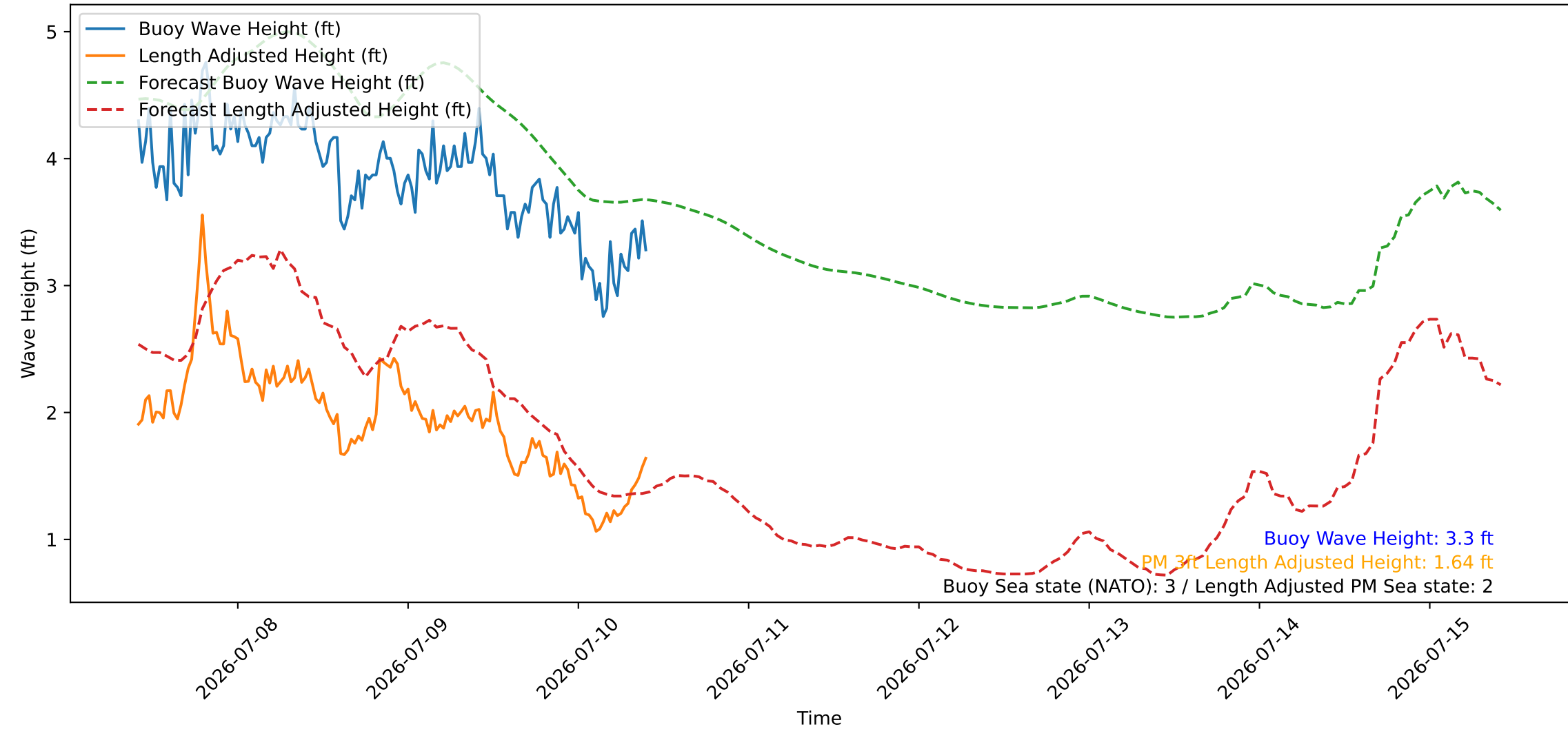
Wave Heights over Time for Green Beach at 2026-07-10 10:11:07
