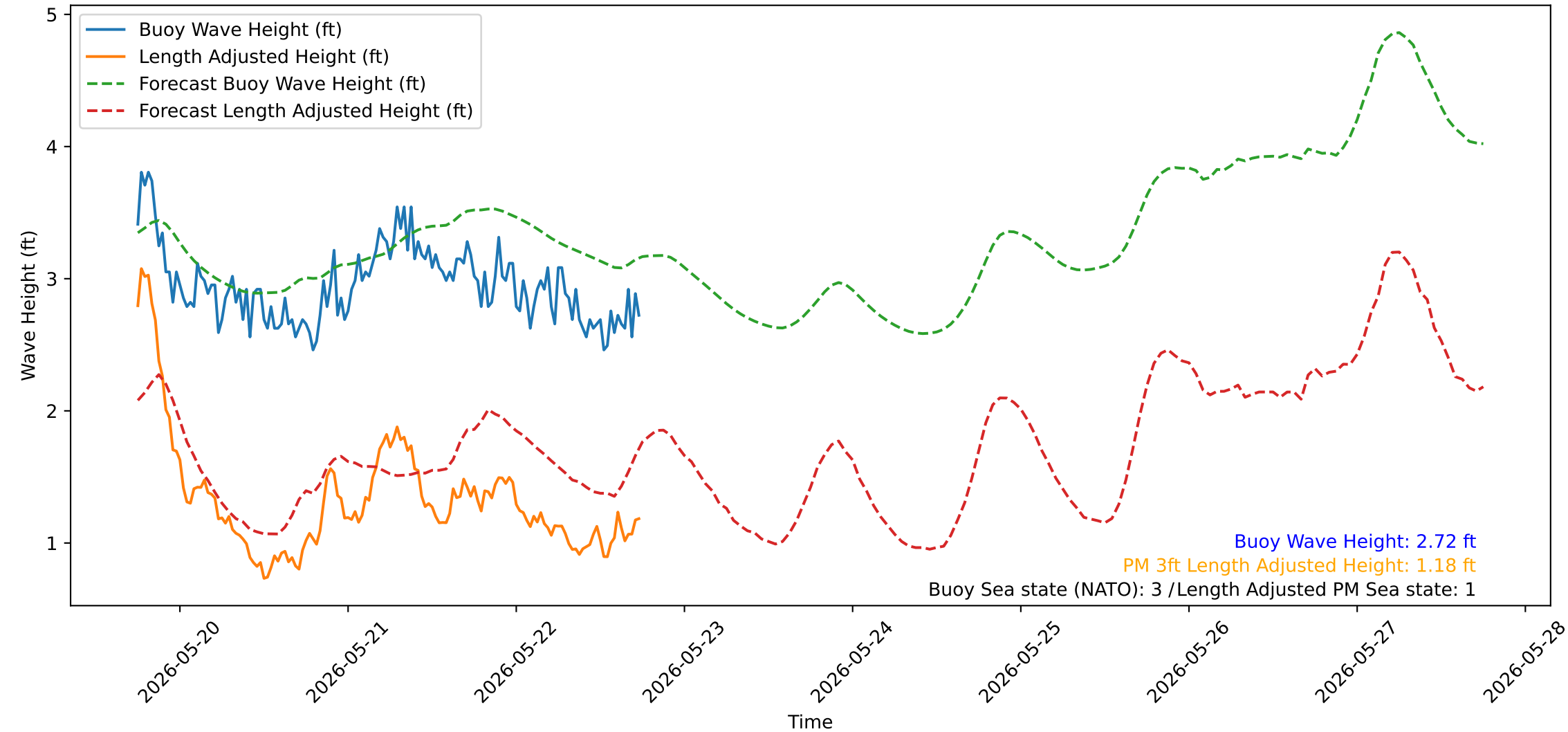
Wave Heights over Time for Green Beach at 2026-05-22 18:11:14
