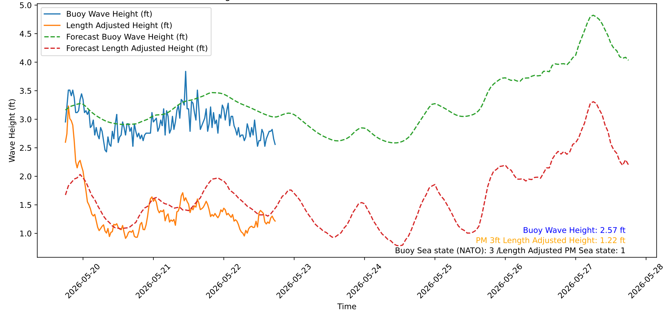
Wave Heights over Time for Oceanside Harbor at 2026-05-22 18:10:31
