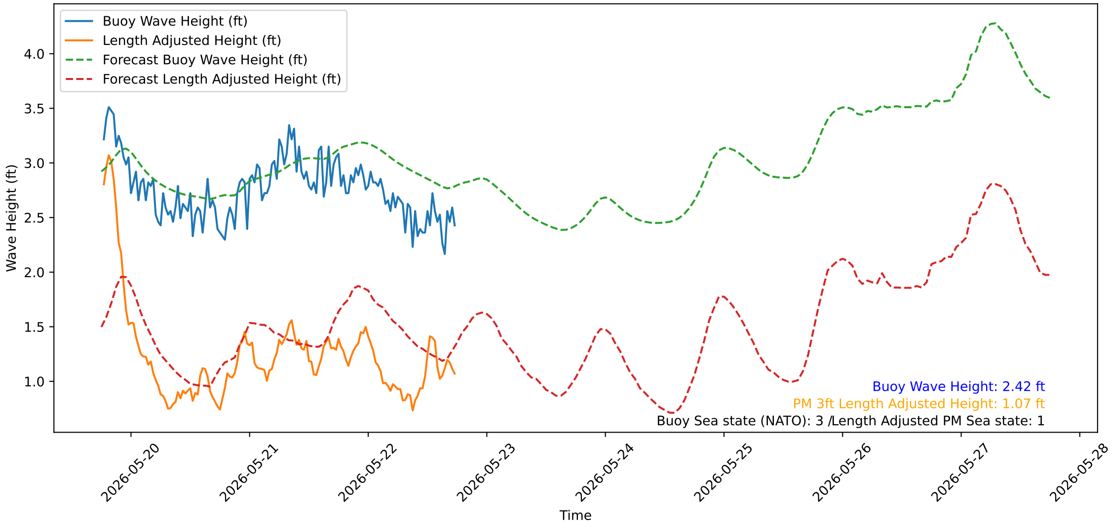
Wave Heights over Time for Red Beach at 2026-05-22 18:10:51
