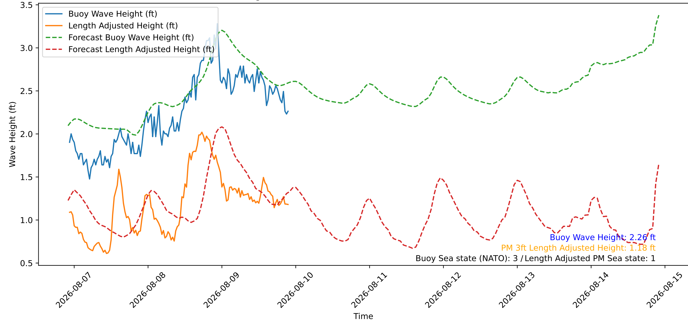
Wave Heights over Time for Red Beach at 2026-08-09 22:10:45
