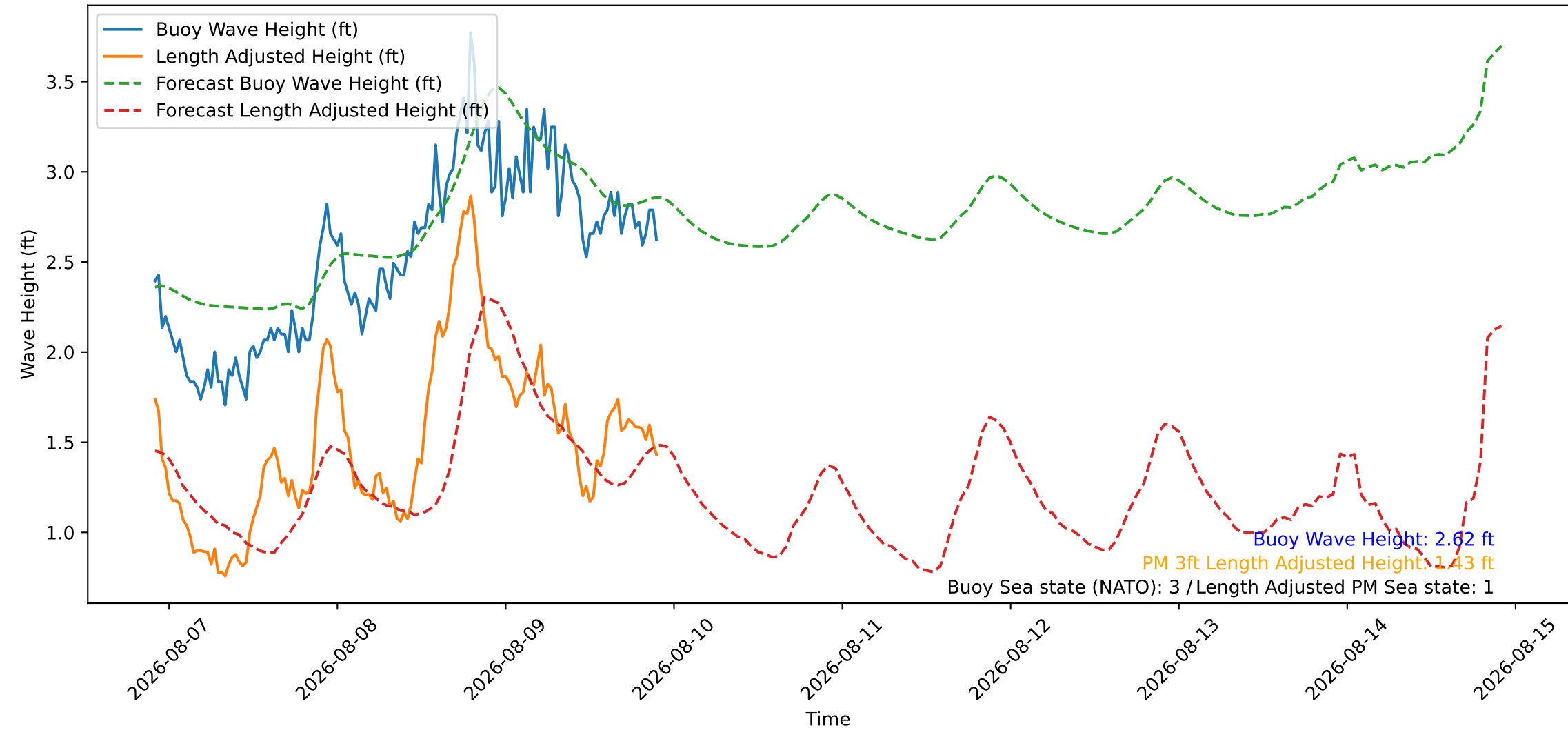
Wave Heights over Time for Green Beach at 2026-08-09 22:11:08
