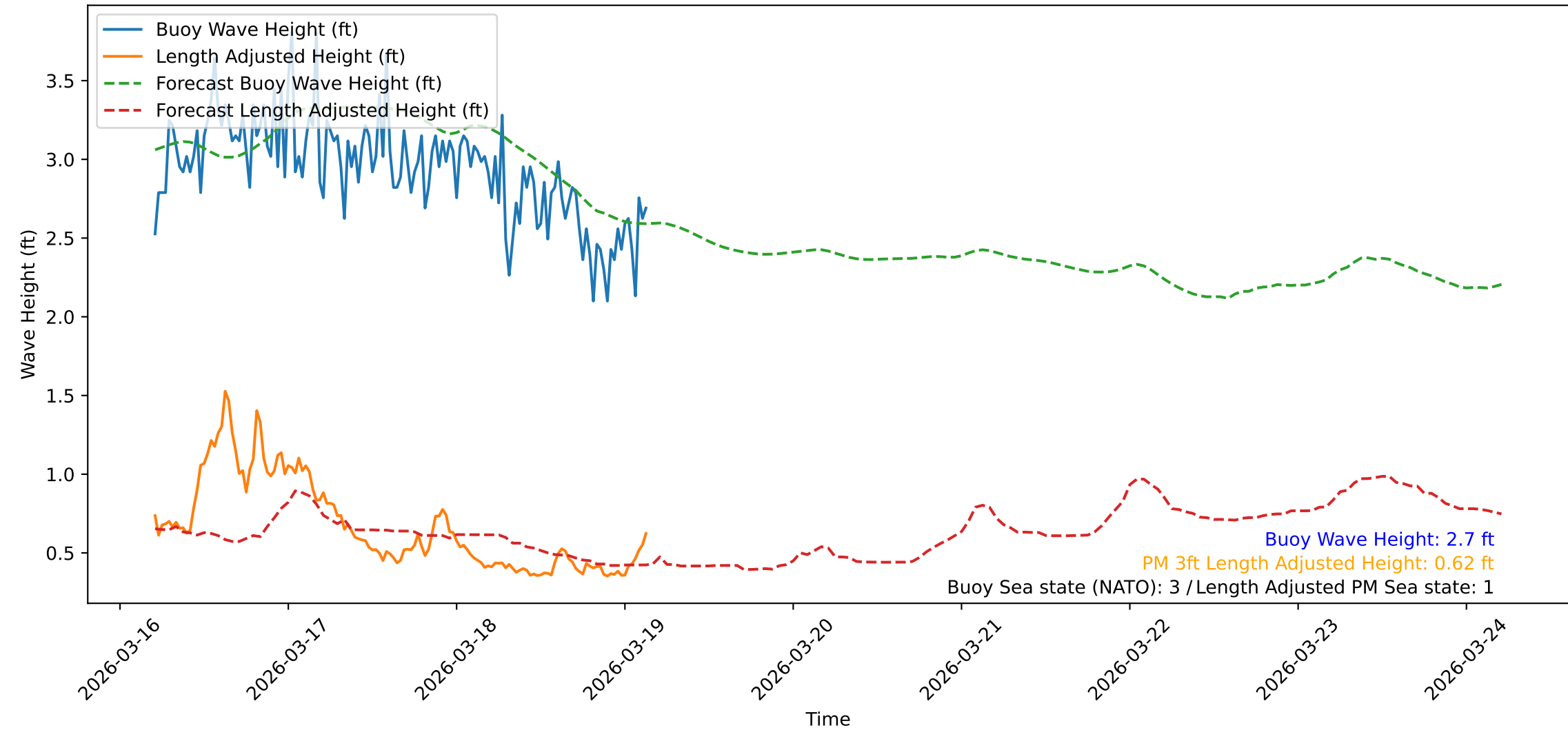
Wave Heights over Time for Red Beach at 2026-03-19 04:30:48
