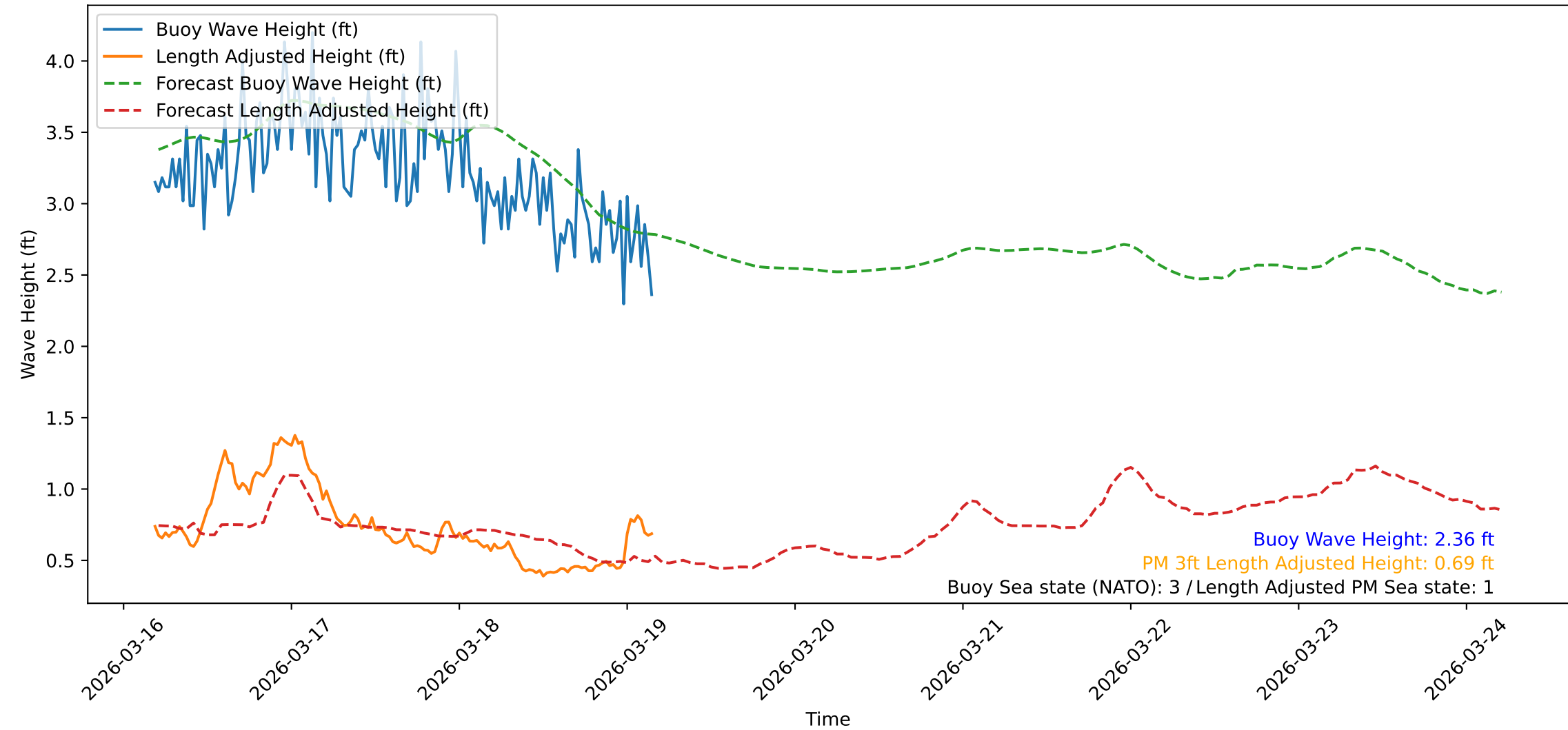
Wave Heights over Time for Green Beach at 2026-03-19 04:31:10
