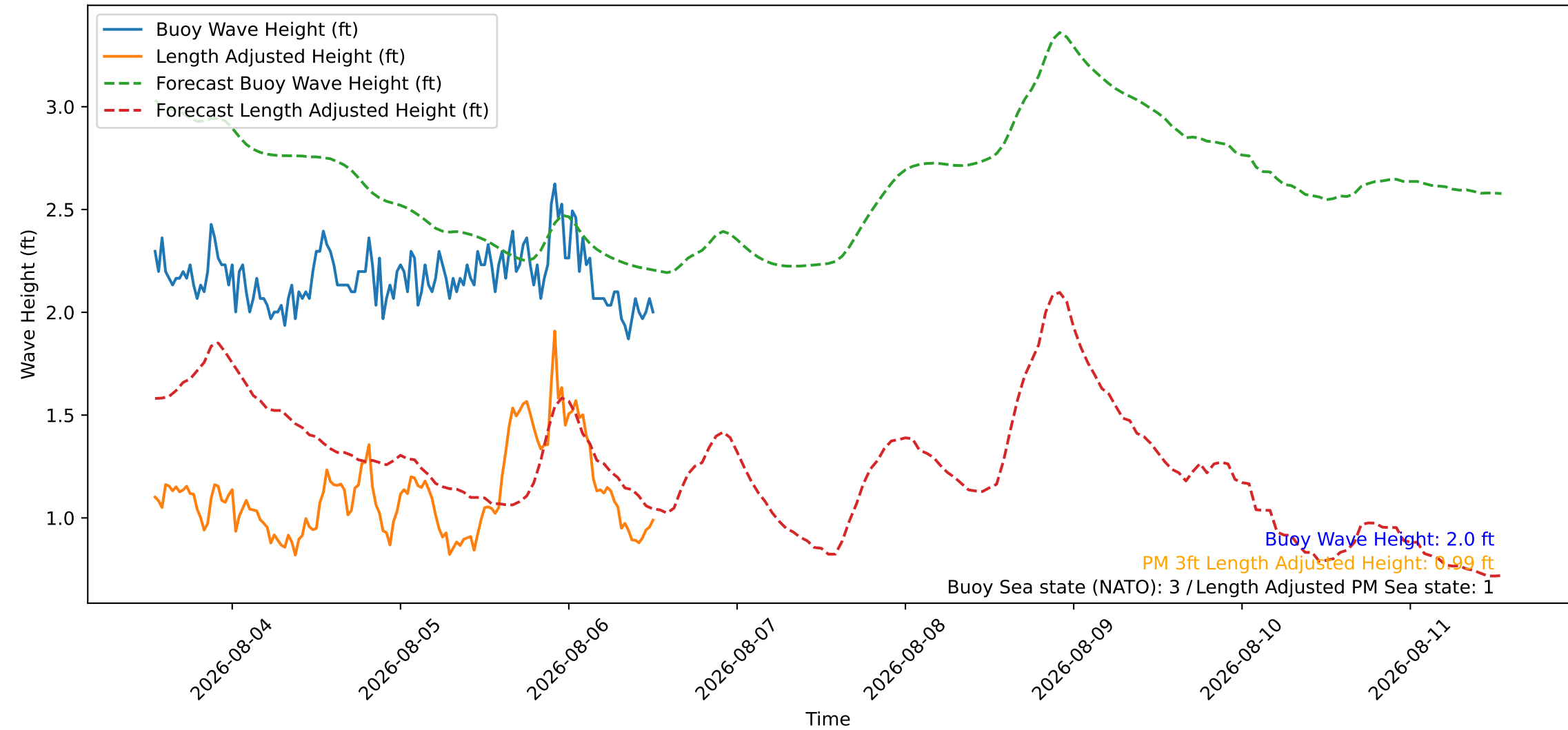
Wave Heights over Time for Green Beach at 2026-08-06 13:01:07
