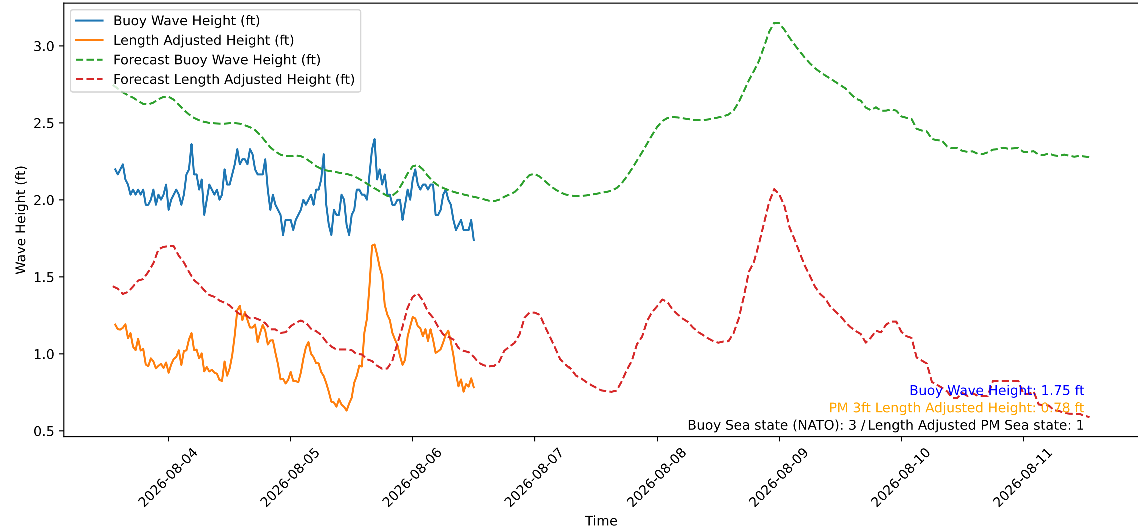
Wave Heights over Time for Red Beach at 2026-08-06 13:00:45
