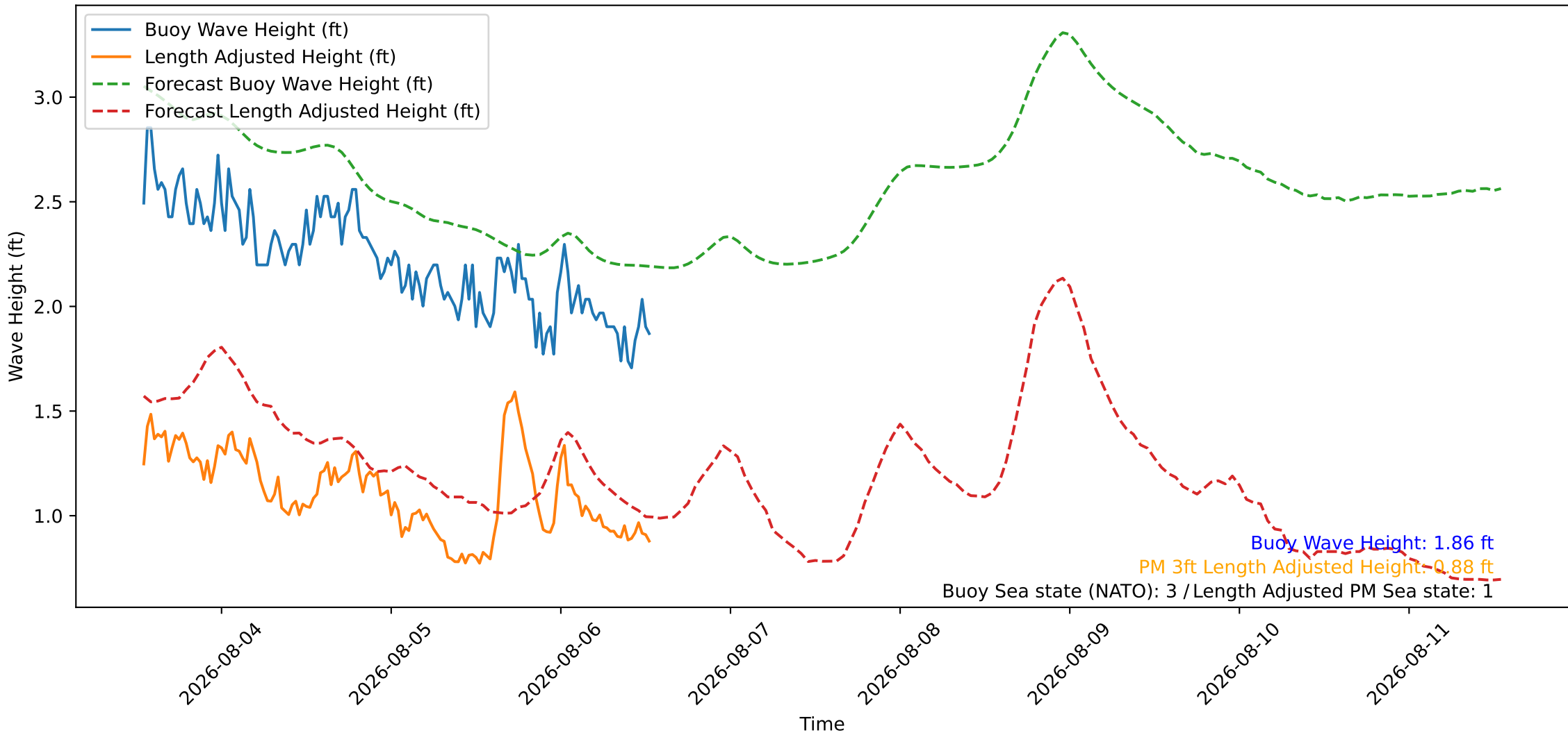
Wave Heights over Time for Oceanside Harbor at 2026-08-06 13:00:26
