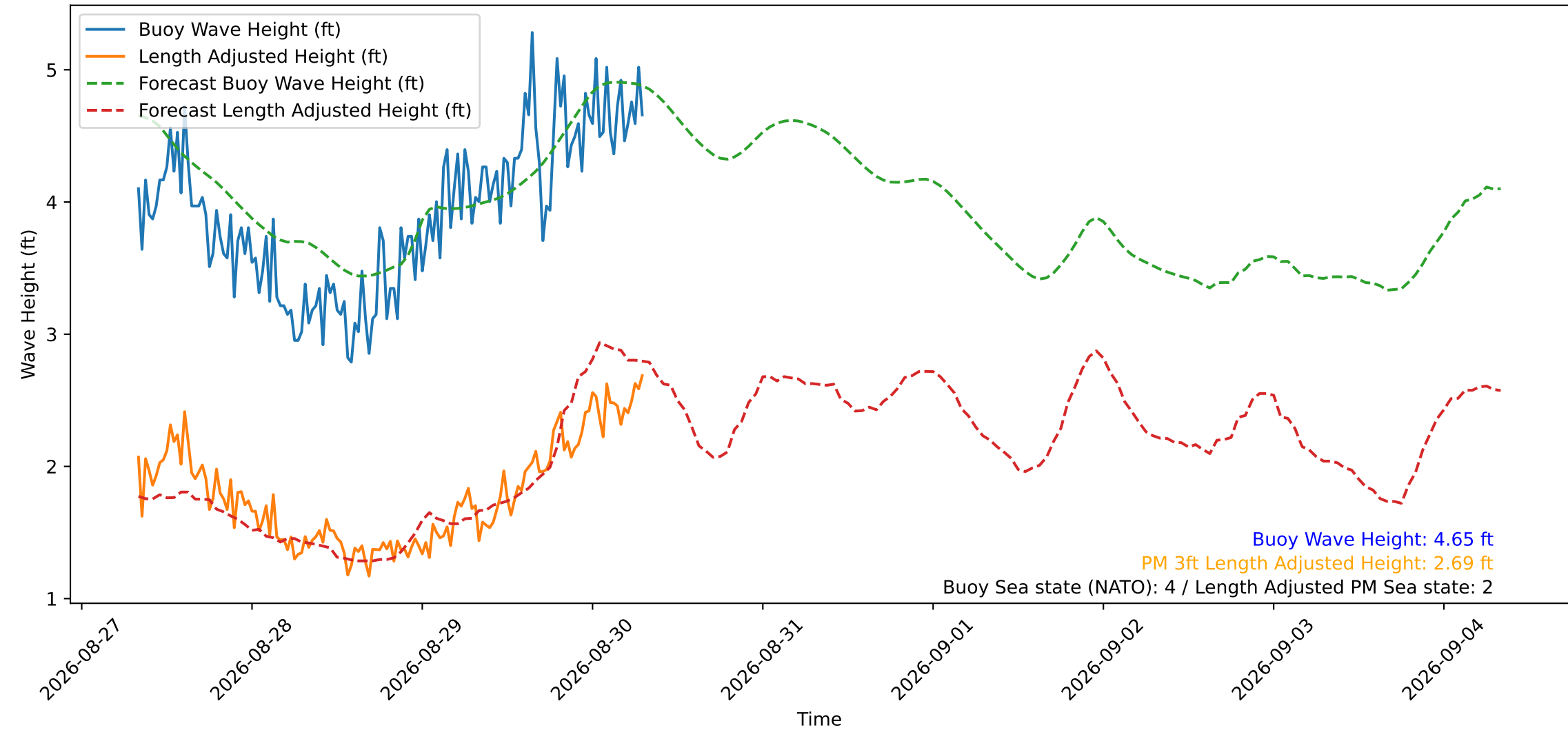
Wave Heights over Time for Oceanside Harbor at 2026-08-30 08:00:30
