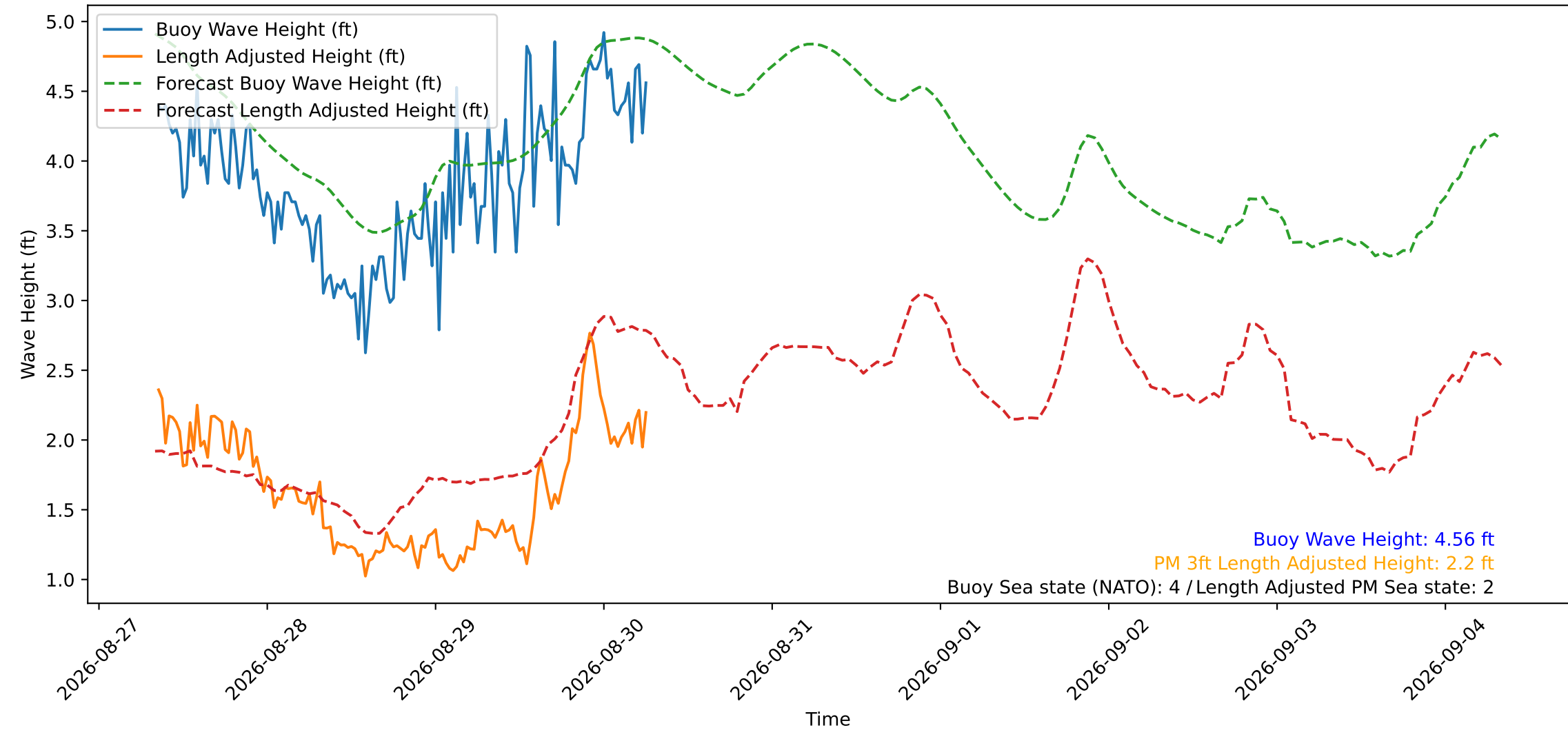
Wave Heights over Time for Green Beach at 2026-08-30 08:01:13
