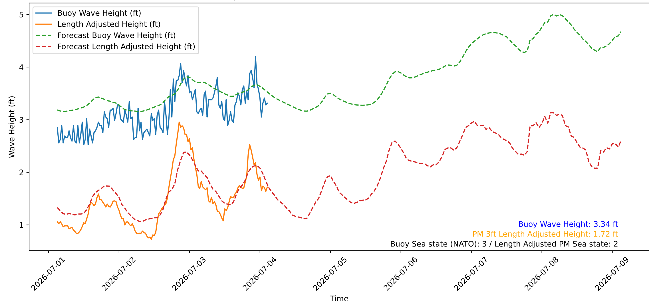
Wave Heights over Time for Green Beach at 2026-07-04 03:11:08
