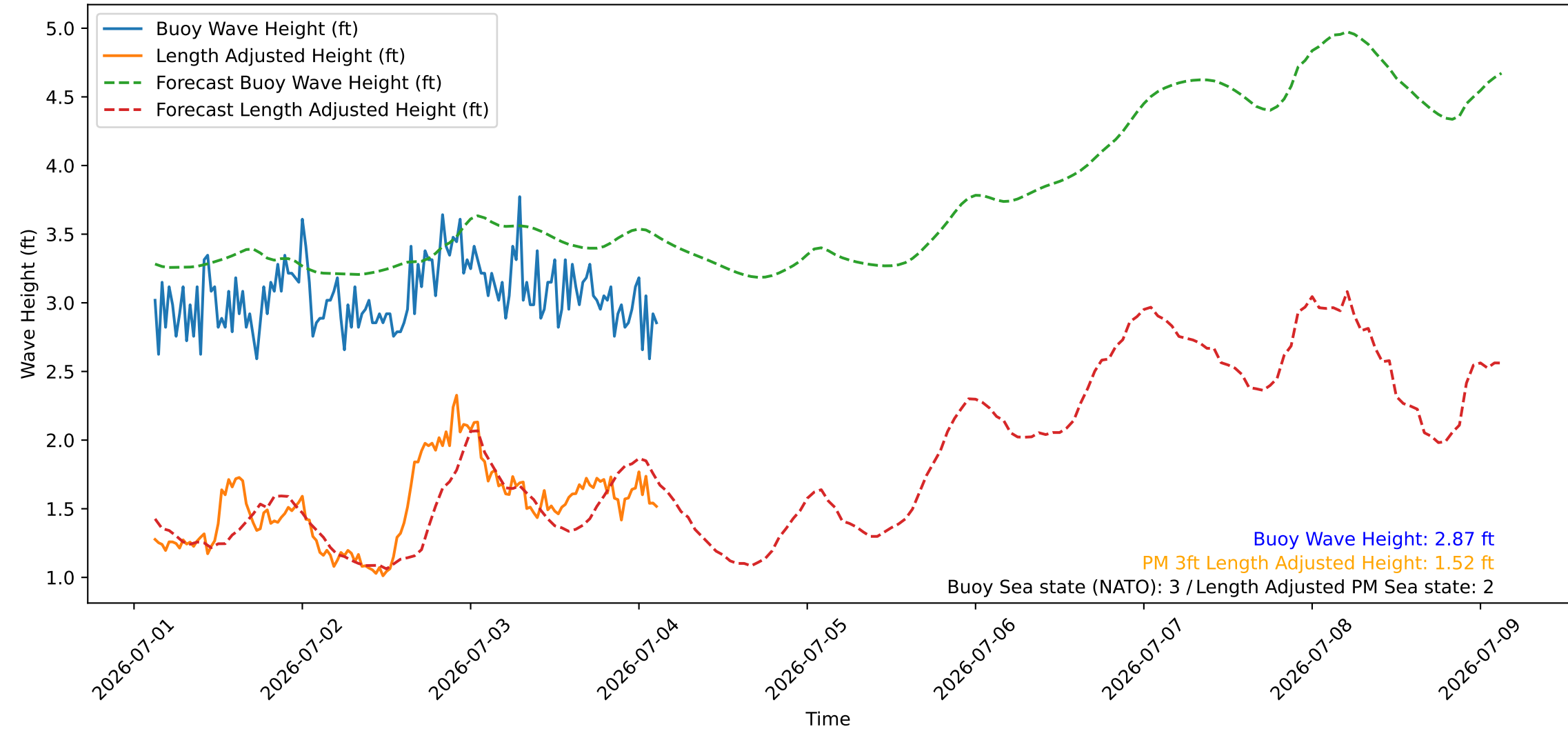
Wave Heights over Time for Oceanside Harbor at 2026-07-04 03:10:26
