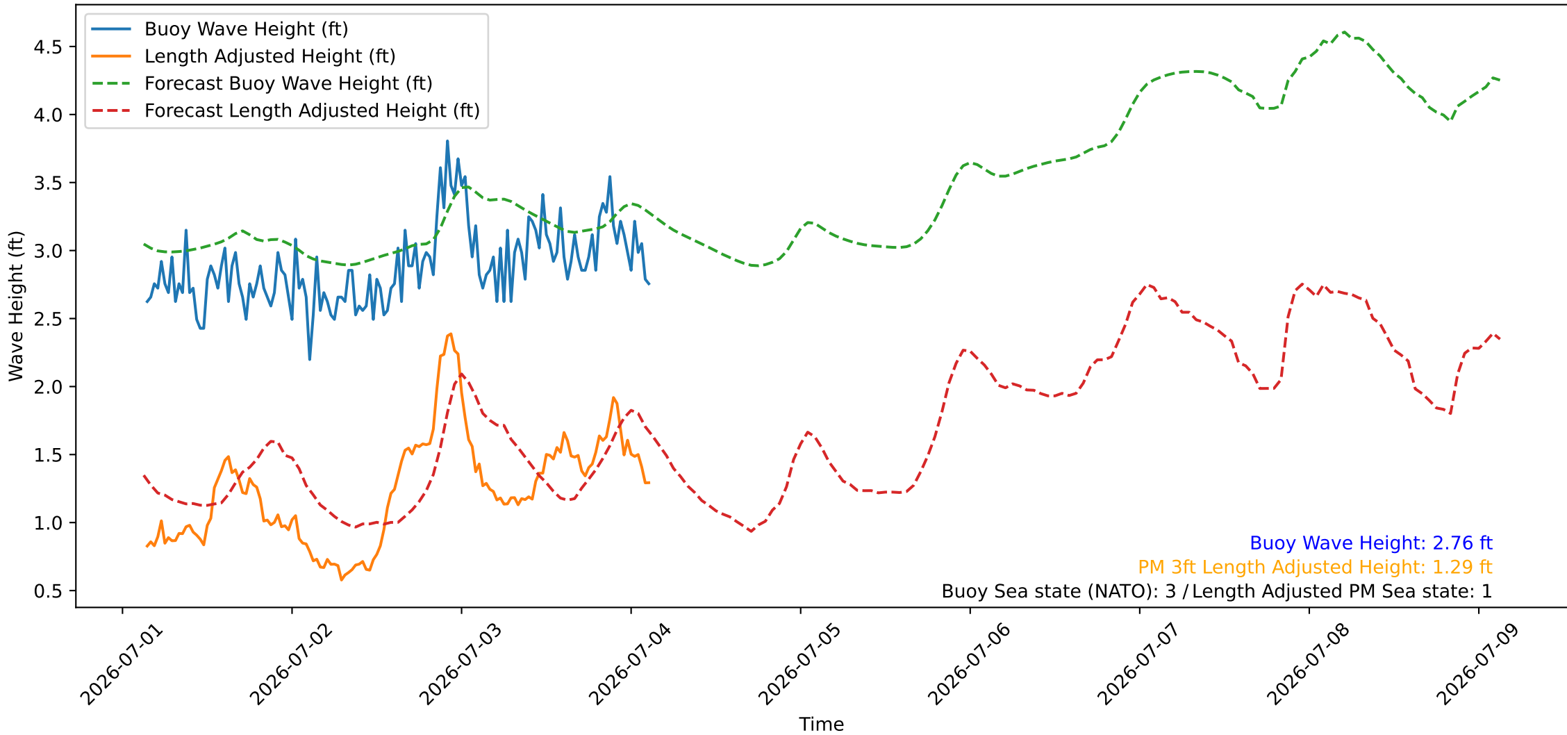
Wave Heights over Time for Red Beach at 2026-07-04 03:10:45
