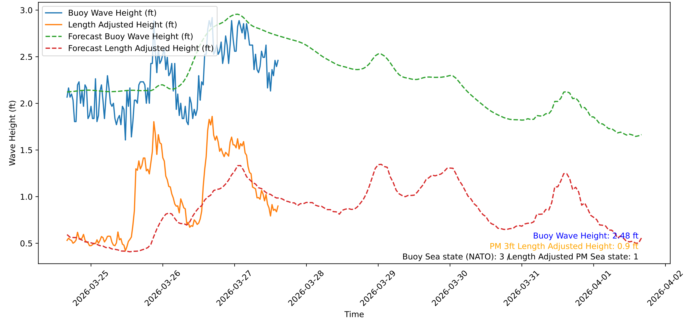
Wave Heights over Time for Oceanside Harbor at 2026-03-27 15:50:31
