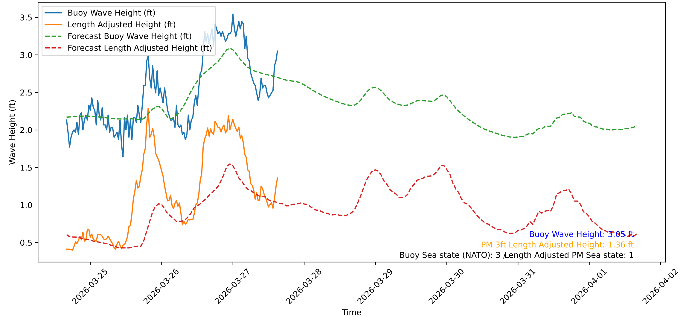
Wave Heights over Time for Green Beach at 2026-03-27 15:51:09
