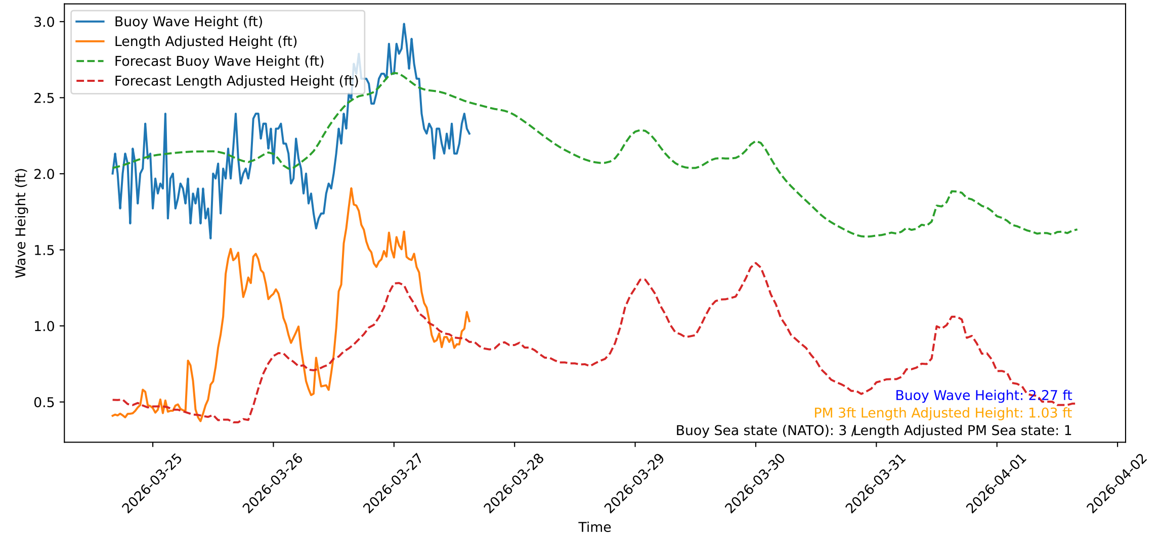
Wave Heights over Time for Red Beach at 2026-03-27 15:50:47
