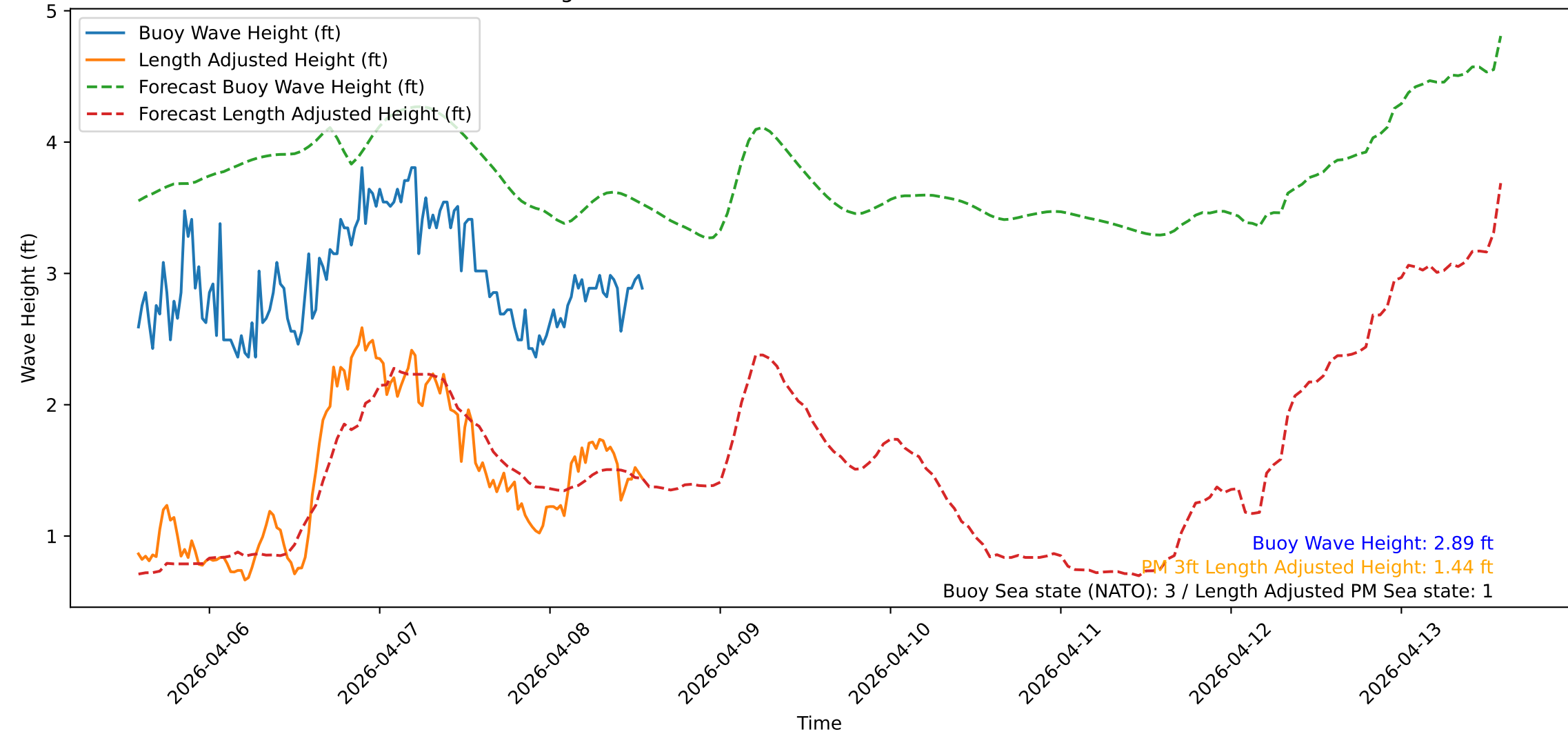
Wave Heights over Time for Green Beach at 2026-04-08 14:01:09
