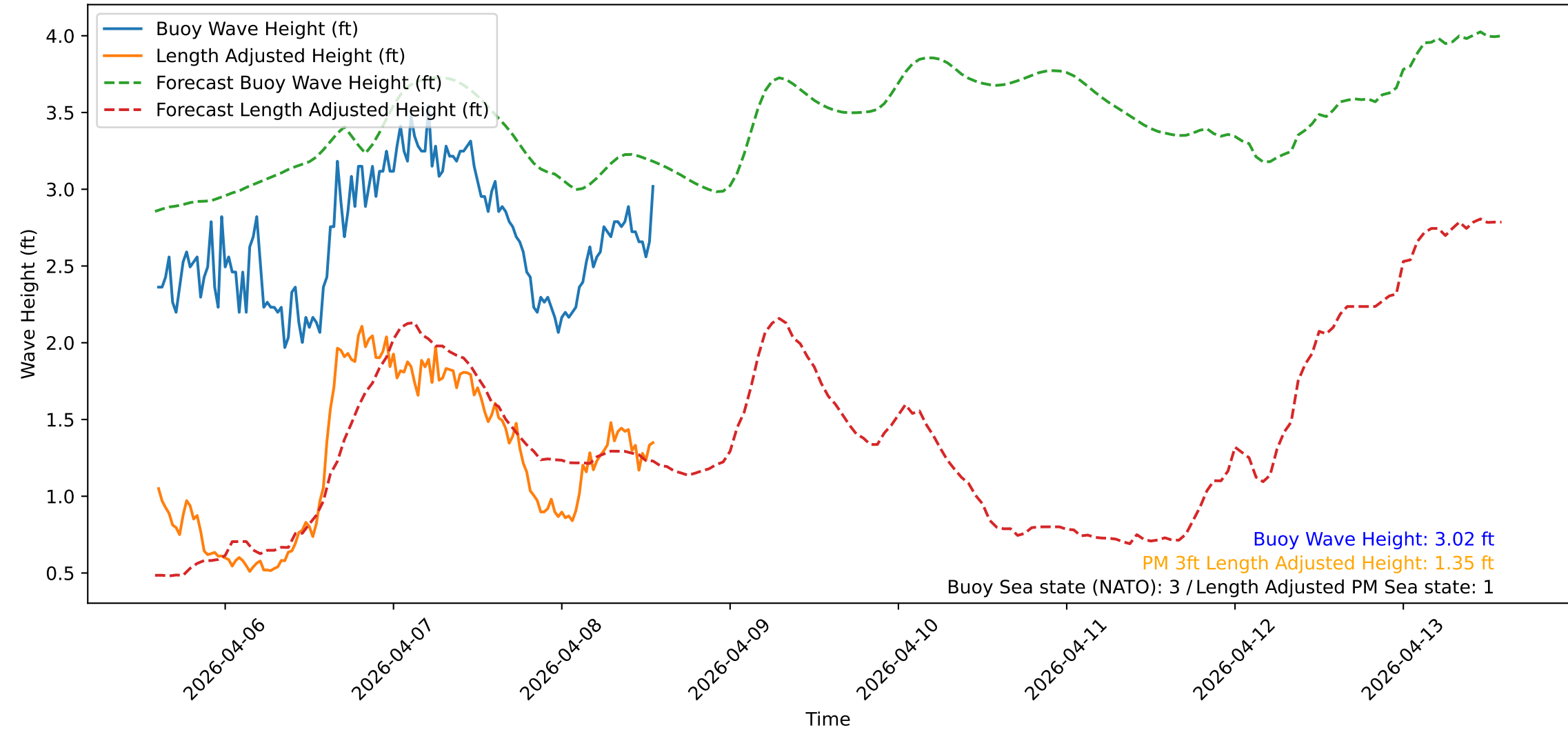
Wave Heights over Time for Red Beach at 2026-04-08 14:00:47
