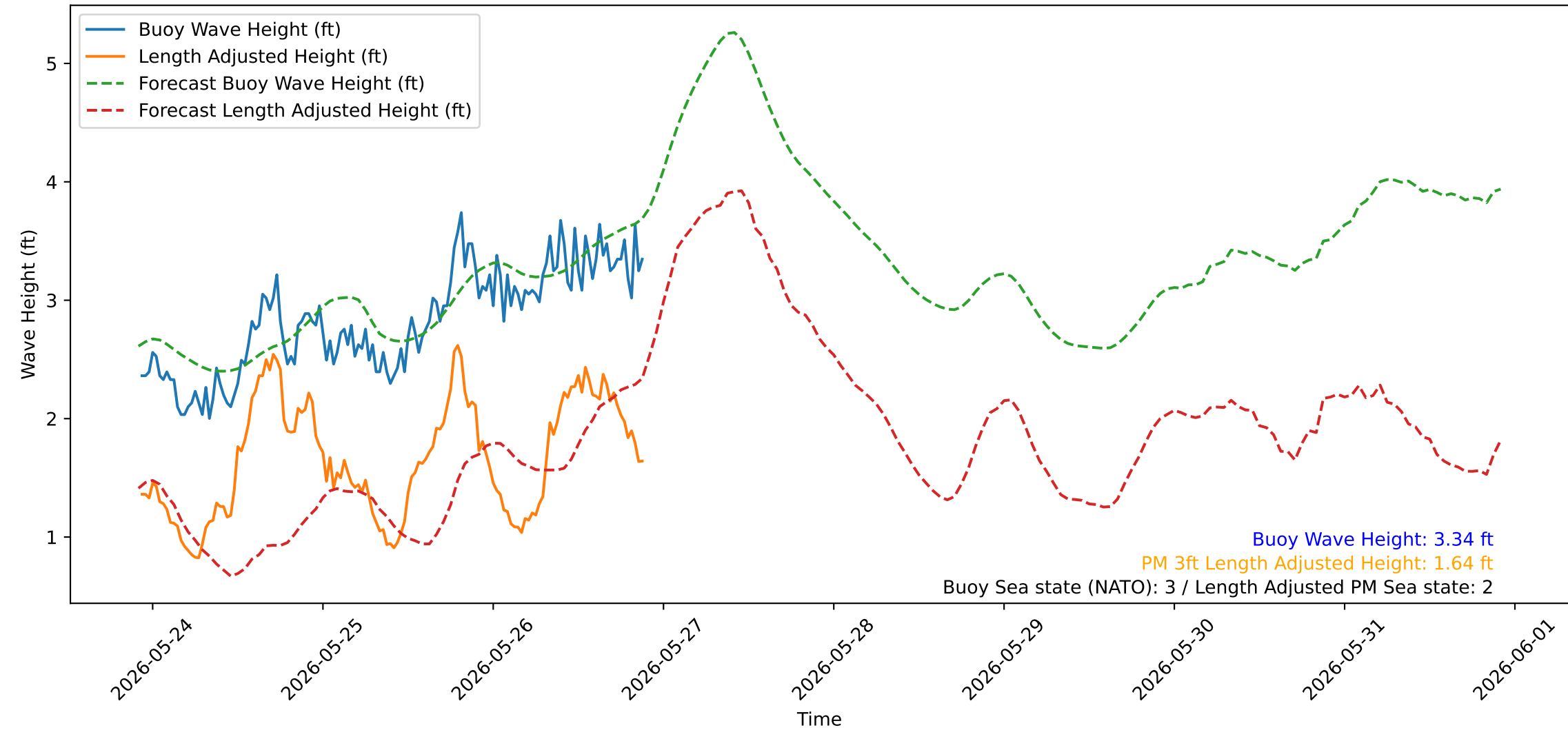
Wave Heights over Time for Red Beach at 2026-05-26 22:00:47
