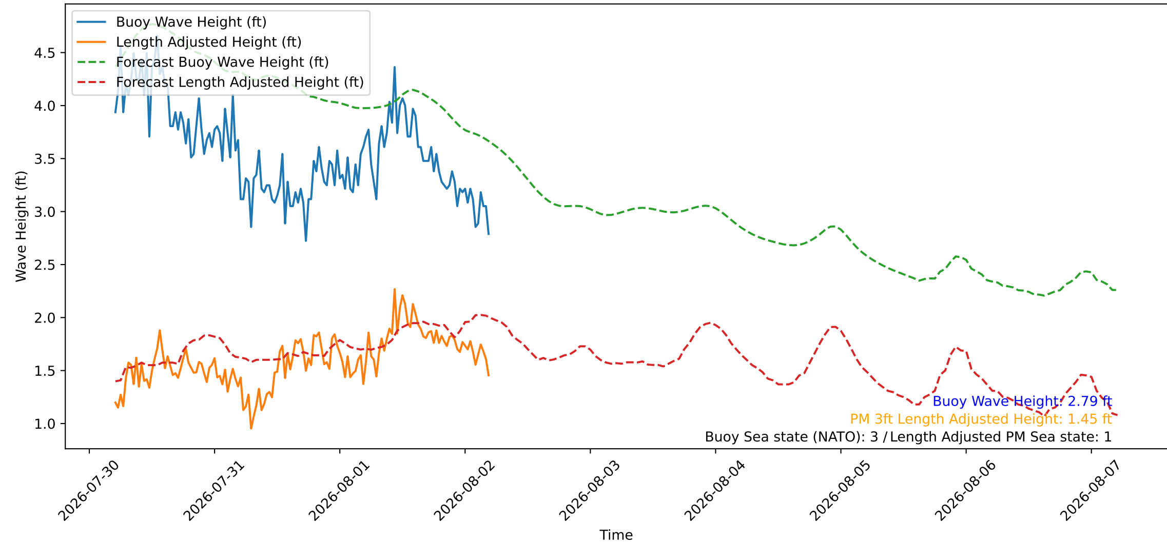
Wave Heights over Time for Oceanside Harbor at 2026-08-02 05:00:26
