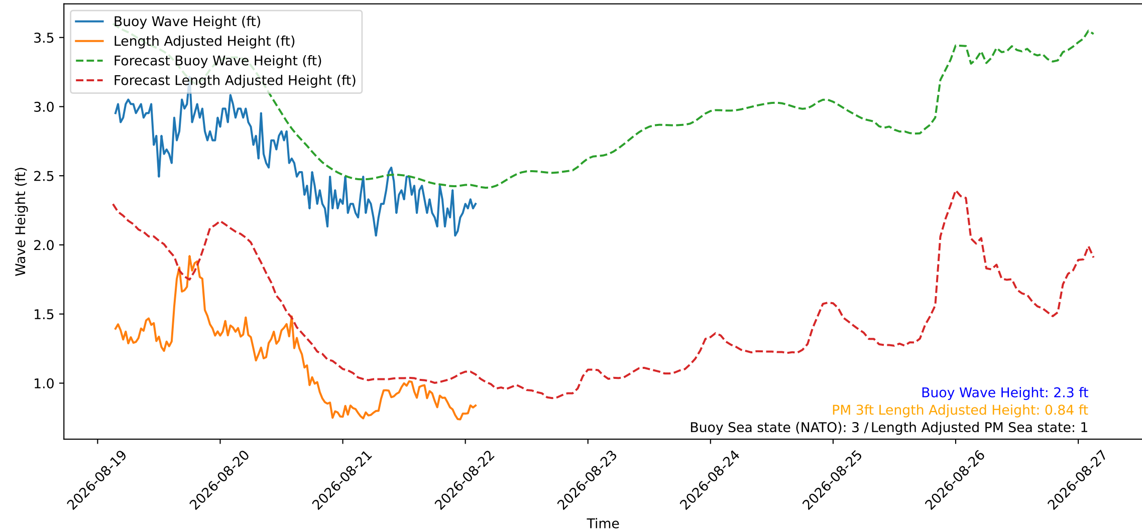
Wave Heights over Time for Red Beach at 2026-08-22 03:00:48
