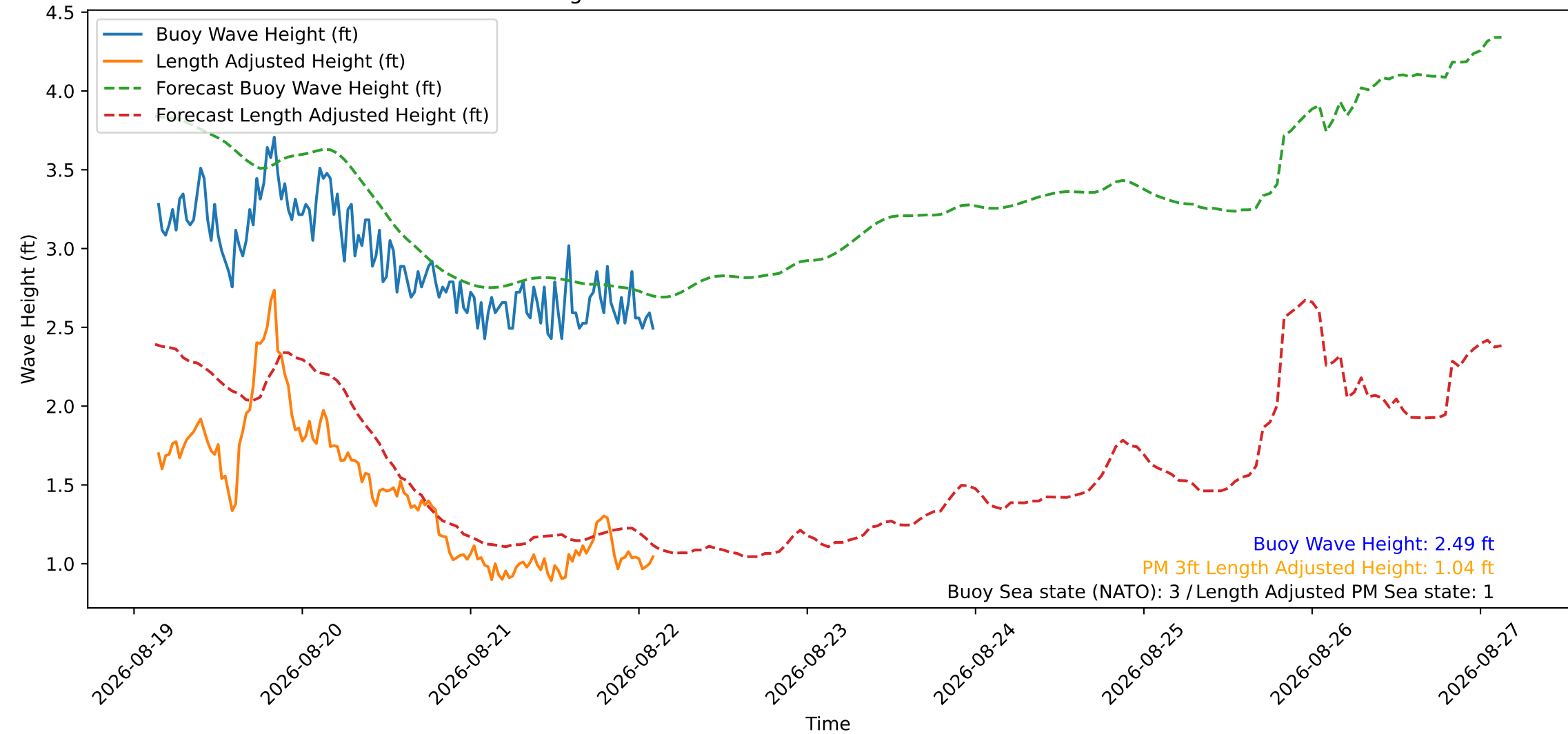
Wave Heights over Time for Green Beach at 2026-08-22 03:01:11
