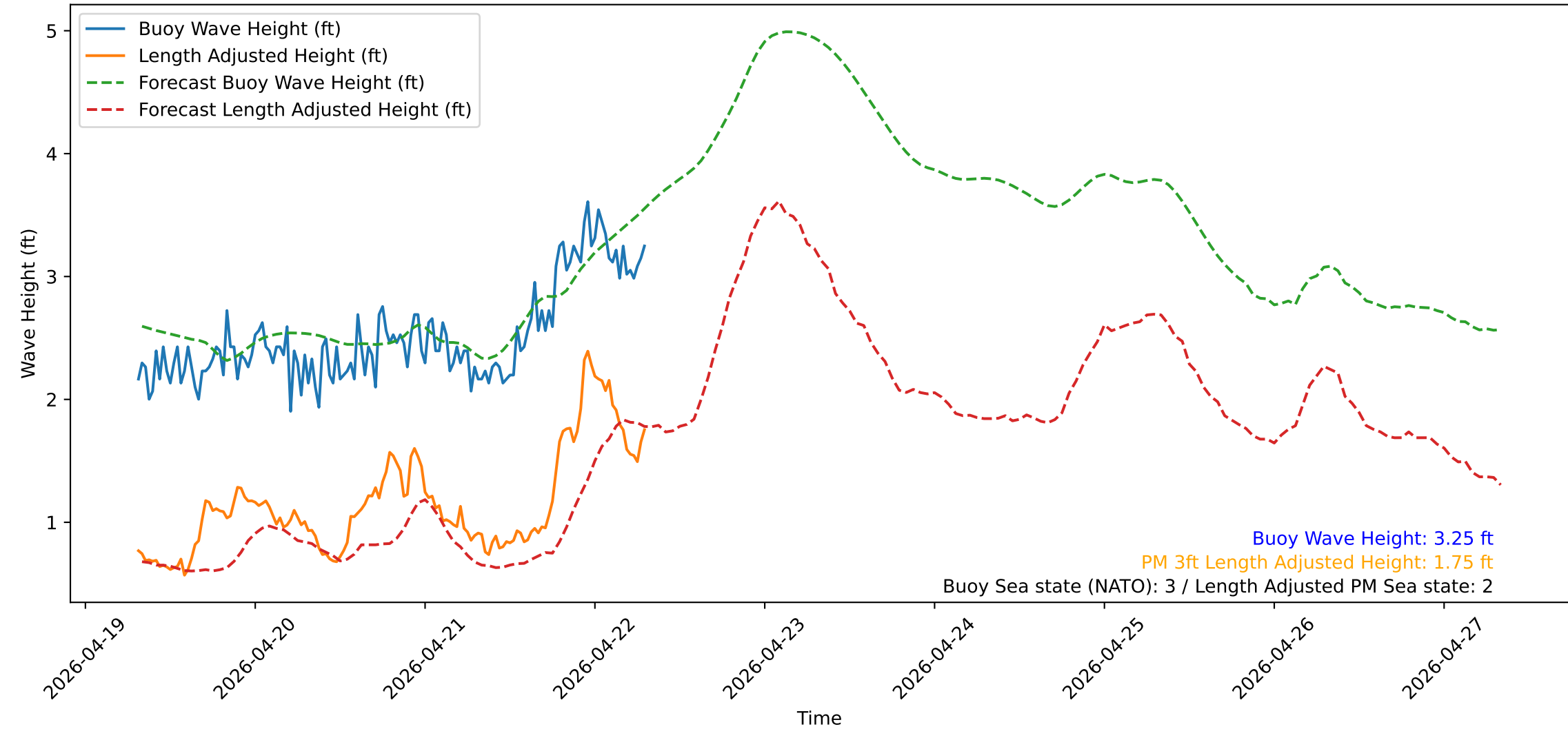
Wave Heights over Time for Oceanside Harbor at 2026-04-22 07:40:31
