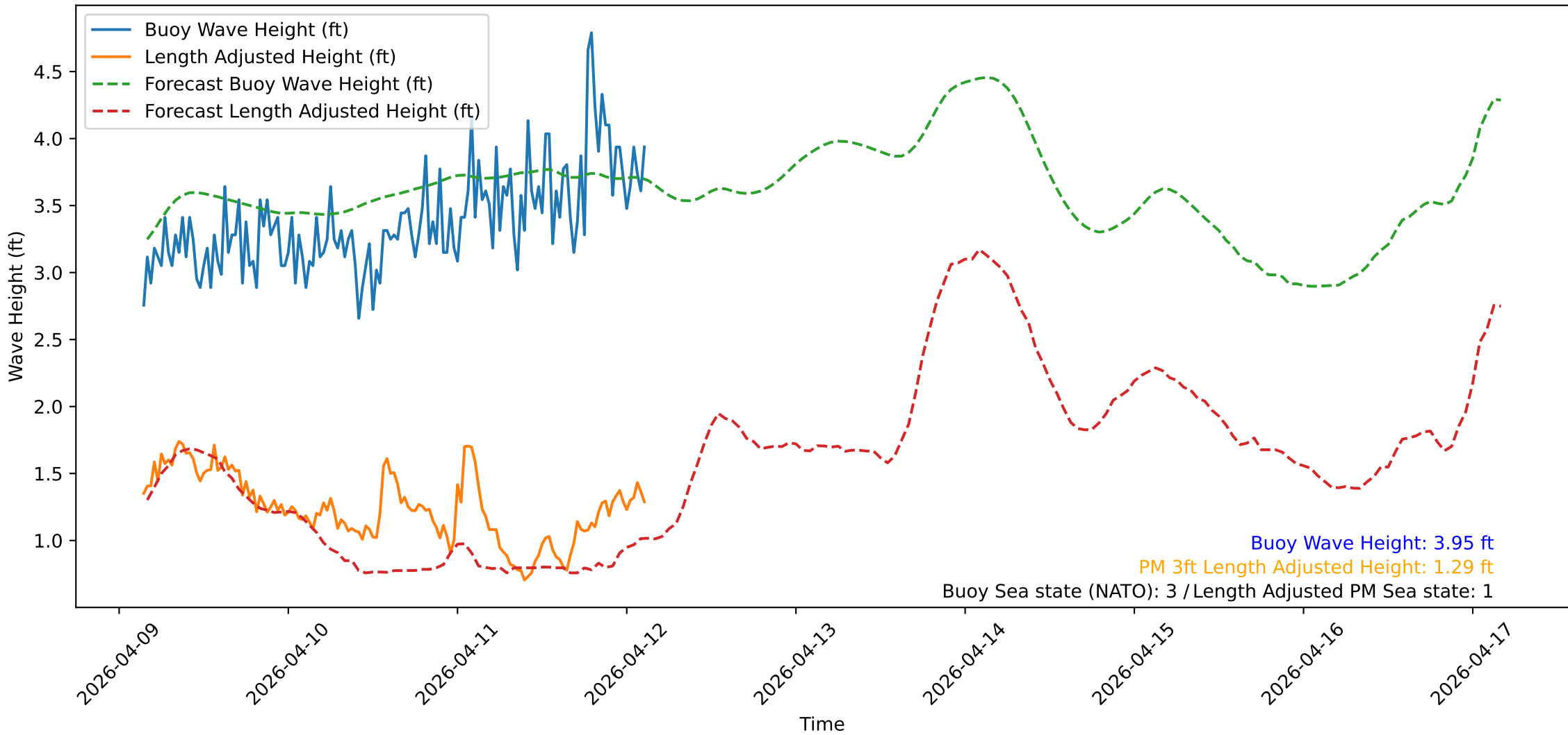
Wave Heights over Time for Oceanside Harbor at 2026-04-12 03:30:32
