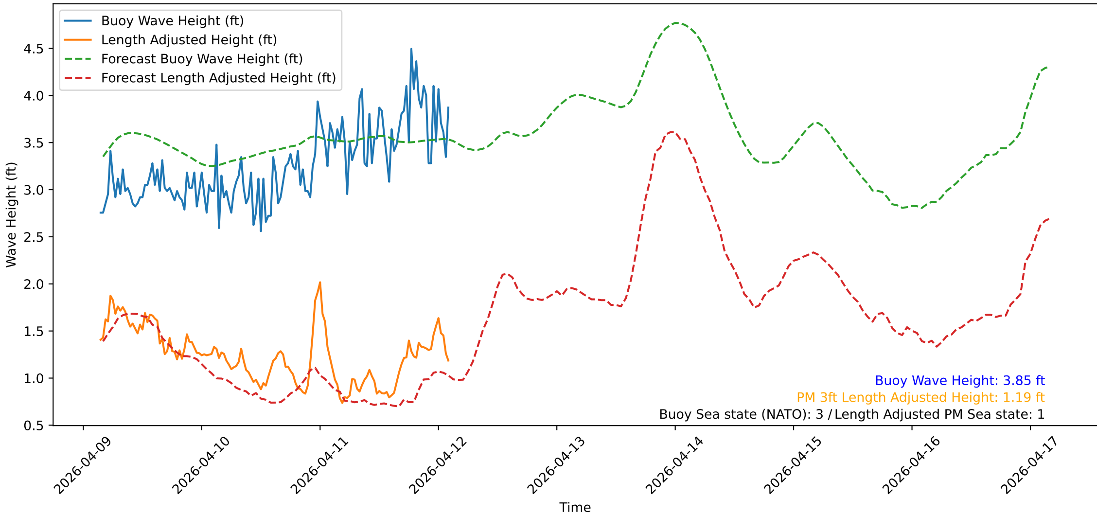
Wave Heights over Time for Green Beach at 2026-04-12 03:31:13
