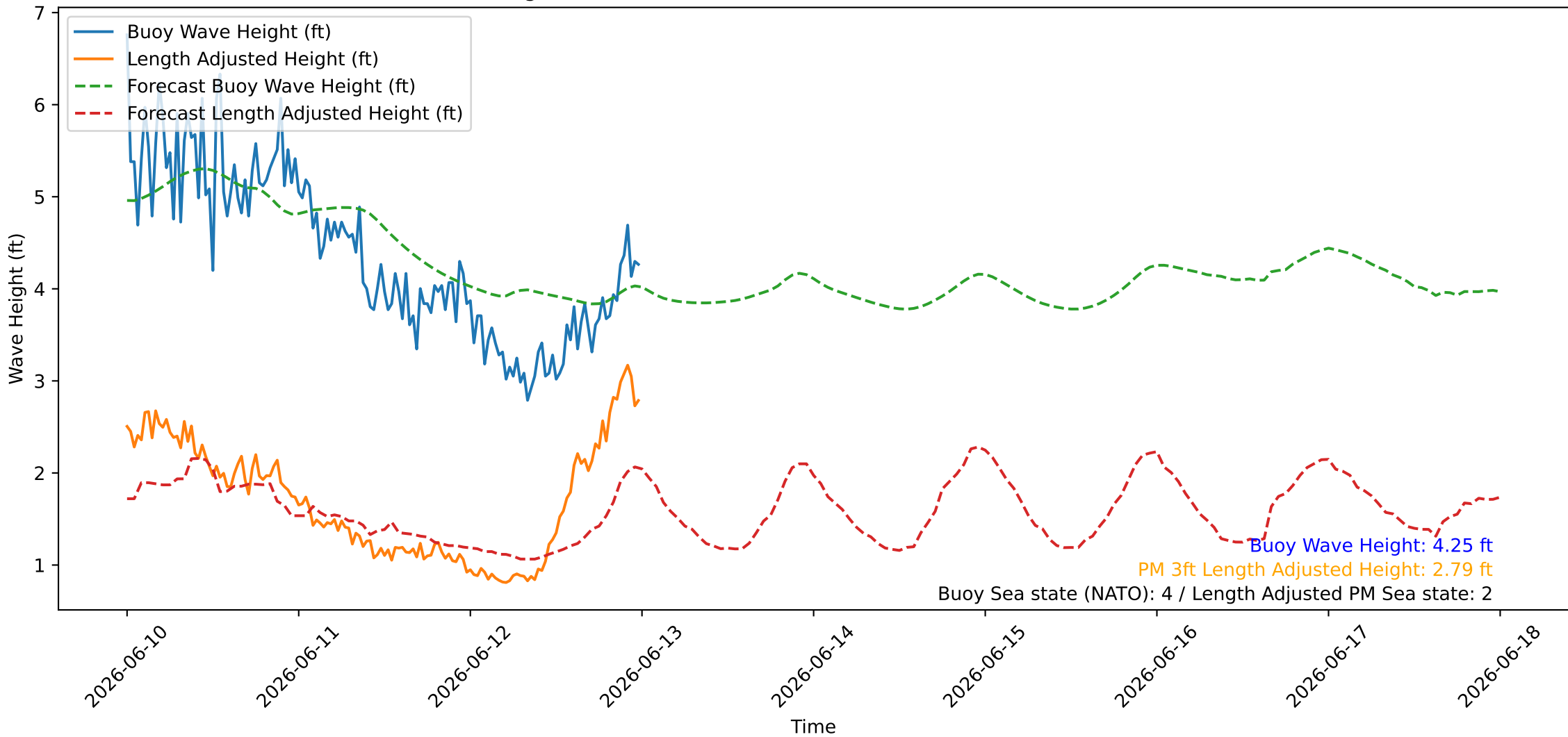
Wave Heights over Time for Oceanside Harbor at 2026-06-13 00:10:26
