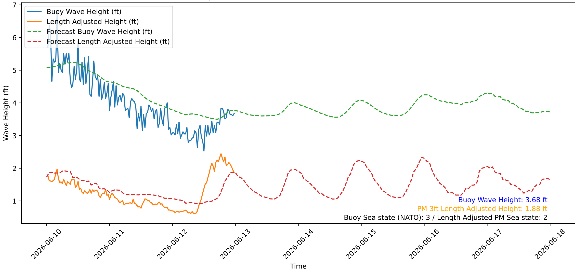
Wave Heights over Time for Red Beach at 2026-06-13 00:10:46
