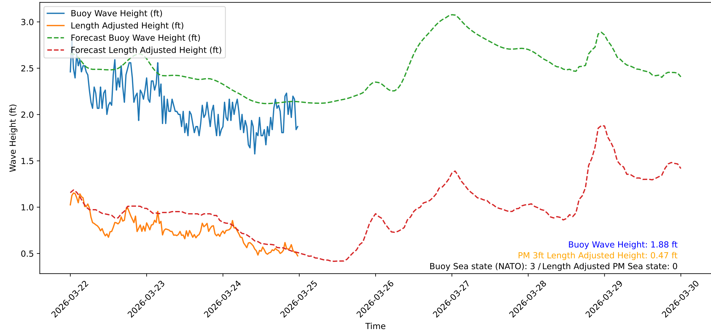
Wave Heights over Time for Oceanside Harbor at 2026-03-25 00:10:31
