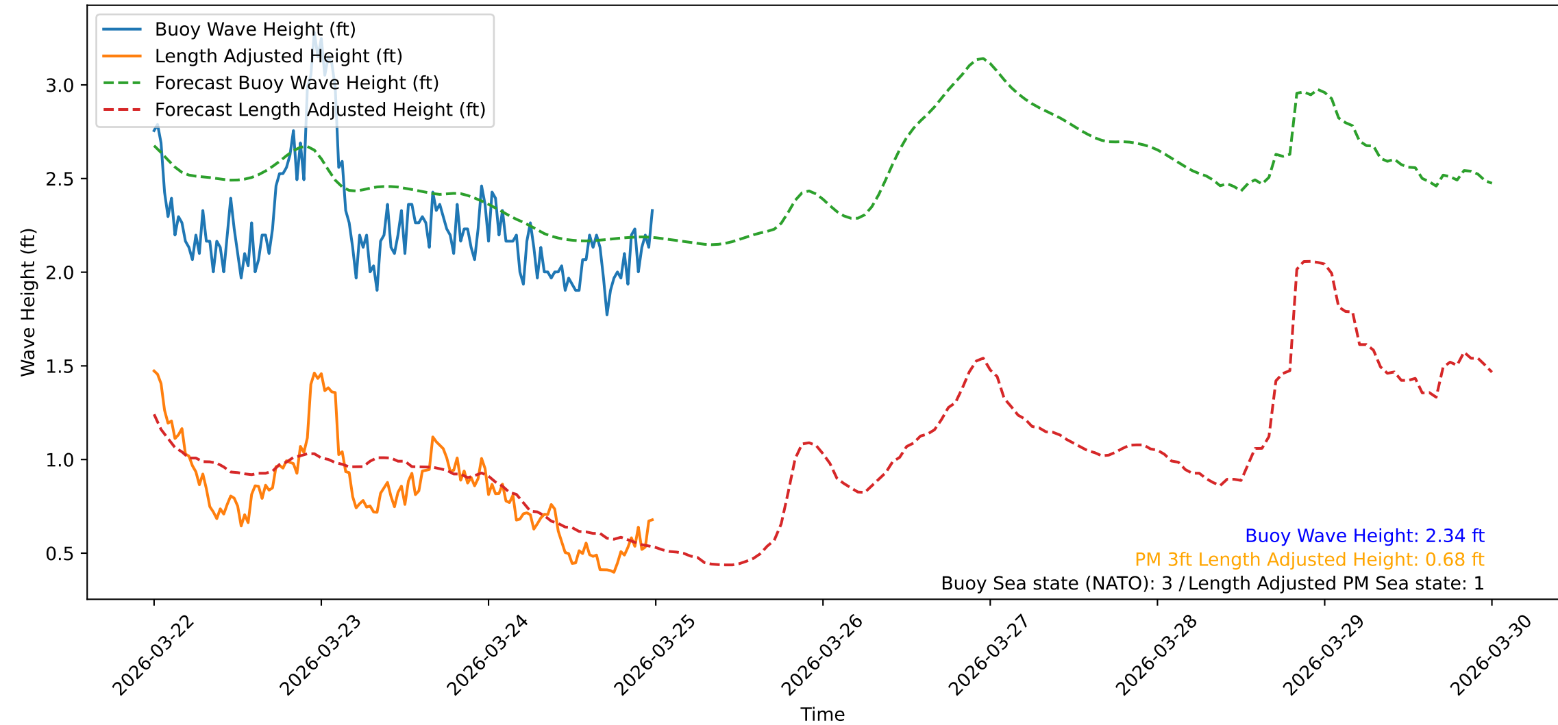
Wave Heights over Time for Green Beach at 2026-03-25 00:11:09
