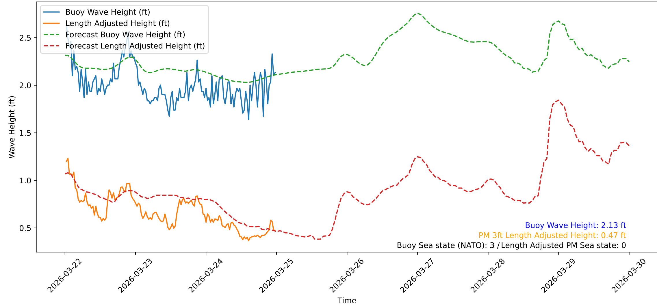
Wave Heights over Time for Red Beach at 2026-03-25 00:10:47
