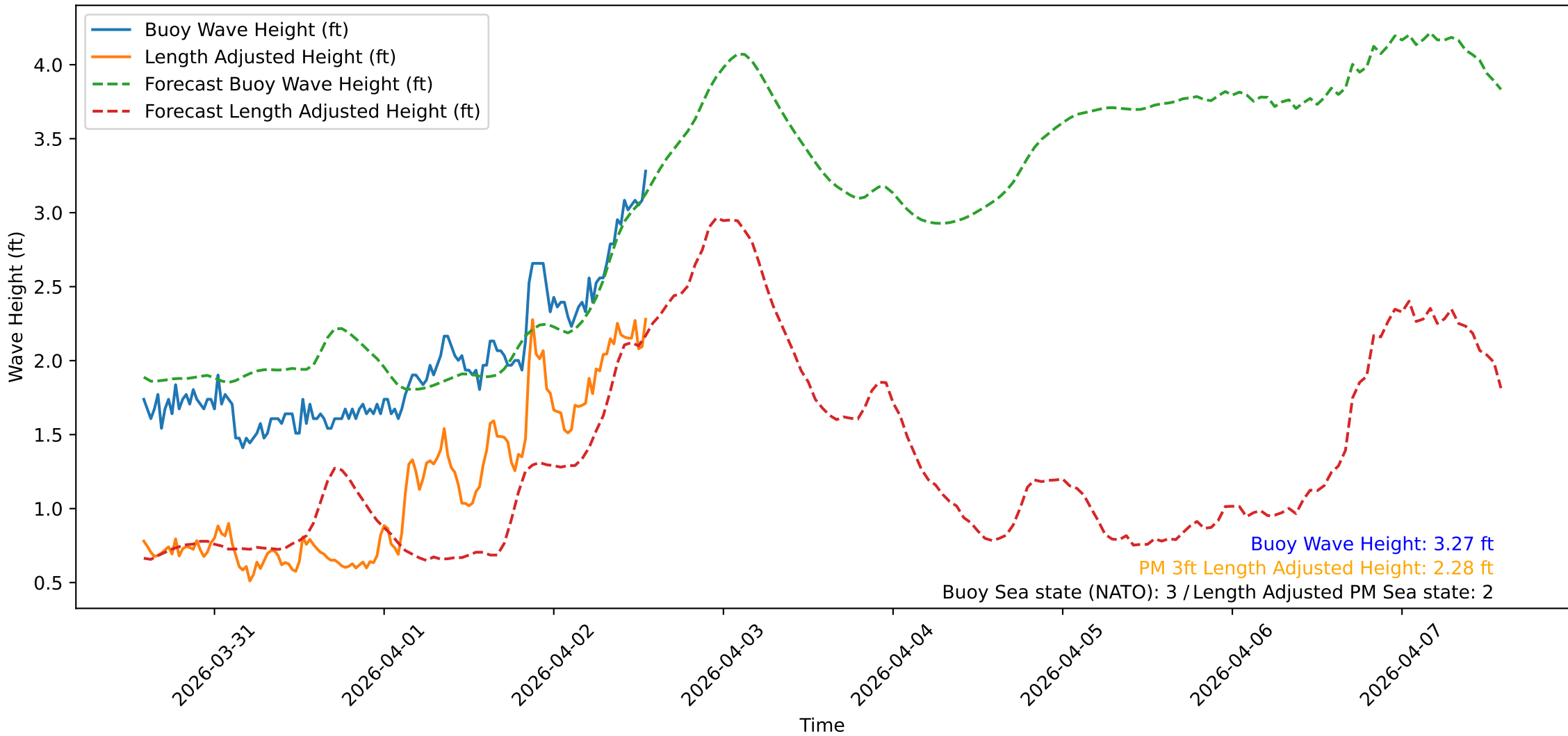
Wave Heights over Time for Green Beach at 2026-04-02 14:01:11
