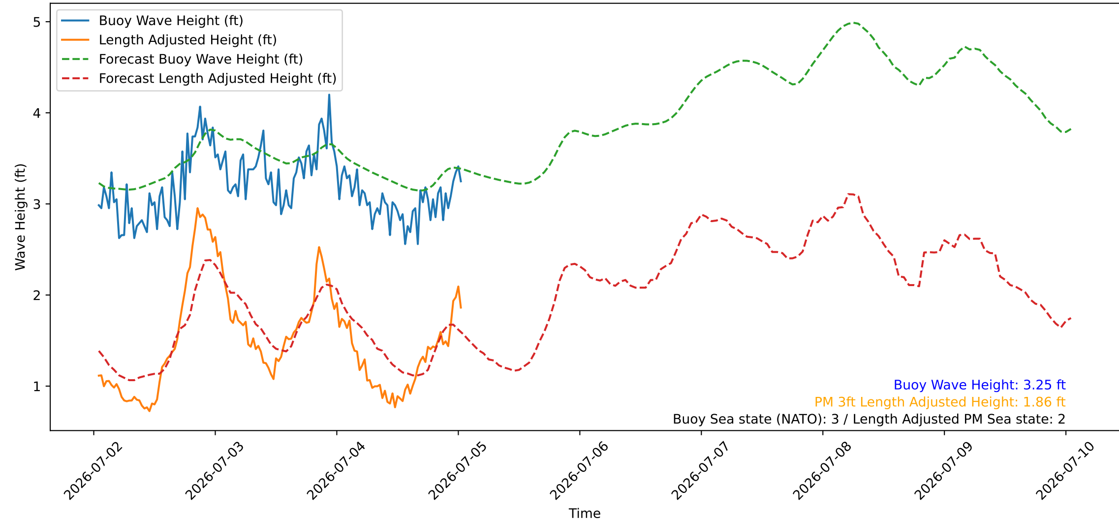
Wave Heights over Time for Green Beach at 2026-07-05 01:11:09
