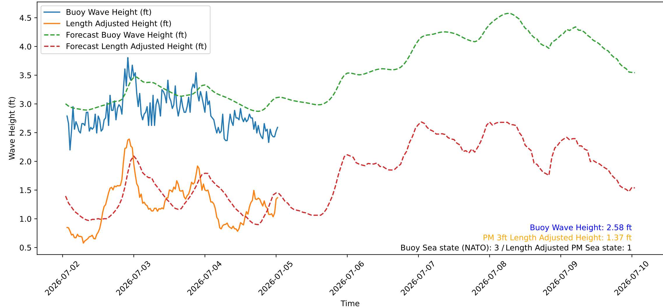
Wave Heights over Time for Red Beach at 2026-07-05 01:10:47
