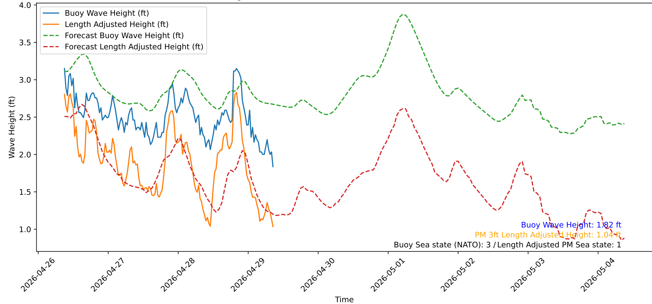
Wave Heights over Time for Green Beach at 2026-04-29 09:11:14
