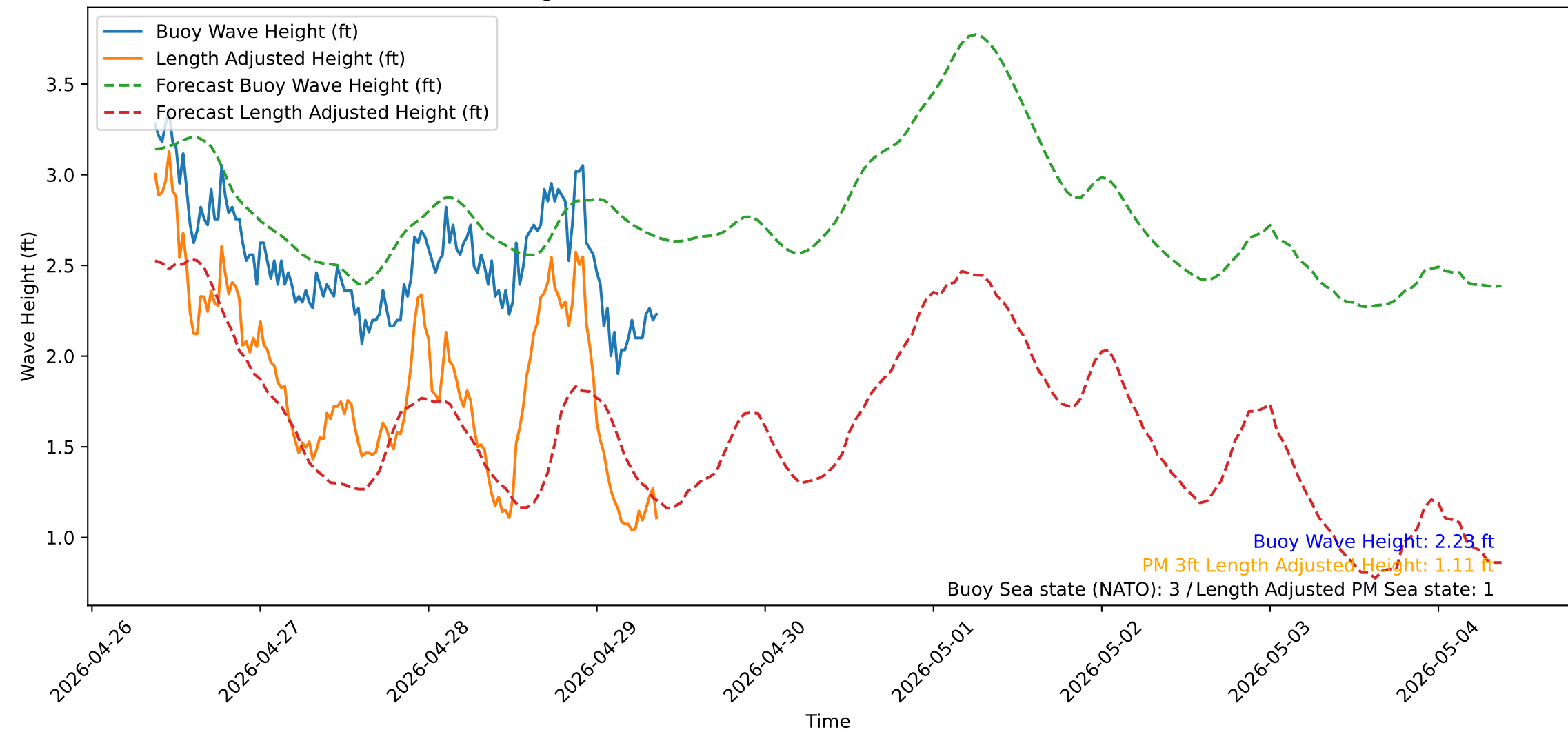
Wave Heights over Time for Oceanside Harbor at 2026-04-29 09:10:32
