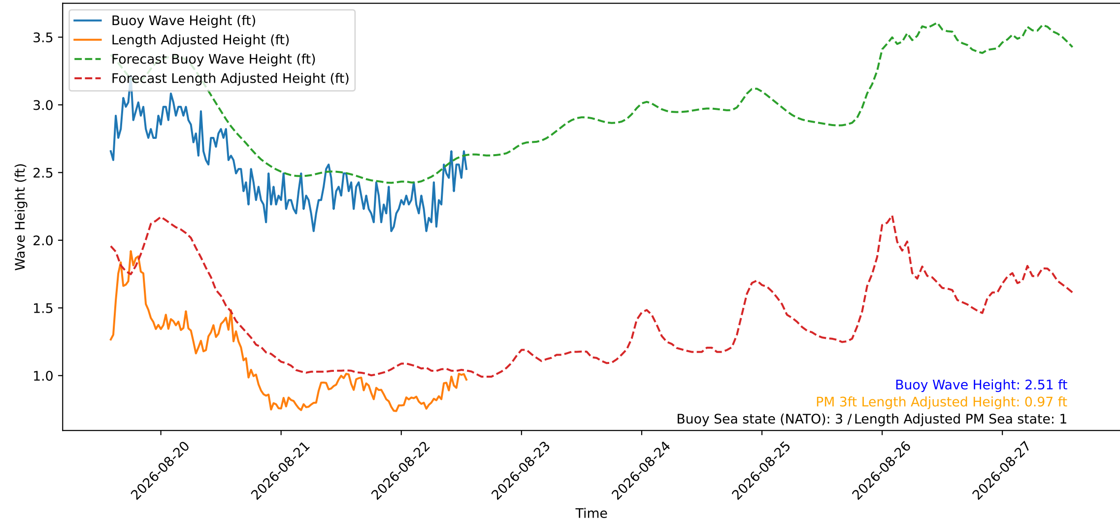
Wave Heights over Time for Red Beach at 2026-08-22 13:40:49
